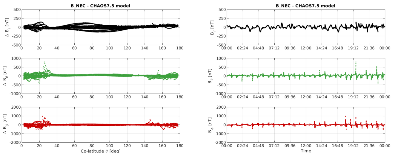
Figure 3-11: S/C B day 19/08: time series of B_{NEC} - B_{Chaos} residuals (right) and B_{NEC} - B_{Chaos} vs colatitude (left).
