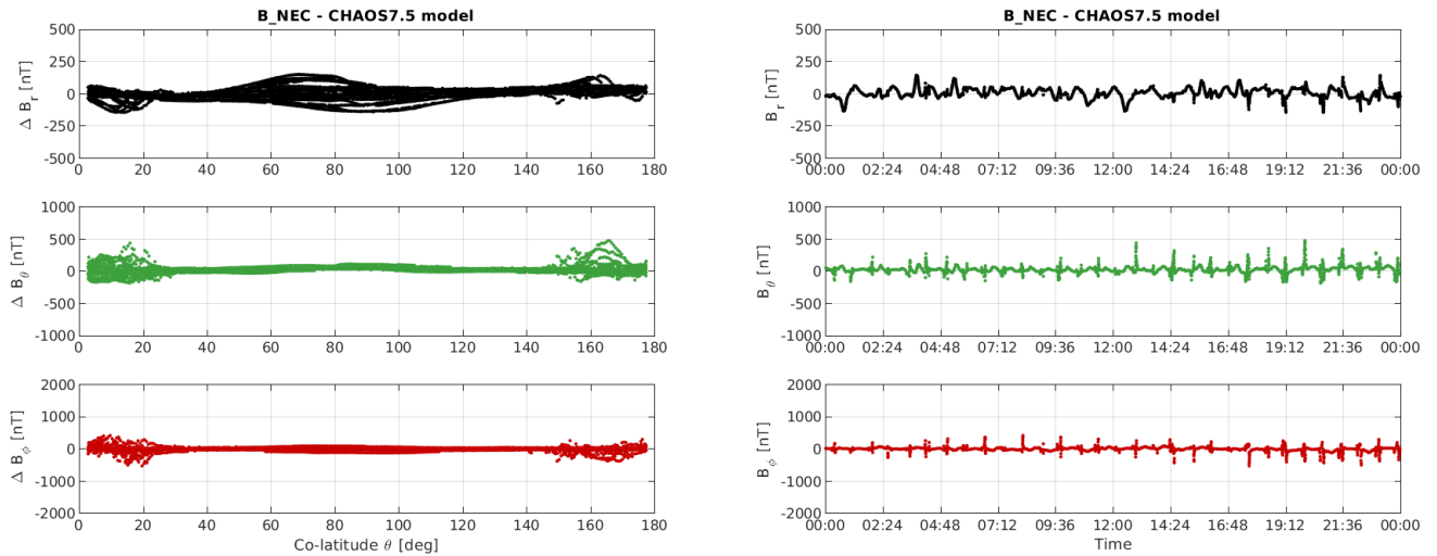
Figure 3-12: S/C C day 19/08: time series of B_{NEC} - B_{Chaos} residuals (right) and B_{NEC} - B_{Chaos} vs colatitude (left)
