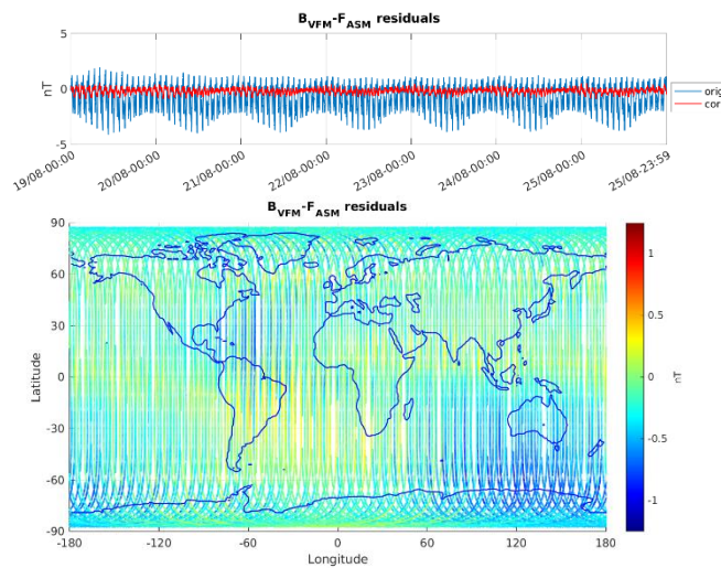
Figure 3-5: ASM-VFM residuals for S/C A, during monitoring period 19/08-25/08. In top figure are plotted: difference between |B_{VFM}| and F_{ASM} (without dB_{Sun} correction) (blue colour), and the residuals with dB_{Sun} corrections (red colour). In bottom figure residuals are presented on the world map.
