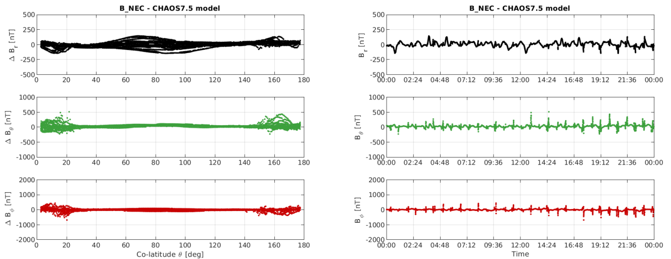
Figure 3-10: S/C A day 19/08: time series of B_{NEC} - B_{Chaos} residuals (right) and B_{NEC} - B_{Chaos} vs colatitude (left).
