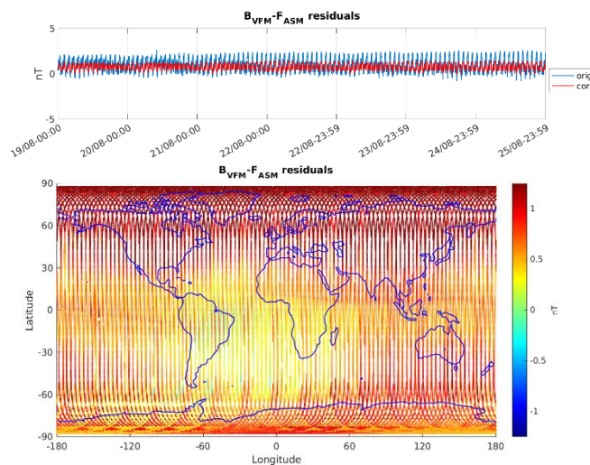
Figure 3-6: ASM-VFM residuals for S/C B, during monitoring period 19/08-25/08. In top figure are plotted: difference between |B_{VFM}| and F_{ASM} (without dB_{Sun} correction) (blue colour), and the residuals with dB_{Sun} corrections (red colour). In bottom figure residuals are presented on the world map.
