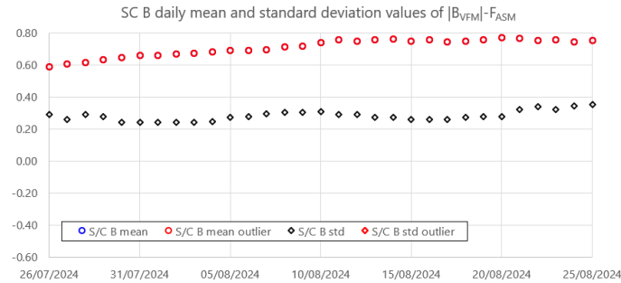
Figure 3-4: Daily mean and standard deviation values of ASM-VFM residuals (defined as dF = |B_{VFM}| - F_{ASM} ) for S/C B.
