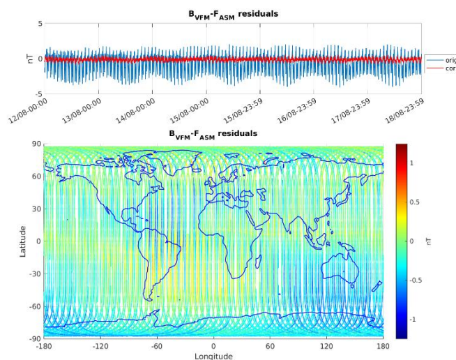
Figure 3-5: ASM-VFM residuals for S/C A, during monitoring period 12/08-18/08. In top figure are plotted: difference between |B_{VFM}| and F_{ASM} (without dB_{Sun} correction) (blue colour), and the residuals with dB_{Sun} corrections (red colour). In bottom figure residuals are presented on the world map.
