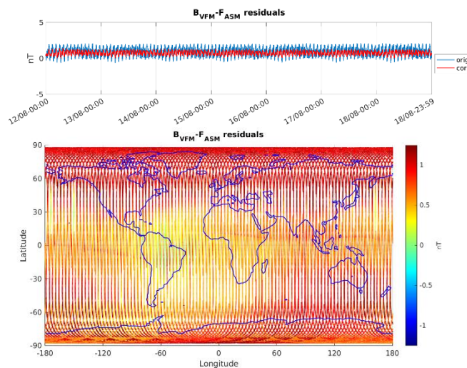
Figure 3-6: ASM-VFM residuals for S/C B, during monitoring period 12/08-18/08. In top figure are plotted: difference between |B_{VFM}| and F_{ASM} (without dB_{Sun} correction) (blue colour), and the residuals with dB_{Sun} corrections (red colour). In bottom figure residuals are presented on the world map.
