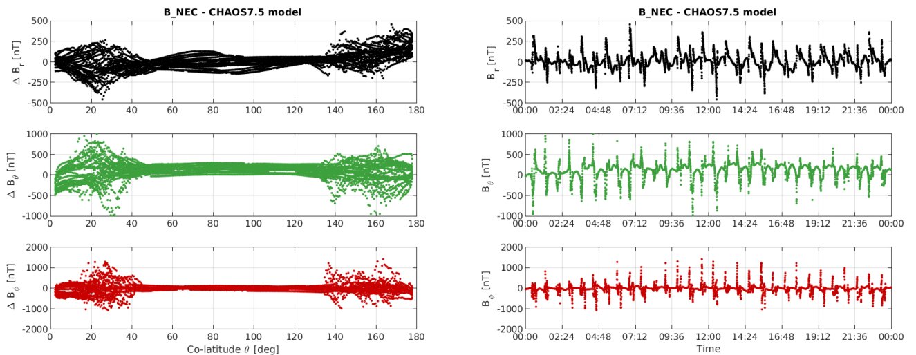
Figure 3-11: S/C B day 12/08: time series of B_{NEC} - B_{Chaos} residuals (right) and B_{NEC} - B_{Chaos} vs colatitude (left).
