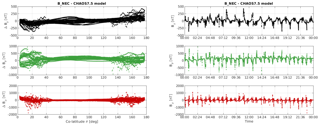
Figure 3-12: S/C C day 12/08: time series of B_{NEC} - B_{Chaos} residuals (right) and B_{NEC} - B_{Chaos} vs colatitude (left)
