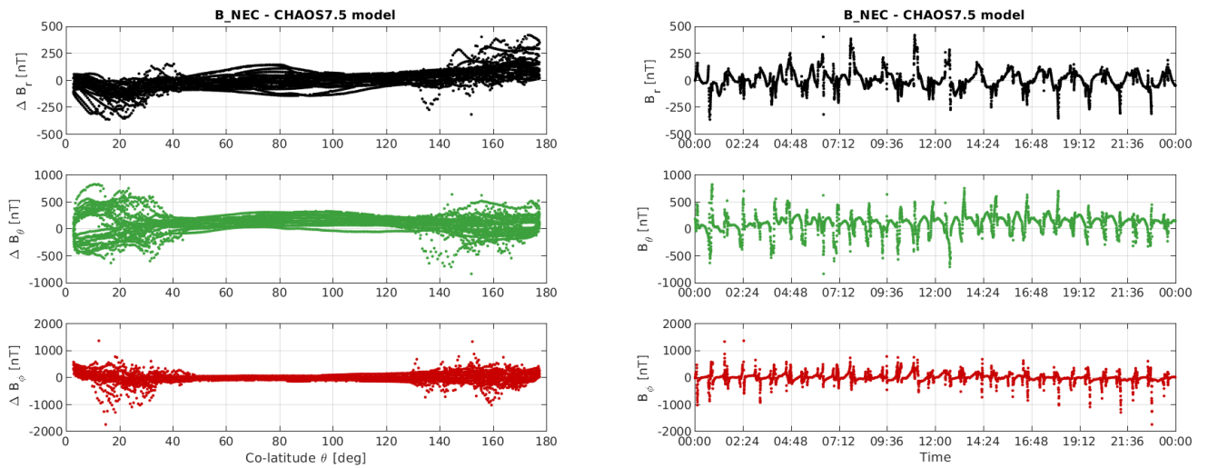
Figure 3-10: S/C A day 12/08: time series of B_{NEC} - B_{Chaos} residuals (right) and B_{NEC} - B_{Chaos} vs colatitude (left).
