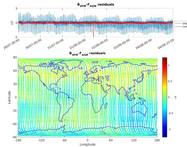
Figure 3-5: ASM-VFM residuals for S/C A, during monitoring period 29/07-04/08. In top figure are plotted: difference between |B_{VFM}| and F_{ASM} (without dB_{Sun} correction) (blue colour), and the residuals with dB_{Sun} corrections (red colour). In bottom figure residuals are presented on the world map.
