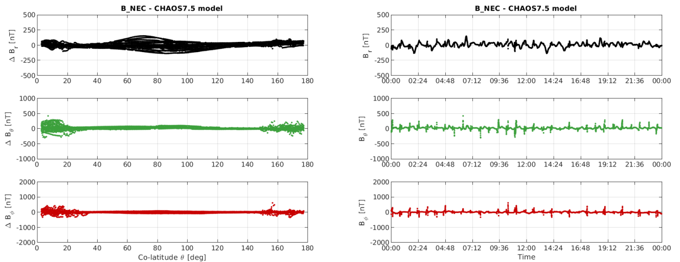
Figure 3-10: S/C A day 29/07: time series of B_{NEC} - B_{Chaos} residuals (right) and B_{NEC} - B_{Chaos} vs colatitude (left).
