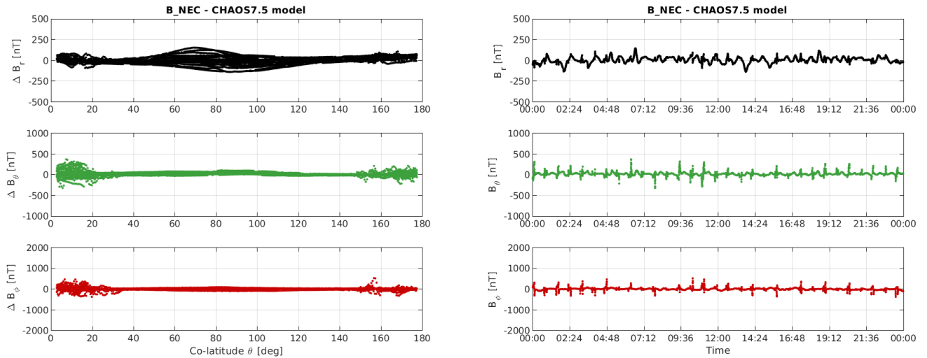
Figure 3-12: S/C C day 29/07: time series of B_{NEC} - B_{Chaos} residuals (right) and B_{NEC} - B_{Chaos} vs colatitude (left)
