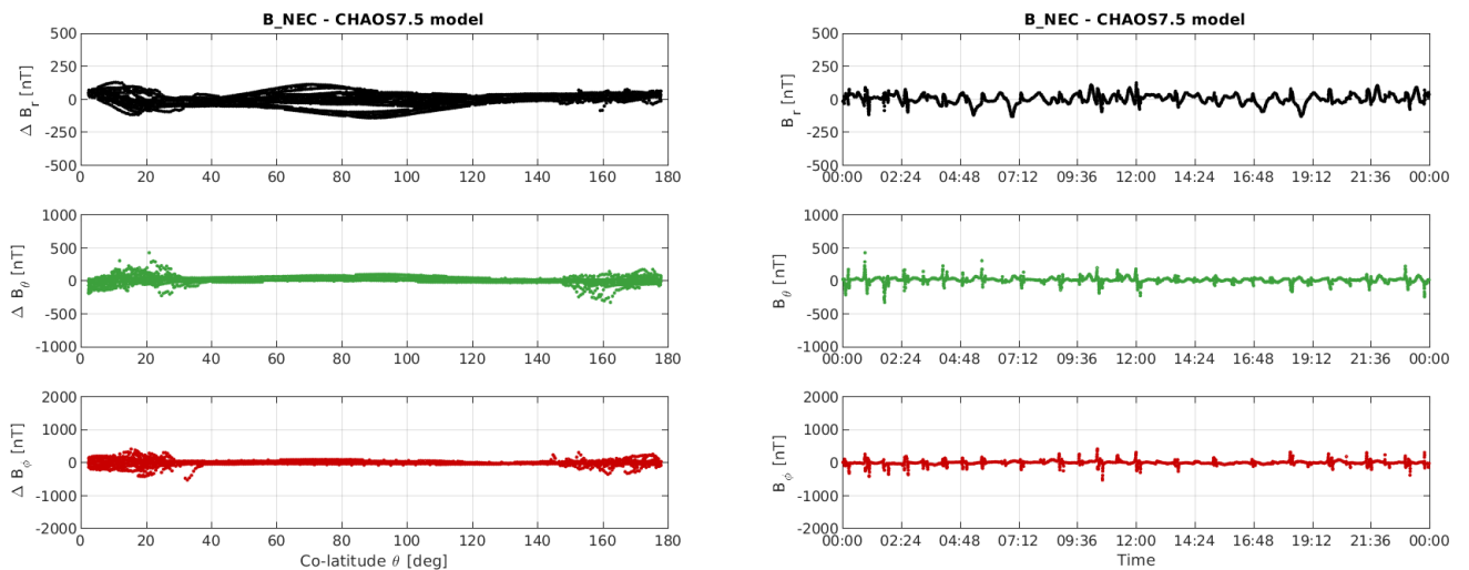
Figure 3-11: S/C B day 29/07: time series of B_{NEC} - B_{Chaos} residuals (right) and B_{NEC} - B_{Chaos} vs colatitude (left).
