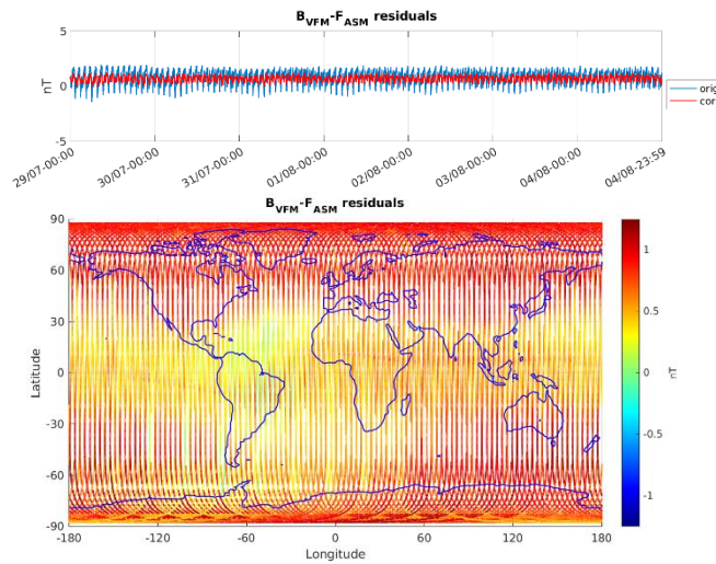
Figure 3-6: ASM-VFM residuals for S/C B, during monitoring period 29/07-04/08. In top figure are plotted: difference between |B_{VFM}| and F_{ASM} (without dB_{Sun} correction) (blue colour), and the residuals with dB_{Sun} corrections (red colour). In bottom figure residuals are presented on the world map.
