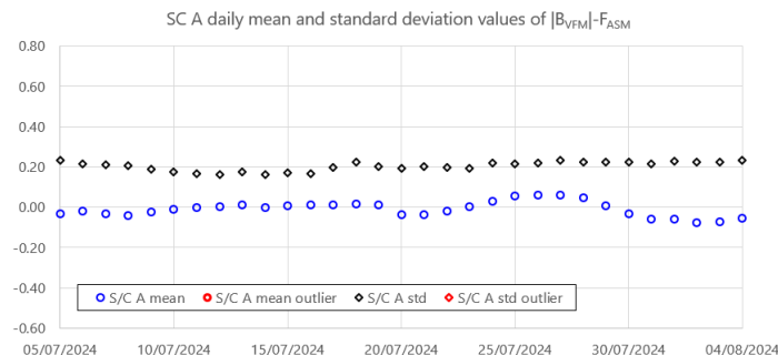
Figure 3-3: Daily mean and standard deviation values of ASM-VFM residuals (defined as dF = |B_{VFM}| - F_{ASM} ) for S/C A.
