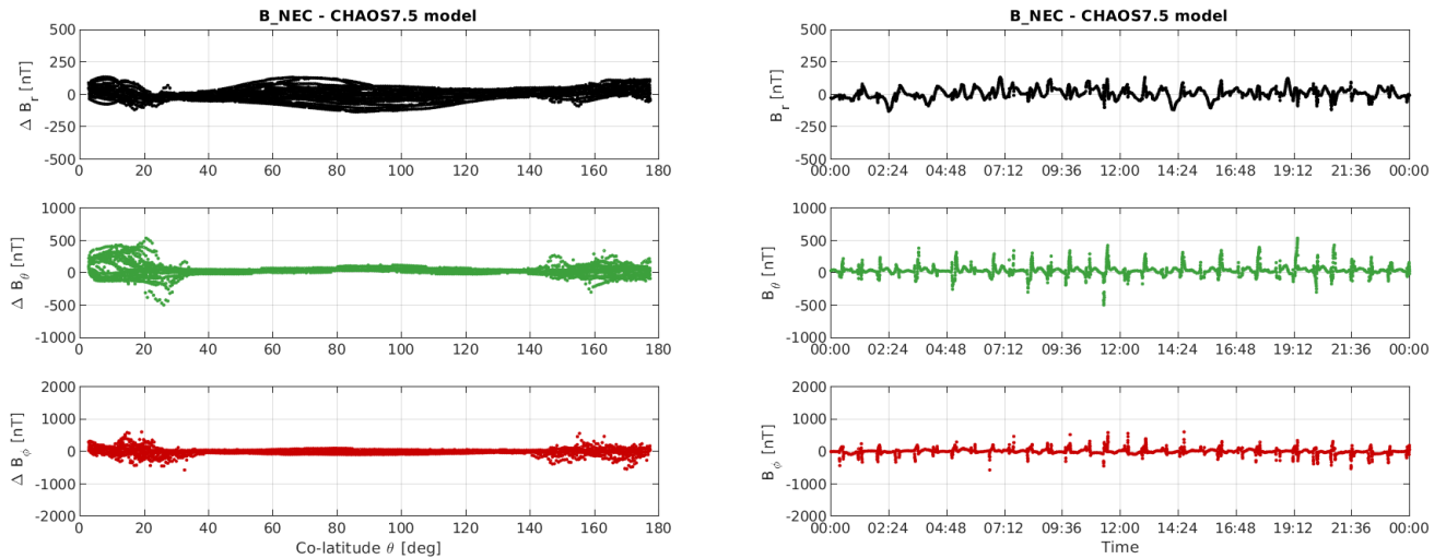
Figure 3-12: S/C C day 22/07: time series of B_{NEC} - B_{Chaos} residuals (right) and B_{NEC} - B_{Chaos} vs colatitude (left)
