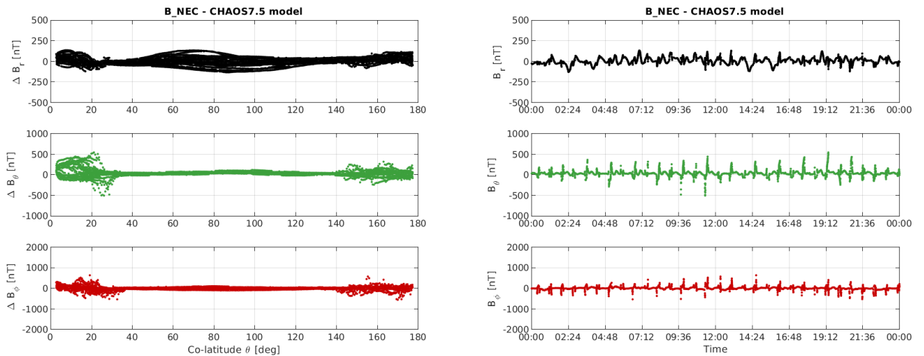
Figure 3-10: S/C A day 22/07: time series of B_{NEC} - B_{Chaos} residuals (right) and B_{NEC} - B_{Chaos} vs colatitude (left).
