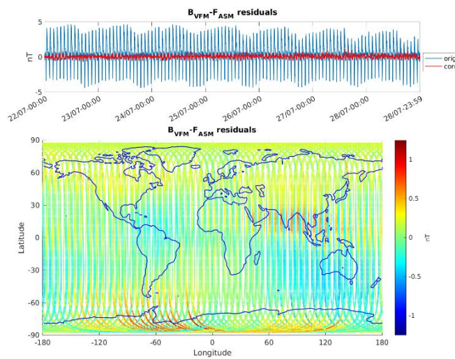
Figure 3-5: ASM-VFM residuals for S/C A, during monitoring period 22/07-28/07. In top figure are plotted: difference between |B_{VFM}| and F_{ASM} (without dB_{Sun} correction) (blue colour), and the residuals with dB_{Sun} corrections (red colour). In bottom figure residuals are presented on the world map.
