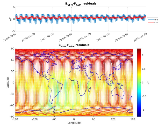
Figure 3-6: ASM-VFM residuals for S/C B, during monitoring period 22/07-28/07. In top figure are plotted: difference between |B_{VFM}| and F_{ASM} (without dB_{Sun} correction) (blue colour), and the residuals with dB_{Sun} corrections (red colour). In bottom figure residuals are presented on the world map.
