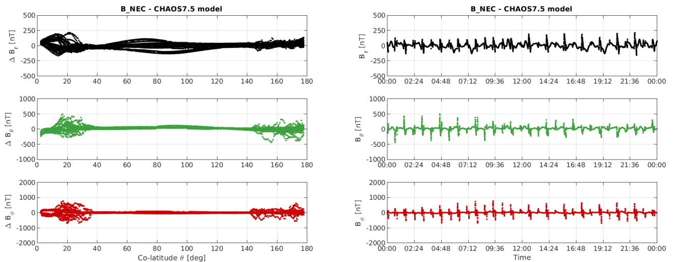
Figure 3-11: S/C B day 22/07: time series of B_{NEC} - B_{Chaos} residuals (right) and B_{NEC} - B_{Chaos} vs colatitude (left).
