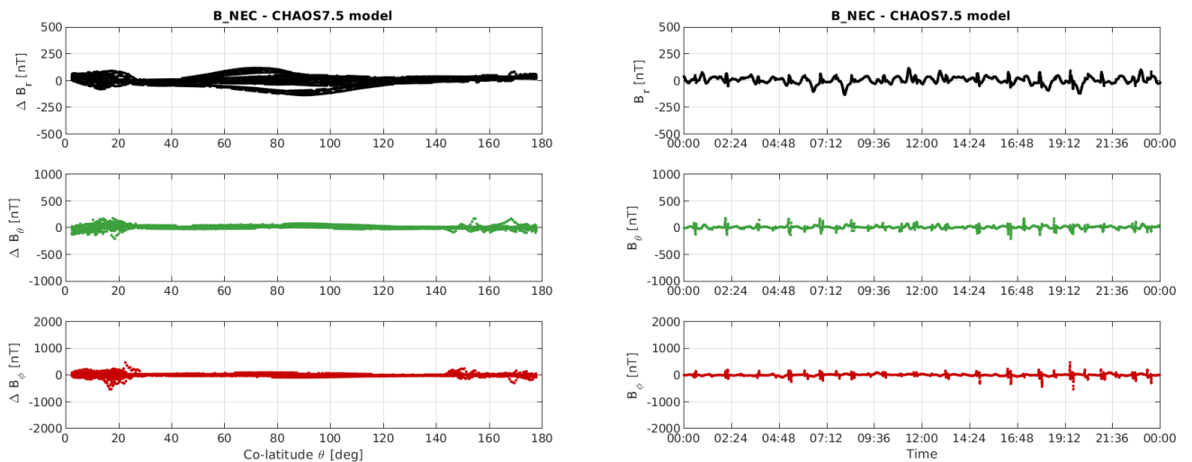
Figure 3-11: S/C B day 15/07: time series of B_{NEC} - B_{Chaos} residuals (right) and B_{NEC} - B_{Chaos} vs colatitude (left).
