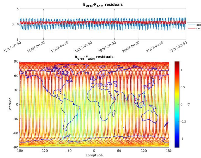
Figure 3-6: ASM-VFM residuals for S/C B, during monitoring period 15/07-21/07. In top figure are plotted: difference between |B_{VFM}| and F_{ASM} (without dB_{Sun} correction) (blue colour), and the residuals with dB_{Sun} corrections (red colour). In bottom figure residuals are presented on the world map.
