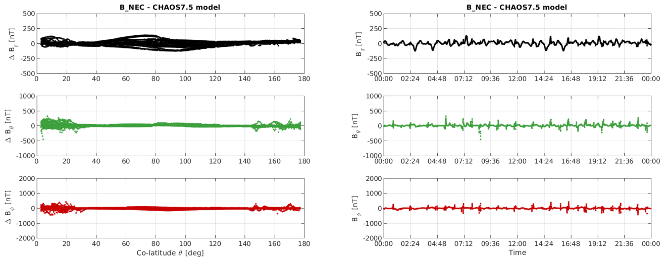
Figure 3-12: S/C C day 15/07: time series of B_{NEC} - B_{Chaos} residuals (right) and B_{NEC} - B_{Chaos} vs colatitude (left)
