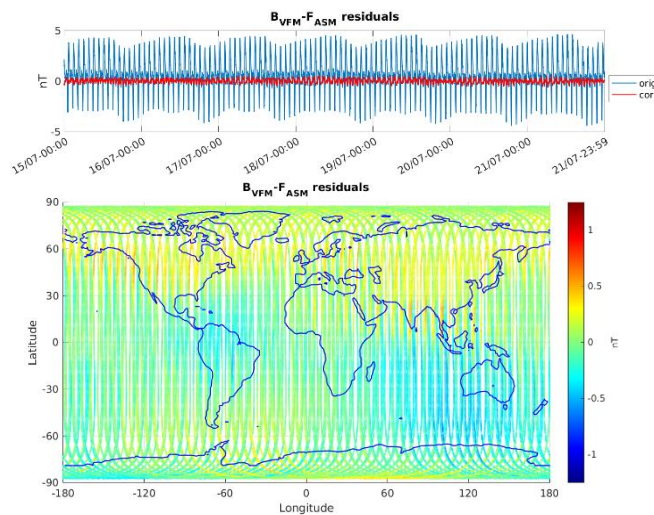
Figure 3-5: ASM-VFM residuals for S/C A, during monitoring period 15/07-21/07. In top figure are plotted: difference between |B_{VFM}| and F_{ASM} (without dB_{Sun} correction) (blue colour), and the residuals with dB_{Sun} corrections (red colour). In bottom figure residuals are presented on the world map.
