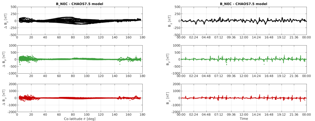
Figure 3-10: S/C A day 15/07: time series of B_{NEC} - B_{Chaos} residuals (right) and B_{NEC} - B_{Chaos} vs colatitude (left).
