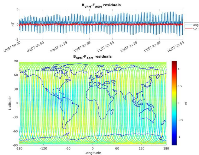
Figure 3-5: ASM-VFM residuals for S/C A, during monitoring period 08/07-14/07. In top figure are plotted: difference between |B_{VFM}| and F_{ASM} (without dB_{Sun} correction) (blue colour), and the residuals with dB_{Sun} corrections (red colour). In bottom figure residuals are presented on the world map.
