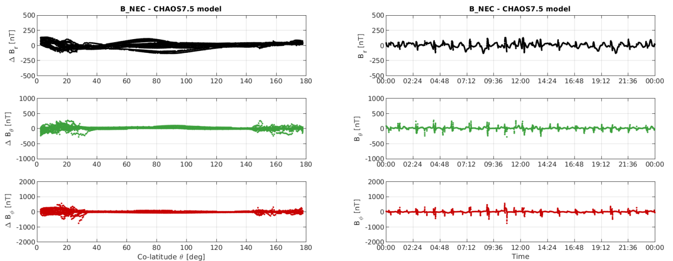
Figure 3-11: S/C B day 08/07: time series of B_{NEC} - B_{Chaos} residuals (right) and B_{NEC} - B_{Chaos} vs colatitude (left).
