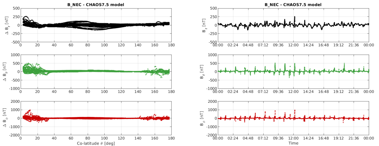
Figure 3-10: S/C A day 08/07: time series of B_{NEC} - B_{Chaos} residuals (right) and B_{NEC} - B_{Chaos} vs colatitude (left).
