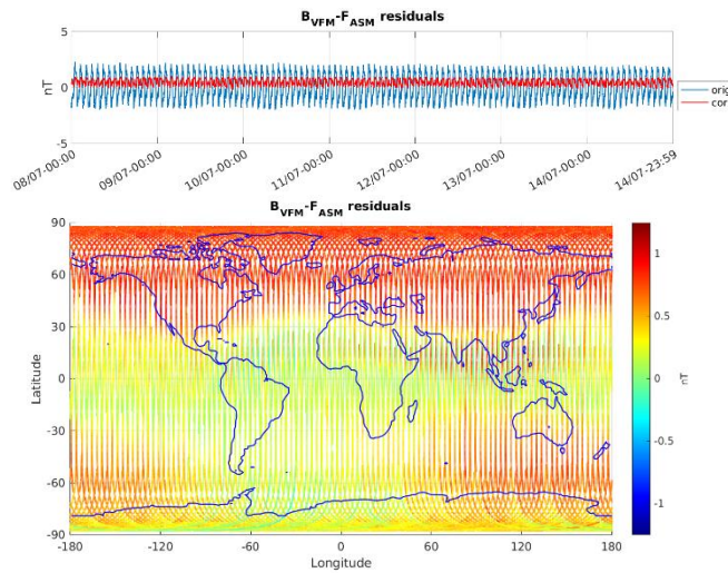
Figure 3-6: ASM-VFM residuals for S/C B, during monitoring period 08/07-14/07. In top figure are plotted: difference between |B_{VFM}| and F_{ASM} (without dB_{Sun} correction) (blue colour), and the residuals with dB_{Sun} corrections (red colour). In bottom figure residuals are presented on the world map.
