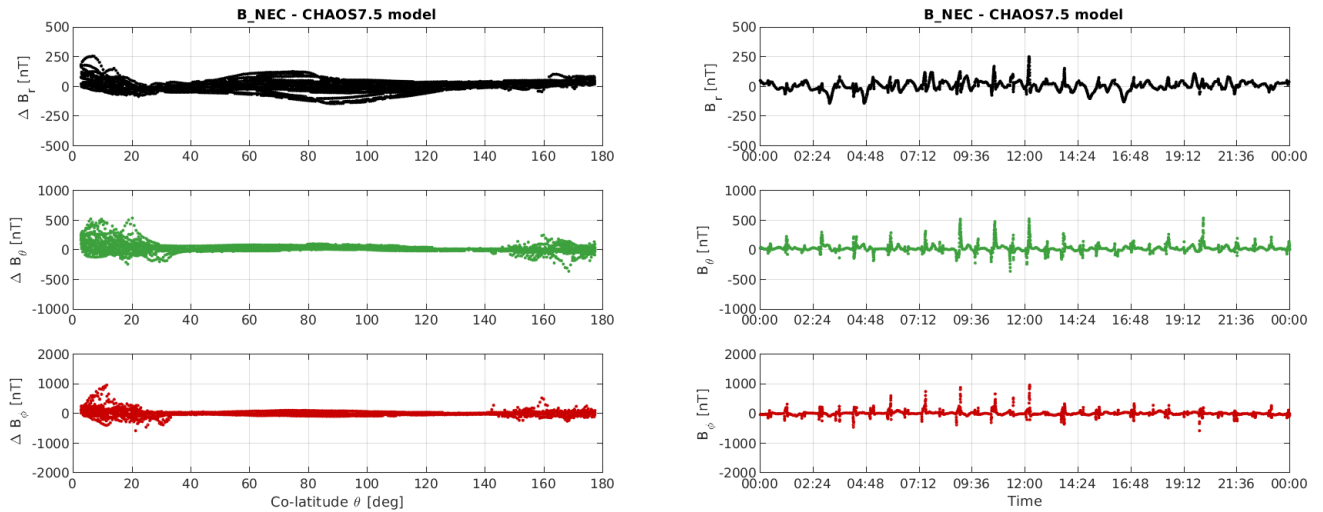
Figure 3-12: S/C C day 08/07: time series of B_{NEC} - B_{Chaos} residuals (right) and B_{NEC} - B_{Chaos} vs colatitude (left)
