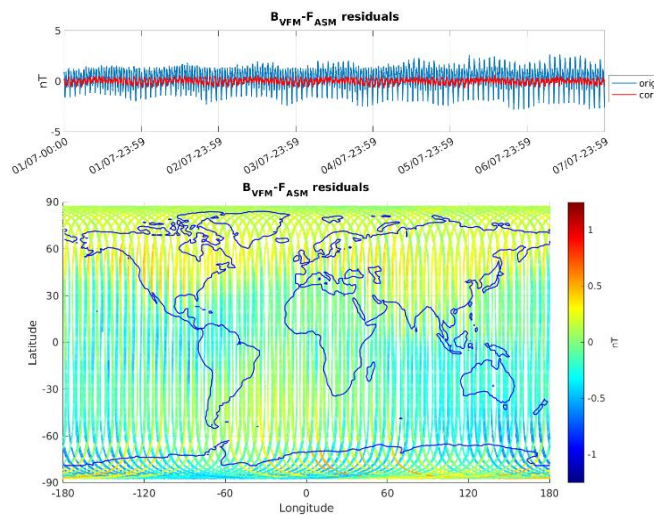
Figure 3-5: ASM-VFM residuals for S/C A, during monitoring period 01/07-07/07. In top figure are plotted: difference between |B_{VFM}| and F_{ASM} (without dB_{Sun} correction) (blue colour), and the residuals with dB_{Sun} corrections (red colour). In bottom figure residuals are presented on the world map.
