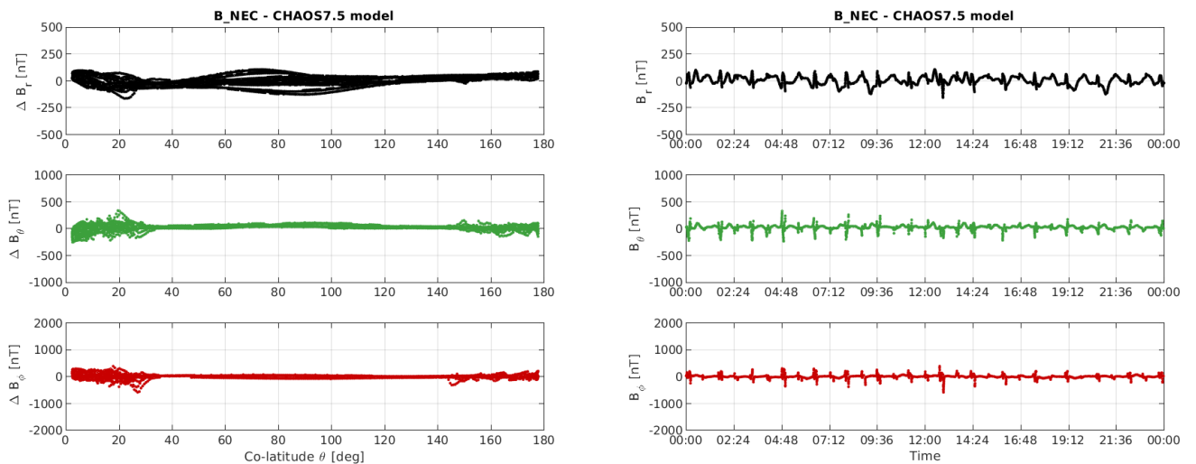
Figure 3-11: S/C B day 01/07: time series of B_{NEC} - B_{Chaos} residuals (right) and B_{NEC} - B_{Chaos} vs colatitude (left).
