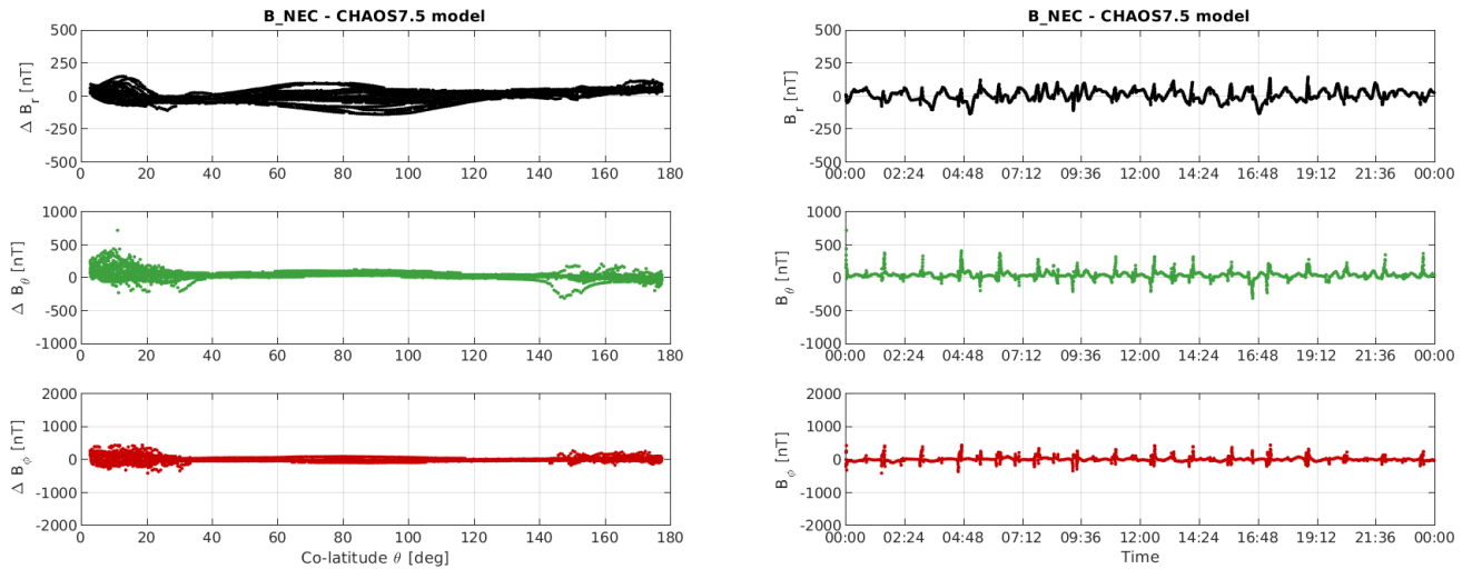
Figure 3-12: S/C C day 01/07: time series of B_{NEC} - B_{Chaos} residuals (right) and B_{NEC} - B_{Chaos} vs colatitude (left)
