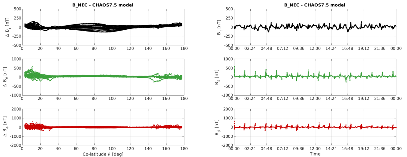
Figure 3-10: S/C A day 01/07: time series of B_{NEC} - B_{Chaos} residuals (right) and B_{NEC} - B_{Chaos} vs colatitude (left).
