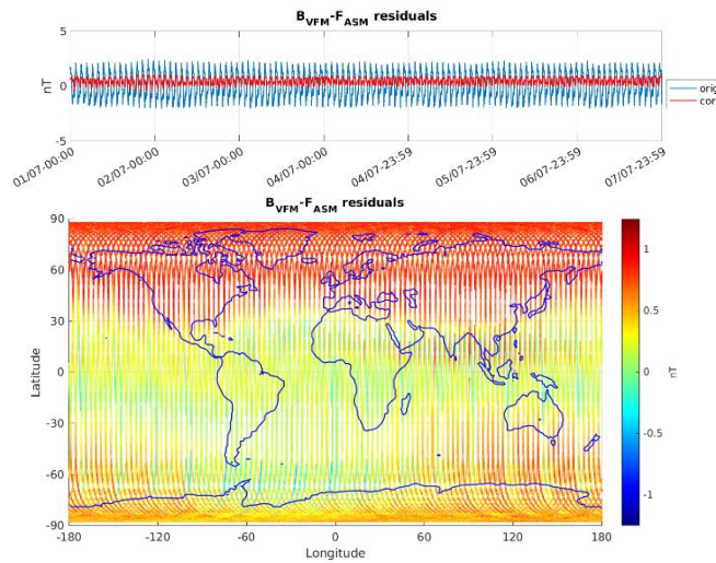
Figure 3-6: ASM-VFM residuals for S/C B, during monitoring period 01/07-07/07. In top figure are plotted: difference between |B_{VFM}| and F_{ASM} (without dB_{Sun} correction) (blue colour), and the residuals with dB_{Sun} corrections (red colour). In bottom figure residuals are presented on the world map.
