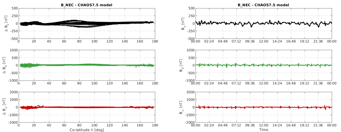
Figure 3-11: S/C B day 24/06: time series of B_{NEC} - B_{Chaos} residuals (right) and B_{NEC} - B_{Chaos} vs colatitude (left).
