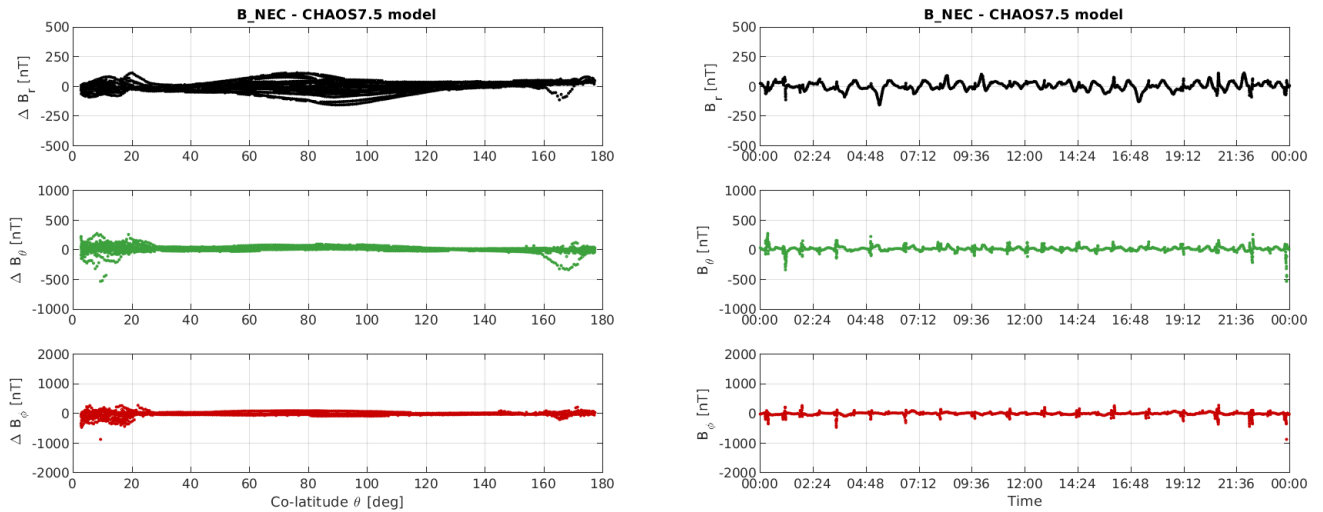
Figure 3-12: S/C C day 24/06: time series of B_{NEC} - B_{Chaos} residuals (right) and B_{NEC} - B_{Chaos} vs colatitude (left)
