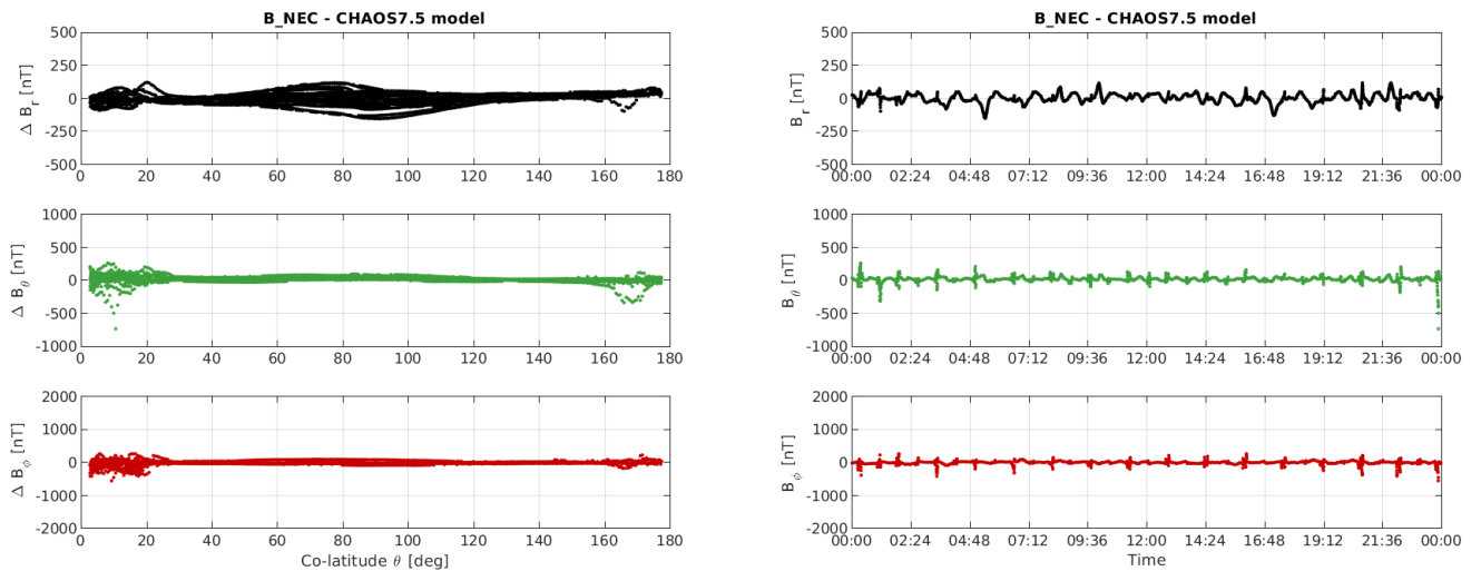
Figure 3-10: S/C A day 24/06: time series of B_{NEC} - B_{Chaos} residuals (right) and B_{NEC} - B_{Chaos} vs colatitude (left).
