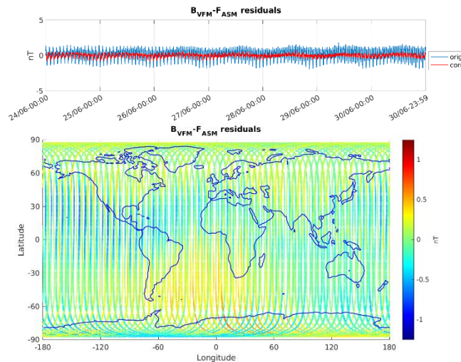
Figure 3-5: ASM-VFM residuals for S/C A, during monitoring period 24/06-30/06. In top figure are plotted: difference between |B_{VFM}| and F_{ASM} (without dB_{Sun} correction) (blue colour), and the residuals with dB_{Sun} corrections (red colour). In bottom figure residuals are presented on the world map.
