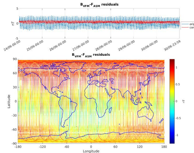
Figure 3-6: ASM-VFM residuals for S/C B, during monitoring period 24/06-30/06. In top figure are plotted: difference between |B_{VFM}| and F_{ASM} (without dB_Sun correction) (blue colour), and the residuals with dB_Sun corrections (red colour). In bottom figure residuals are presented on the world map.
