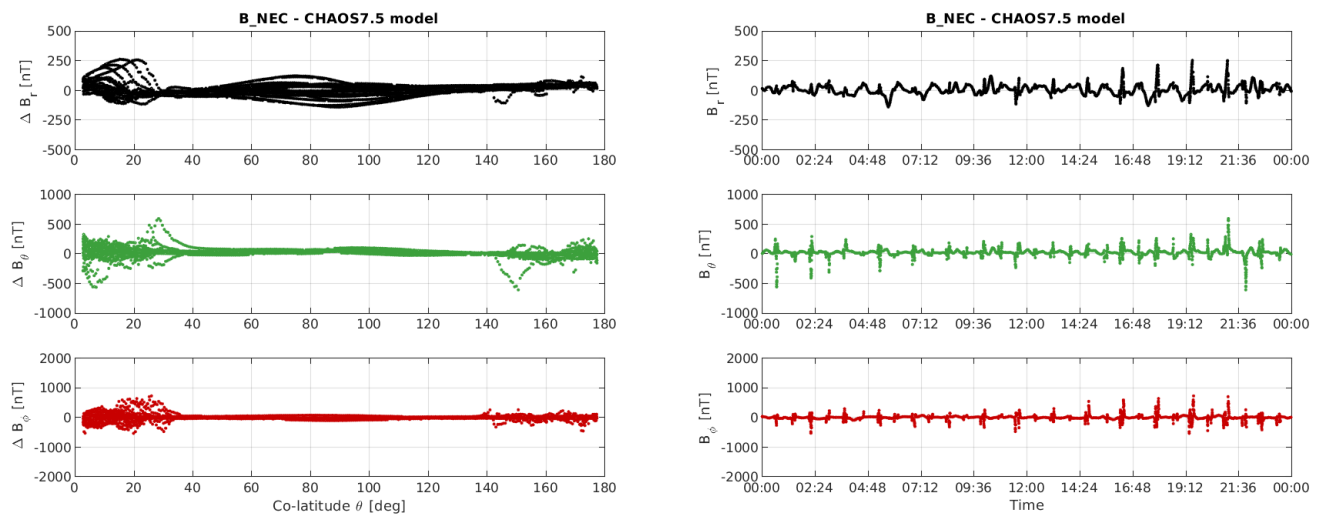
Figure 3-12: S/C C day 17/06: time series of B_{NEC} - B_{Chaos} residuals (right) and B_{NEC} - B_{Chaos} vs colatitude (left)
