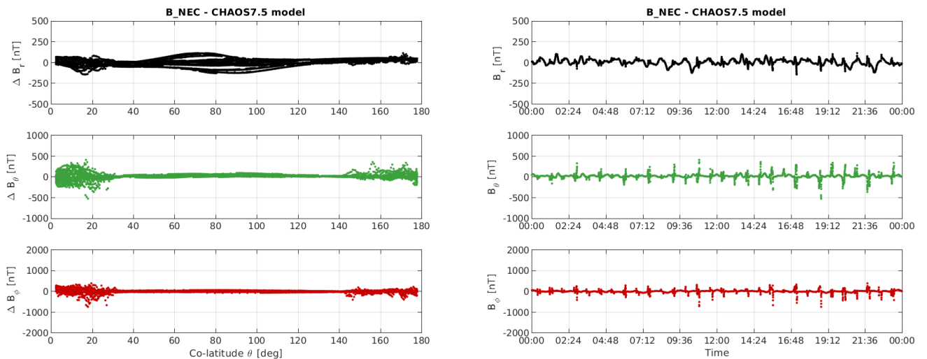
Figure 3-11: S/C B day 17/06: time series of B_{NEC} - B_{Chaos} residuals (right) and B_{NEC} - B_{Chaos} vs colatitude (left).
