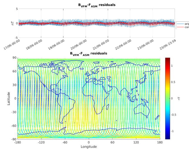
Figure 3-5: ASM-VFM residuals for S/C A, during monitoring period 17/06-23/06. In top figure are plotted: difference between |B_{VFM}| and F_{ASM} (without dB_{Sun} correction) (blue colour), and the residuals with dB_{Sun} corrections (red colour). In bottom figure residuals are presented on the world map.
