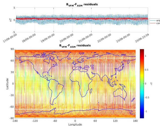
Figure 3-6: ASM-VFM residuals for S/C B, during monitoring period 17/06-23/06. In top figure are plotted: difference between |B_{VFM}| and F_{ASM} (without dB_{Sun} correction) (blue colour), and the residuals with dB_{Sun} corrections (red colour). In bottom figure residuals are presented on the world map.
