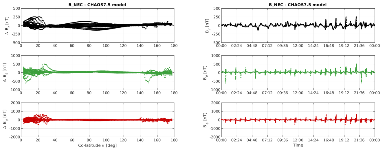
Figure 3-10: S/C A day 17/06: time series of B_{NEC} - B_{Chaos} residuals (right) and B_{NEC} - B_{Chaos} vs colatitude (left).
