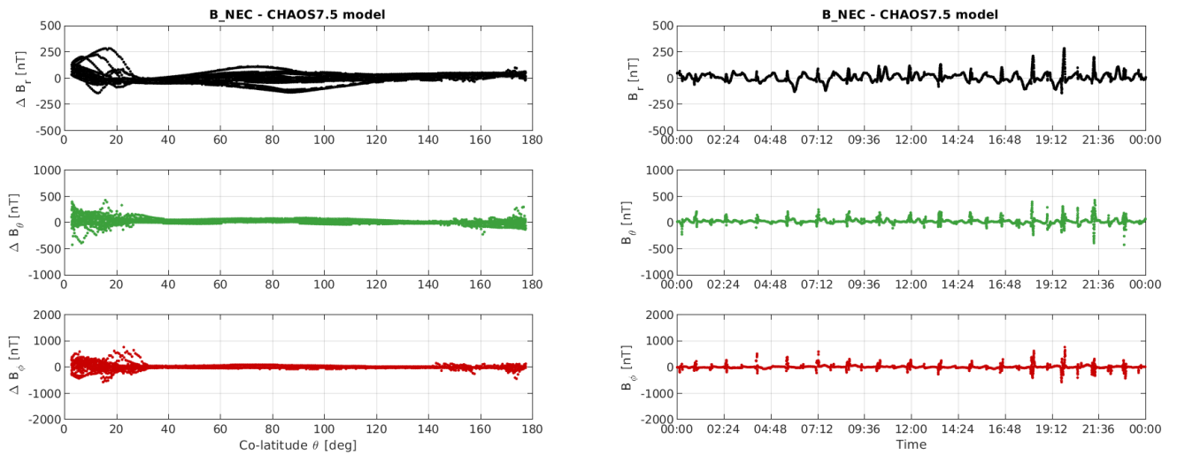
Figure 3-10: S/C A day 10/06: time series of B_{NEC} - B_{Chaos} residuals (right) and B_{NEC} - B_{Chaos} vs colatitude (left).
