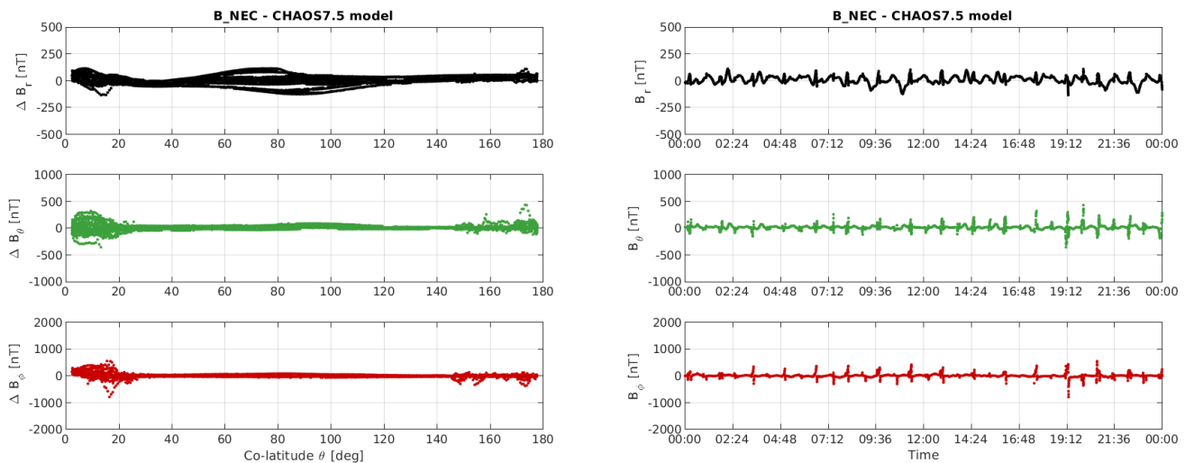
Figure 3-11: S/C B day 10/06: time series of B_{NEC} - B_{Chaos} residuals (right) and B_{NEC} - B_{Chaos} vs colatitude (left).
