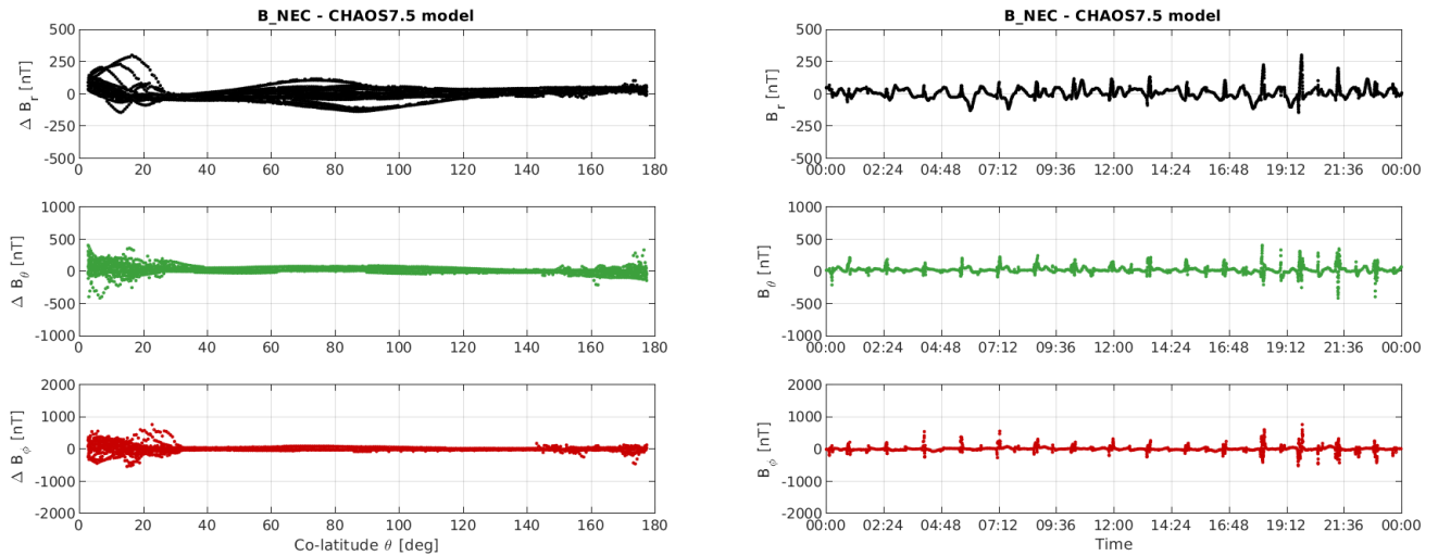
Figure 3-12: S/C C day 10/06: time series of B_{NEC} - B_{Chaos} residuals (right) and B_{NEC} - B_{Chaos} vs colatitude (left)
