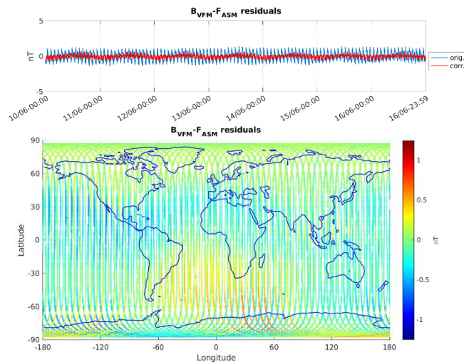
Figure 3-5: ASM-VFM residuals for S/C A, during monitoring period 10/06-16/06. In top figure are plotted: difference between |B_{VFM}| and F_{ASM} (without dB_{Sun} correction) (blue colour), and the residuals with dB_{Sun} corrections (red colour). In bottom figure residuals are presented on the world map.
