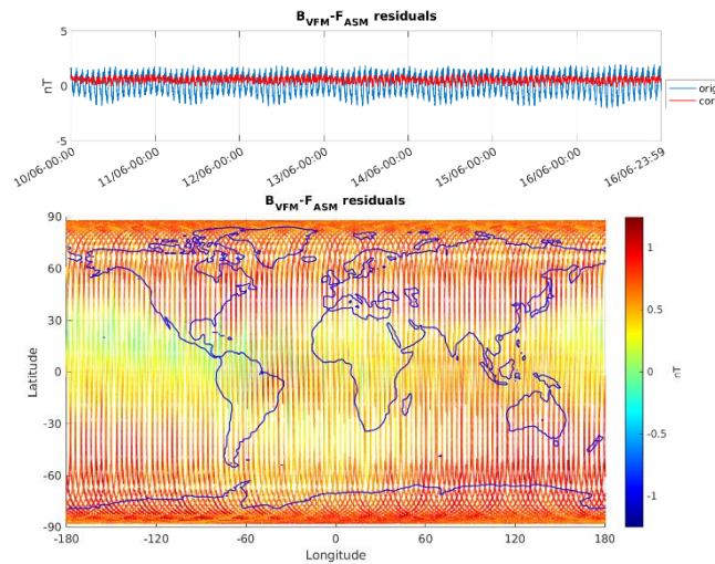
Figure 3-6: ASM-VFM residuals for S/C B, during monitoring period 10/06-16/06. In top figure are plotted: difference between |B_{VFM}| and F_{ASM} (without dB_Sun correction) (blue colour), and the residuals with dB_Sun corrections (red colour). In bottom figure residuals are presented on the world map.
