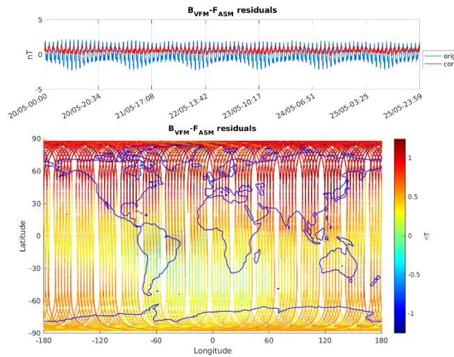
Figure 3-6: ASM-VFM residuals for S/C B, during monitoring period 20/05-26/05. In top figure are plotted: difference between |B_{VFM}| and F_{ASM} (without dB_{Sun} correction) (blue colour), and the residuals with dB_{Sun} corrections (red colour). In bottom figure residuals are presented on the world map.
