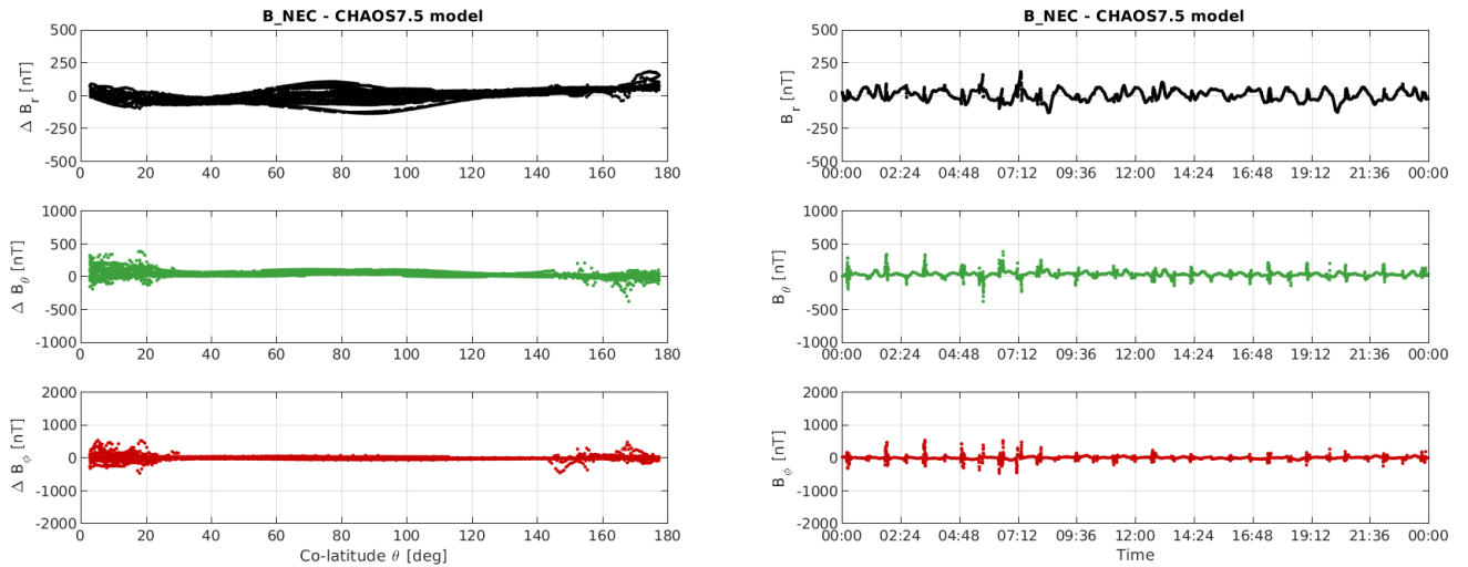
Figure 3-12: S/C C day 20.05: time series of B_{NEC} - B_{Chaos} residuals (right) and B_{NEC} - B_{Chaos} vs colatitude (left)
