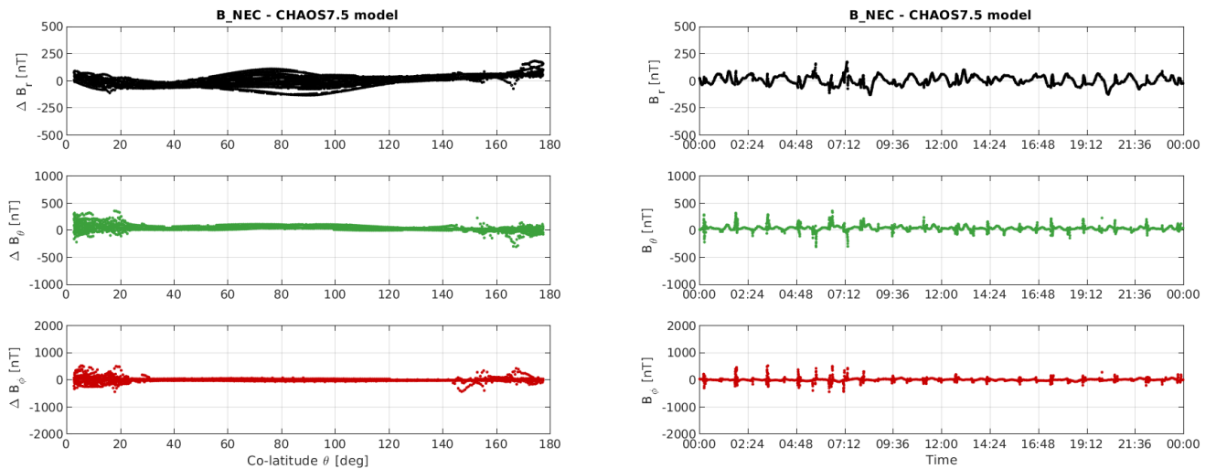
Figure 3-10: S/C A day 20.05: time series of B_{NEC} - B_{Chaos} residuals (right) and B_{NEC} - B_{Chaos} vs colatitude (left).
