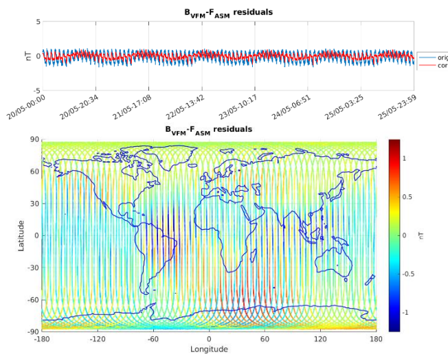
Figure 3-5: ASM-VFM residuals for S/C A, during monitoring period 20/05-26/05. In top figure are plotted: difference between |B_{VFM}| and F_{ASM} (without dB_{Sun} correction) (blue colour), and the residuals with dB_{Sun} corrections (red colour). In bottom figure residuals are presented on the world map.
