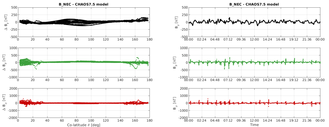
Figure 3-11: S/C B day 20.05: time series of B_{NEC} - B_{Chaos} residuals (right) and B_{NEC} - B_{Chaos} vs colatitude (left).
