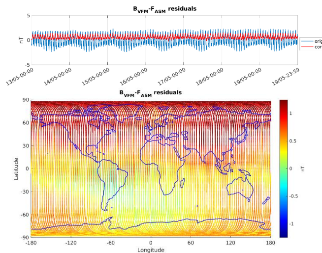
Figure 3-6: ASM-VFM residuals for S/C B, during monitoring period 13/05-19/05. In top figure are plotted: difference between |B_{VFM}| and F_{ASM} (without dB_{Sun} correction) (blue colour), and the residuals with dB_{Sun} corrections (red colour). In bottom figure residuals are presented on the world map.
