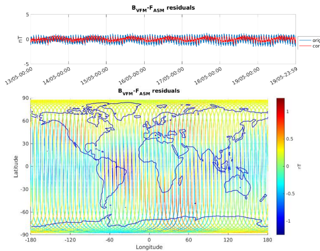
Figure 3-5: ASM-VFM residuals for S/C A, during monitoring period 13/05-19/05. In top figure are plotted: difference between |B_{VFM}| and F_{ASM} (without dB_{Sun} correction) (blue colour), and the residuals with dB_{Sun} corrections (red colour). In bottom figure residuals are presented on the world map.
