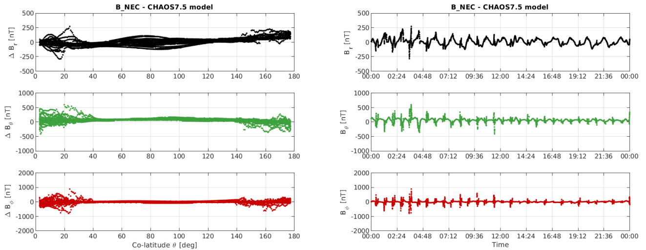
Figure 3-12: S/C C day 13/05: time series of B_{NEC} - B_{Chaos} residuals (right) and B_{NEC} - B_{Chaos} vs colatitude (left)
