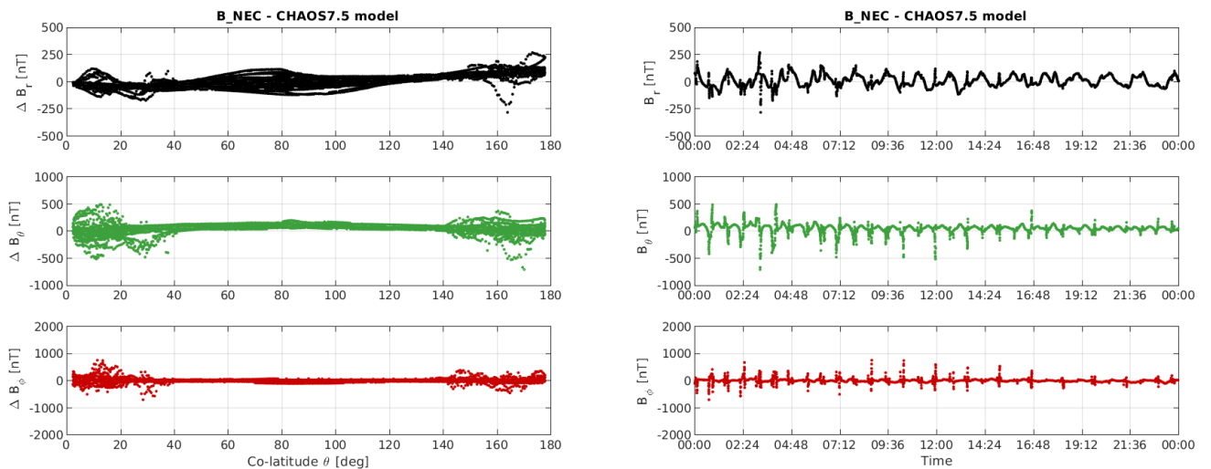
Figure 3-11: S/C B day 13/05: time series of B_{NEC} - B_{Chaos} residuals (right) and B_{NEC} - B_{Chaos} vs colatitude (left).
