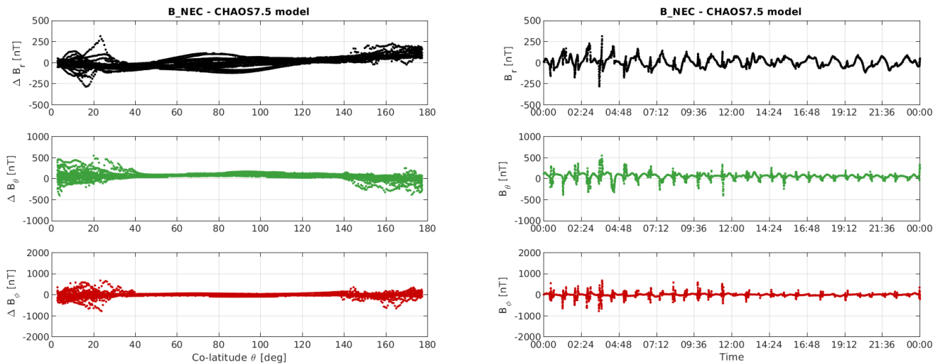
Figure 3-10: S/C A day 13/05: time series of B_{NEC} - B_{Chaos} residuals (right) and B_{NEC} - B_{Chaos} vs colatitude (left).
