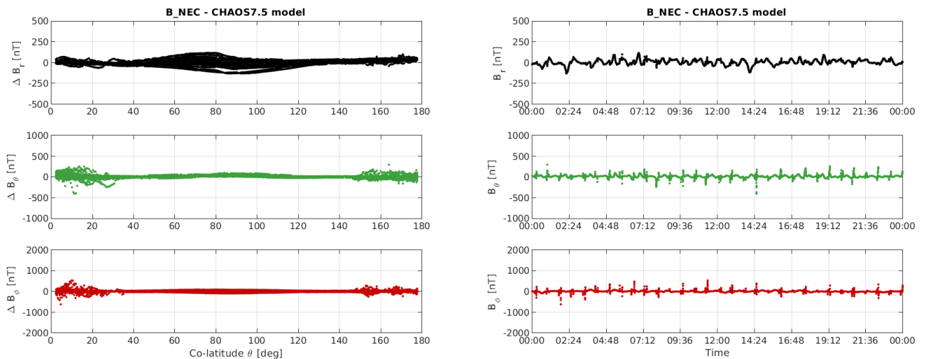
Figure 3-11: S/C B day 29/04: time series of B_{NEC} - B_{Chaos} residuals (right) and B_{NEC} - B_{Chaos} vs colatitude (left).
