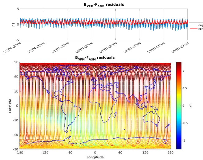
Figure 3-6: ASM-VFM residuals for S/C B, during monitoring period 29/04-05/05. In top figure are plotted: difference between |B_{VFM}| and F_{ASM} (without dB_{Sun} correction) (blue colour), and the residuals with dB_{Sun} corrections (red colour). In bottom figure residuals are presented on the world map.
