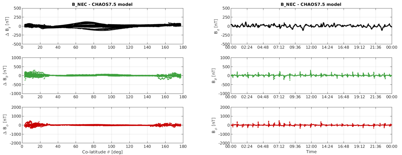
Figure 3-12: S/C C day 29/04: time series of B_{NEC} - B_{Chaos} residuals (right) and B_{NEC} - B_{Chaos} vs colatitude (left)
