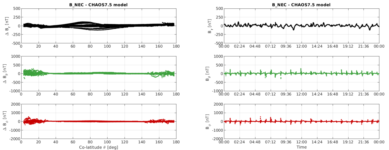
Figure 3-10: S/C A day 29/04: time series of B_{NEC} - B_{Chaos} residuals (right) and B_{NEC} - B_{Chaos} vs colatitude (left).
