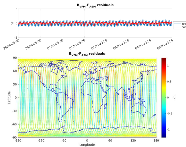
Figure 3-5: ASM-VFM residuals for S/C A, during monitoring period 29/04-05/05. In top figure are plotted: difference between |B_{VFM}| and F_{ASM} (without dB_{Sun} correction) (blue colour), and the residuals with dB_{Sun} corrections (red colour). In bottom figure residuals are presented on the world map.
