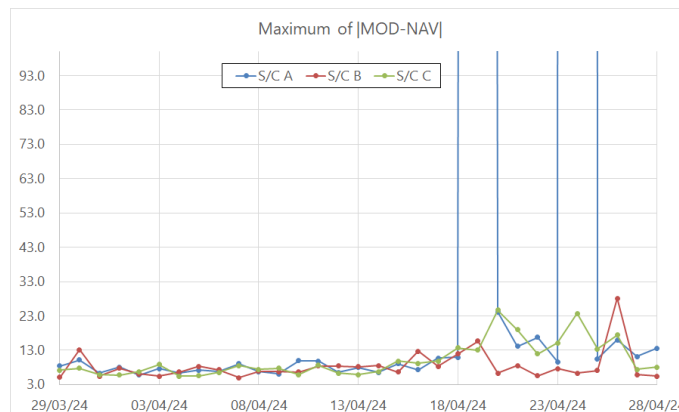
Figure 3-2: Plot of the maximum difference of the absolute value of the difference between MOD and NAV solutions for all satellites. Plot covers last month of operation. Data peak in S/C-A on 24 th April was caused by multiple data gaps caused due to GPSR Synch Loss anomaly.
