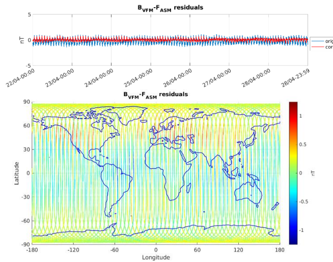
Figure 3-5: ASM-VFM residuals for S/C A, during monitoring period 22/04-28/04. In top figure are plotted: difference between |B_{VFM}| and F_{ASM} (without dB_{Sun} correction) (blue colour), and the residuals with dB_{Sun} corrections (red colour). In bottom figure residuals are presented on the world map.
