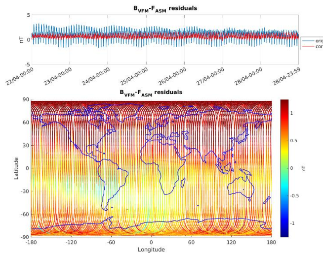
Figure 3-6: ASM-VFM residuals for S/C B, during monitoring period 22/04-28/04. In top figure are plotted: difference between |B_{VFM}| and F_{ASM} (without dB_{Sun} correction) (blue colour), and the residuals with dB_{Sun} corrections (red colour). In bottom figure residuals are presented on the world map.
