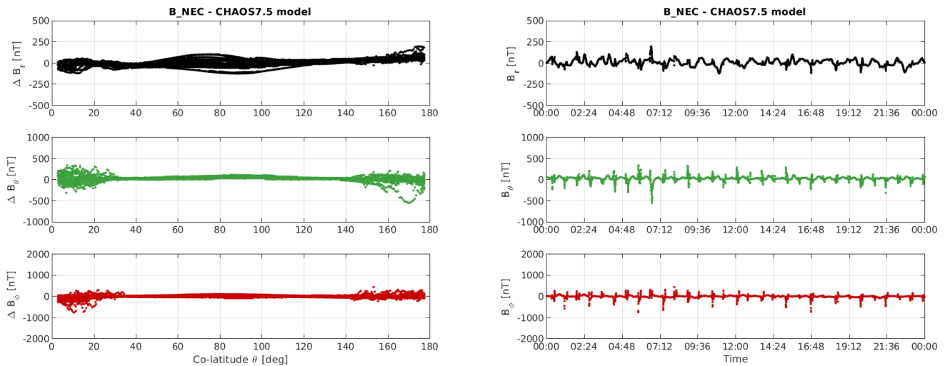
Figure 3-10: S/C A day 22/04: time series of B_{NEC} - B_{Chaos} residuals (right) and B_{NEC} - B_{Chaos} vs colatitude (left).
