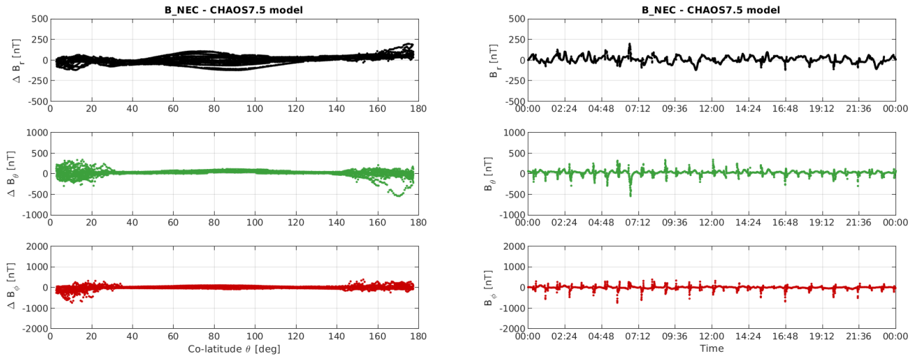
Figure 3-12: S/C C day 22/04: time series of B_{NEC} - B_{Chaos} residuals (right) and B_{NEC} - B_{Chaos} vs colatitude (left)
