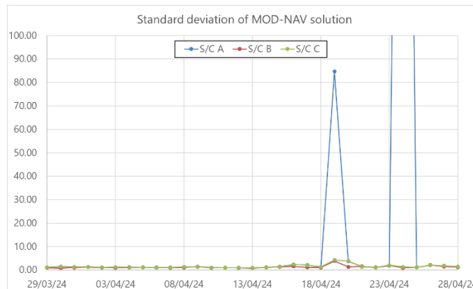
Figure 3-1: Plot of the standard deviation of the difference between MOD and NAV solutions for all satellites. Plot covers last month of operation. Data peak in S/C-A on 24 th April was caused by multiple data gaps caused due to GPSR Synch Loss anomaly.
