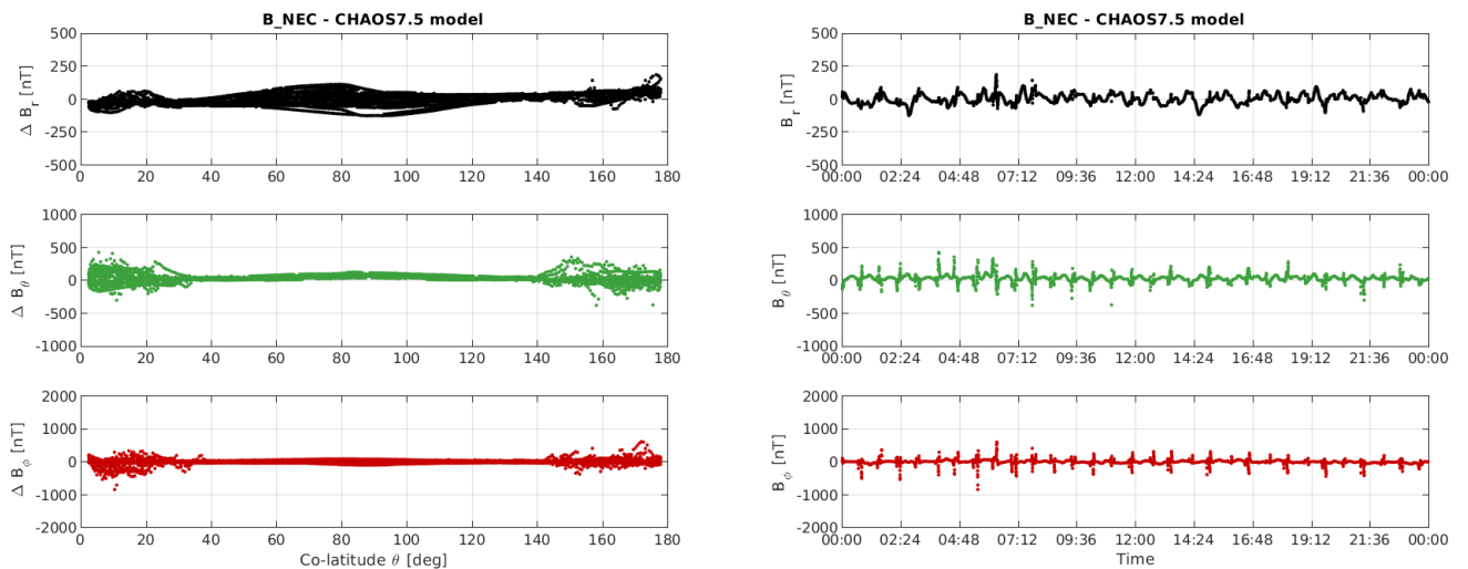
Figure 3-11: S/C B day 22/04: time series of B_{NEC} - B_{Chaos} residuals (right) and B_{NEC} - B_{Chaos} vs colatitude (left).
