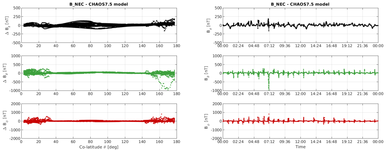
Figure 3-12: S/C C day 08/04: time series of B_{NEC} - B_{Chaos} residuals (right) and B_{NEC} - B_{Chaos} vs colatitude (left)
