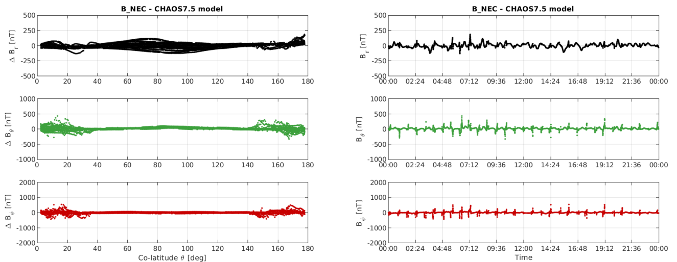
Figure 3-11: S/C B day 08/04: time series of B_{NEC} - B_{Chaos} residuals (right) and B_{NEC} - B_{Chaos} vs colatitude (left).
