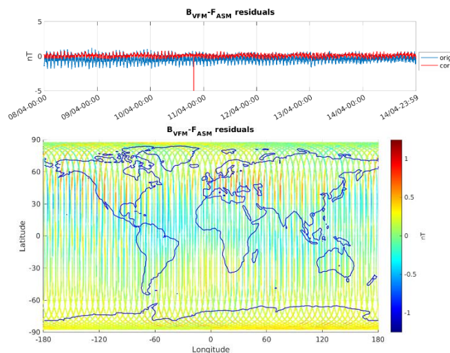
Figure 3-5: ASM-VFM residuals for S/C A, during monitoring period 08/04-14/04. In top figure are plotted: difference between |B_{VFM}| and F_{ASM} (without dB_{Sun} correction) (blue colour), and the residuals with dB_{Sun} corrections (red
