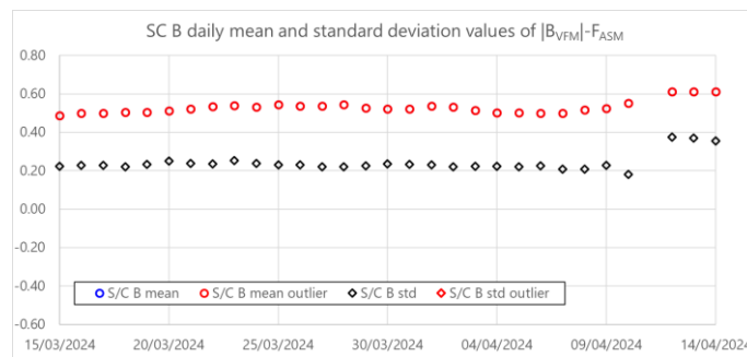
Figure 3-4: Daily mean and standard deviation values of ASM-VFM residuals (defined as dF=|B_{VFM}|-F_{ASM} ) for S/C B. A data gap on 11 th April is caused by anomaly which triggered VFM switch-off due to MonID 603.
