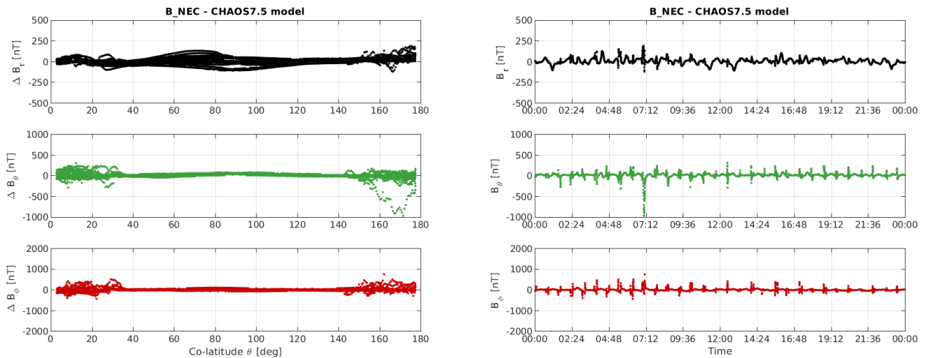
Figure 3-10: S/C A day 08/04: time series of B_{NEC} - B_{Chaos} residuals (right) and B_{NEC} - B_{Chaos} vs colatitude (left).
