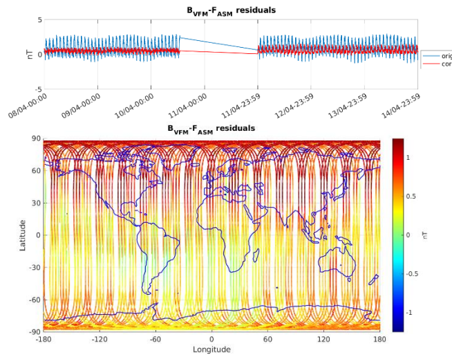
Figure 3-6: ASM-VFM residuals for S/C B, during monitoring period 08/04-14/04. In top figure are plotted: difference between |B_{VFM}| and F_{ASM} (without dB_{Sun} correction) (blue colour), and the residuals with dB_{Sun} corrections (red colour). In bottom figure residuals are presented on the world map. Residuals outlier on 10 th April is coming from the data gaps present in all instruments data from 19:33:20 to 19:34:27.. A data gap on 10-11 th April is caused by anomaly which triggered VFM switch-off due to MonID 603.
