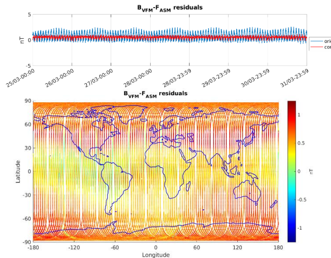
Figure 3-6: ASM-VFM residuals for S/C B, during monitoring period 25/03-31/03. In top figure are plotted: difference between |B_{VFM}| and F_{ASM} (without dB_{Sun} correction) (blue colour), and the residuals with dB_{Sun} corrections (red colour). In bottom figure residuals are presented on the world map.
