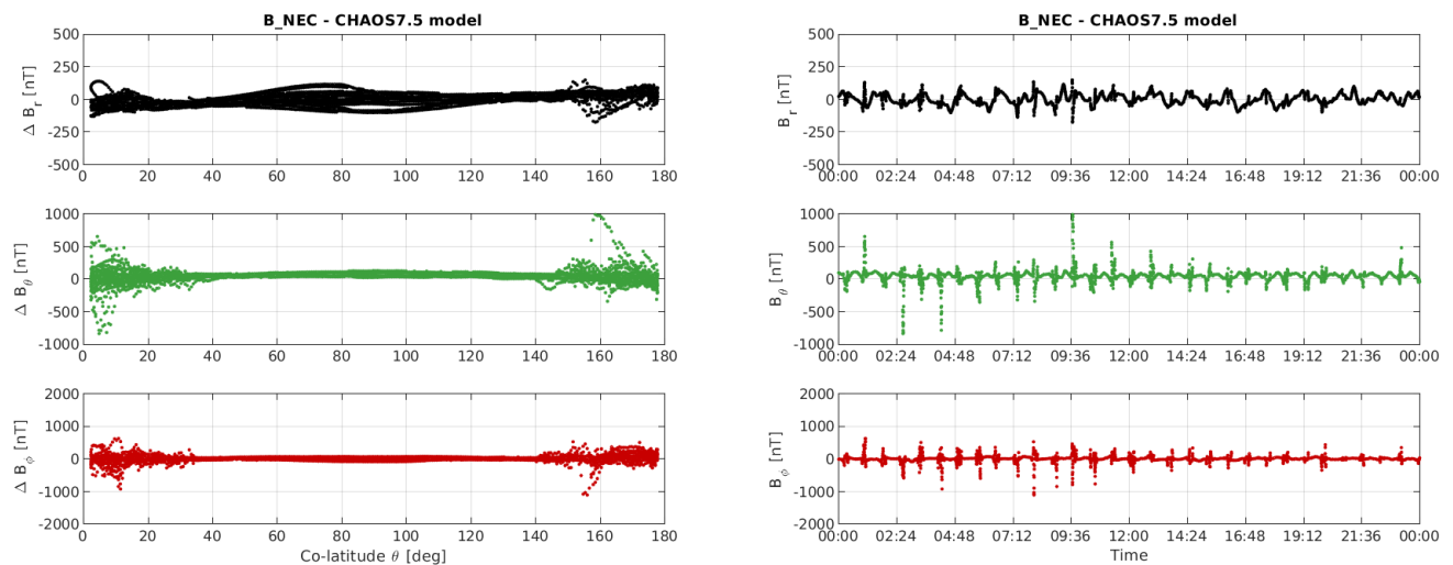
Figure 3-11: S/C B day 25/03: time series of B_{NEC} - B_{chaos} residuals (right) and B_{NEC} - B_{chaos} vs colatitude (left).
