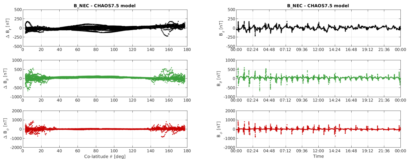
Figure 3-12: S/C C day 25/03: time series of B_{NEC} - B_{Chaos} residuals (right) and B_{NEC} - B_{Chaos} vs colatitude (left)
