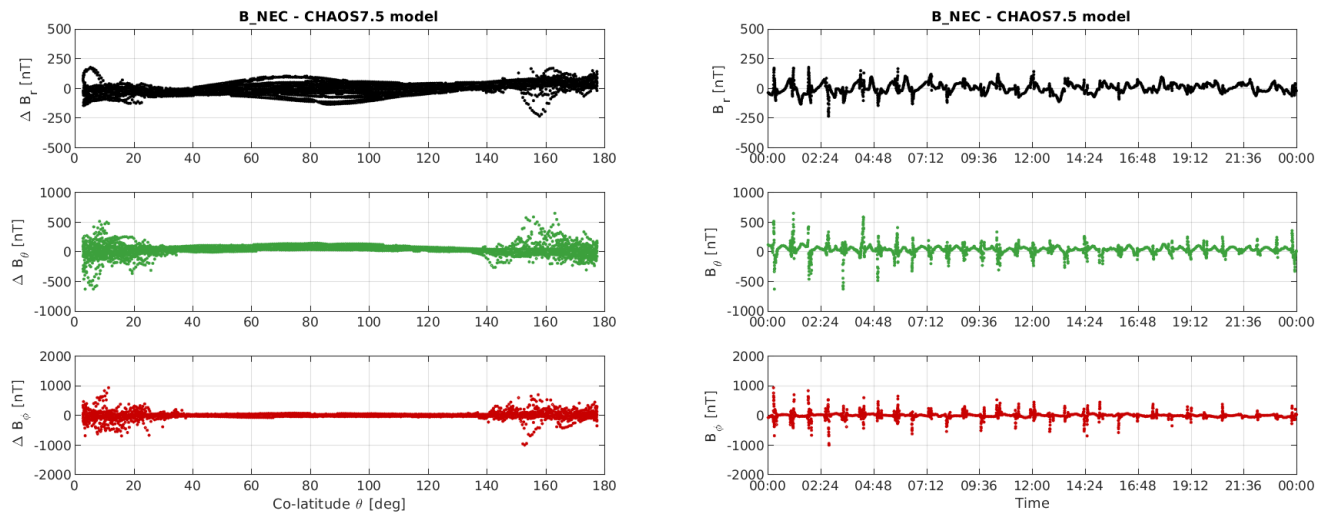
Figure 3-10: S/C A day 25/03: time series of B_{NEC} - B_{chaos} residuals (right) and B_{NEC} - B_{chaos} vs colatitude (left).
