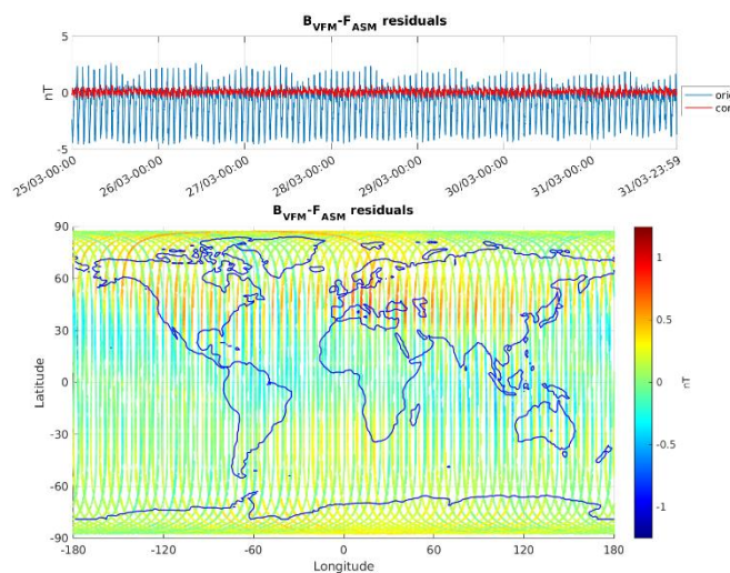
Figure 3-5: ASM-VFM residuals for S/C A, during monitoring period 25/03-31/03. In top figure are plotted: difference between |B_{VFM}| and F_{ASM} (without dB_{Sun} correction) (blue colour), and the residuals with dB_{Sun} corrections (red colour). In bottom figure residuals are presented on the world map.
