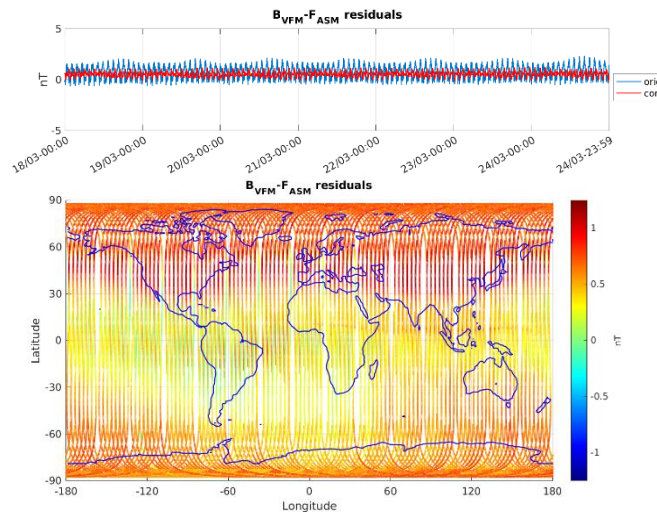
Figure 3-6: ASM-VFM residuals for S/C B, during monitoring period 18/03-24/03. In top figure are plotted: difference between |B_{VFM}| and F_{ASM} (without dB_{Sun} correction) (blue colour), and the residuals with dB_{Sun} corrections (red colour). In bottom figure residuals are presented on the world map.
