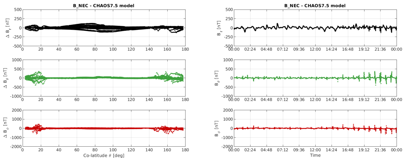
Figure 3-12: S/C C day 18/03: time series of B_{NEC} - B_{Chaos} residuals (right) and B_{NEC} - B_{Chaos} vs colatitude (left)
