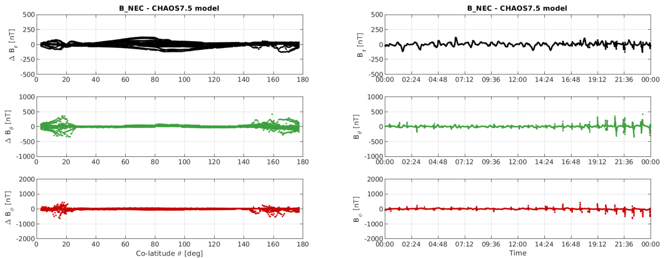
Figure 3-10: S/C A day 18/03: time series of B_{NEC} - B_{chaos} residuals (right) and B_{NEC} - B_{chaos} vs colatitude (left).
