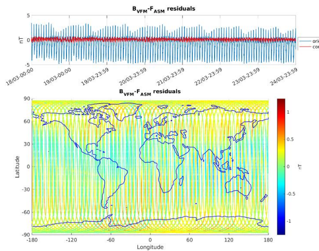
Figure 3-5: ASM-VFM residuals for S/C A, during monitoring period 18/03-24/03. In top figure are plotted: difference between |B_{VFM}| and F_{ASM} (without dB_{Sun} correction) (blue colour), and the residuals with dB_{Sun} corrections (red colour). In bottom figure residuals are presented on the world map.
