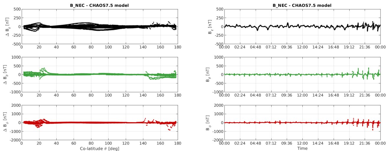
Figure 3-11: S/C B day 18/03: time series of B_{NEC} - B_{chaos} residuals (right) and B_{NEC} - B_{chaos} vs colatitude (left).
