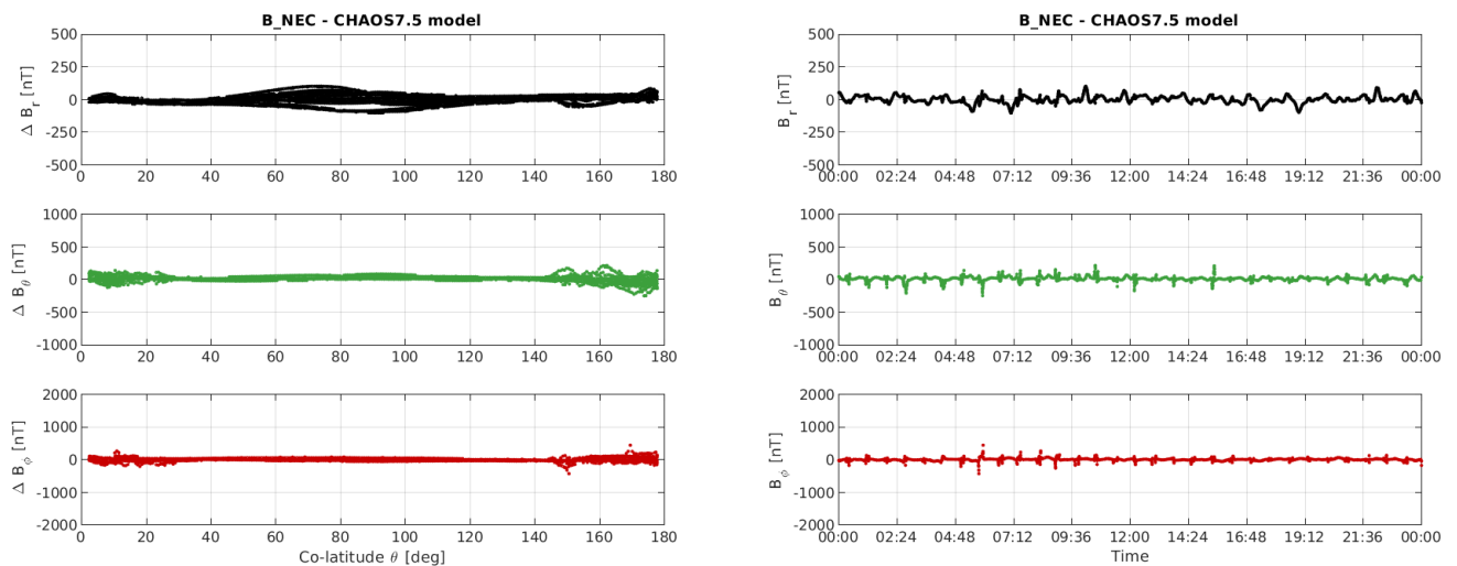
Figure 3-11: S/C B day 11/03: time series of B_{NEC} - B_{chaos} residuals (right) and B_{NEC} - B_{chaos} vs colatitude (left).
