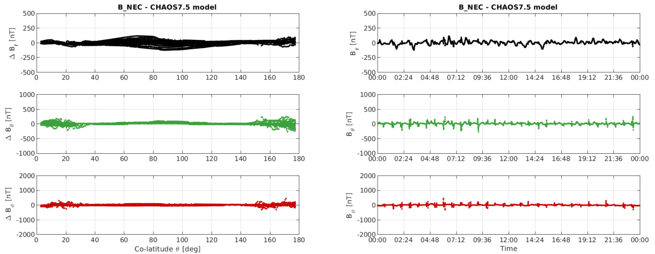
Figure 3-12: S/C C day 11/03: time series of B_{NEC} - B_{Chaos} residuals (right) and B_{NEC} - B_{Chaos} vs colatitude (left)
