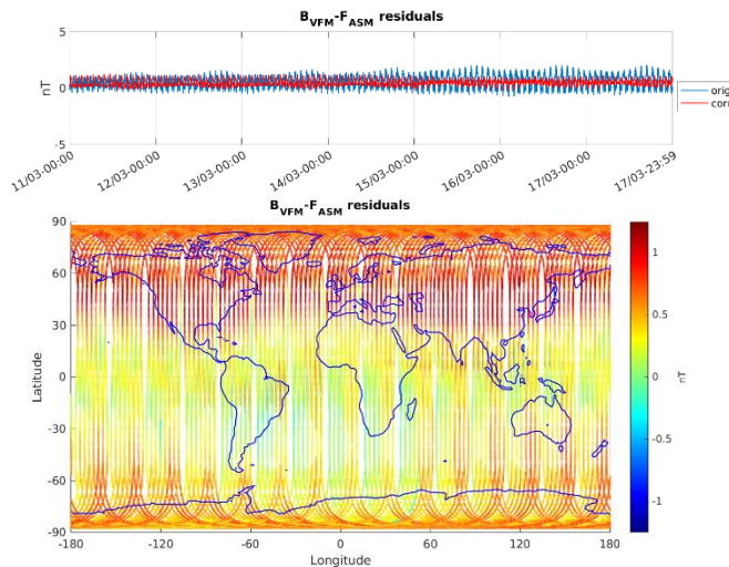
Figure 3-6: ASM-VFM residuals for S/C B, during monitoring period 11/03-17/03. In top figure are plotted: difference between |B_{VFM}| and F_{ASM} (without dB_{Sun} correction) (blue colour), and the residuals with dB_{Sun} corrections (red colour). In bottom figure residuals are presented on the world map.
