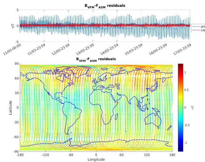
Figure 3-5: ASM-VFM residuals for S/C A, during monitoring period 11/03-17/03. In top figure are plotted: difference between |B_{VFM}| and F_{ASM} (without dB_{Sun} correction) (blue colour), and the residuals with dB_{Sun} corrections (red colour). In bottom figure residuals are presented on the world map.
