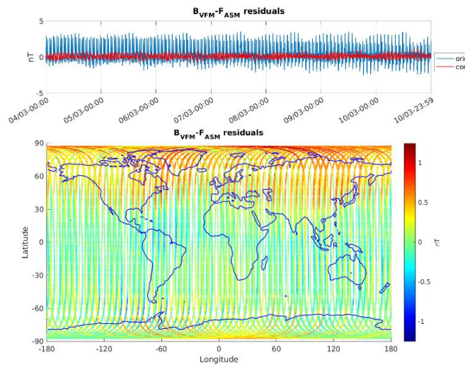
Figure 3-5: ASM-VFM residuals for S/C A, during monitoring period 04/03-10/03. In top figure are plotted: difference between |B_{VFM}| and F_{ASM} (without dB_{Sun} correction) (blue colour), and the residuals with dB_{Sun} corrections (red colour). In bottom figure residuals are presented on the world map.
