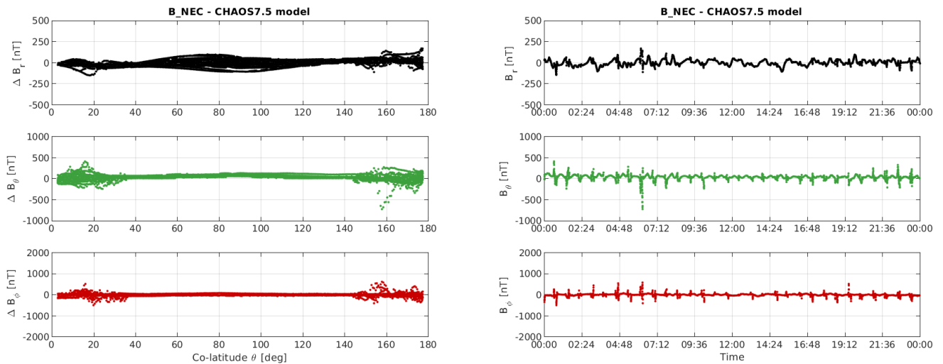
Figure 3-10: S/C A day 04/03: time series of B_{NEC} - B_{chaos} residuals (right) and B_{NEC} - B_{chaos} vs colatitude (left).
