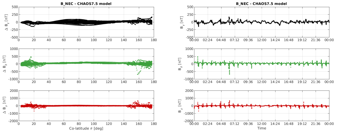
Figure 3-12: S/C C day 04/03: time series of B_{NEC} - B_{Chaos} residuals (right) and B_{NEC} - B_{Chaos} vs colatitude (left)
