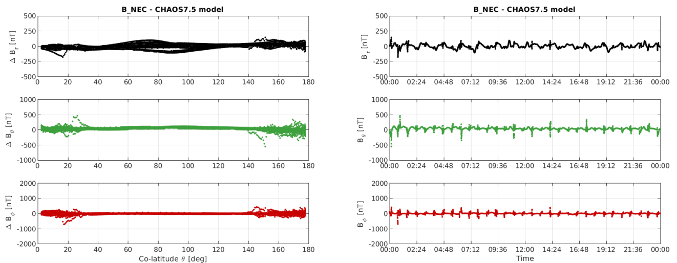
Figure 3-11: S/C B day 04/03: time series of B_{NEC} - B_{chaos} residuals (right) and B_{NEC} - B_{chaos} vs colatitude (left).
