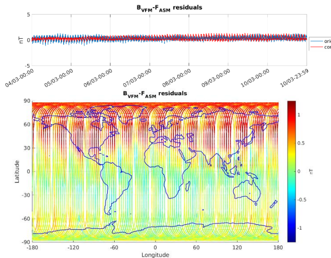
Figure 3-6: ASM-VFM residuals for S/C B, during monitoring period 04/03-10/03. In top figure are plotted: difference between |B_{VFM}| and F_{ASM} (without dB_{Sun} correction) (blue colour), and the residuals with dB_{Sun} corrections (red colour). In bottom figure residuals are presented on the world map.
