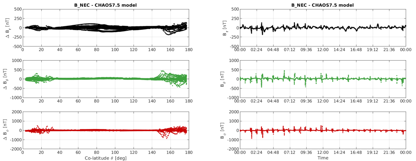
Figure 3-10: S/C A day 26/02: time series of B_{NEC} - B_{chaos} residuals (right) and B_{NEC} - B_{chaos} vs colatitude (left).
