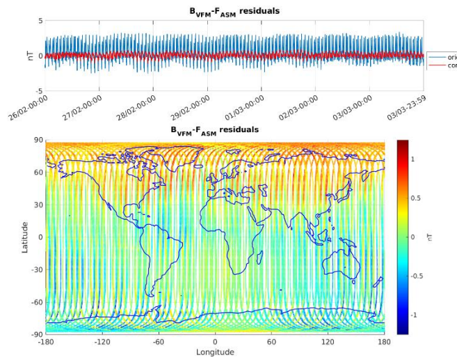
Figure 3-5: ASM-VFM residuals for S/C A, during monitoring period 26/02-03/03. In top figure are plotted: difference between |B_{VFM}| and F_{ASM} (without dB_{Sun} correction) (blue colour), and the residuals with dB_{Sun} corrections (red colour). In bottom figure residuals are presented on the world map.
