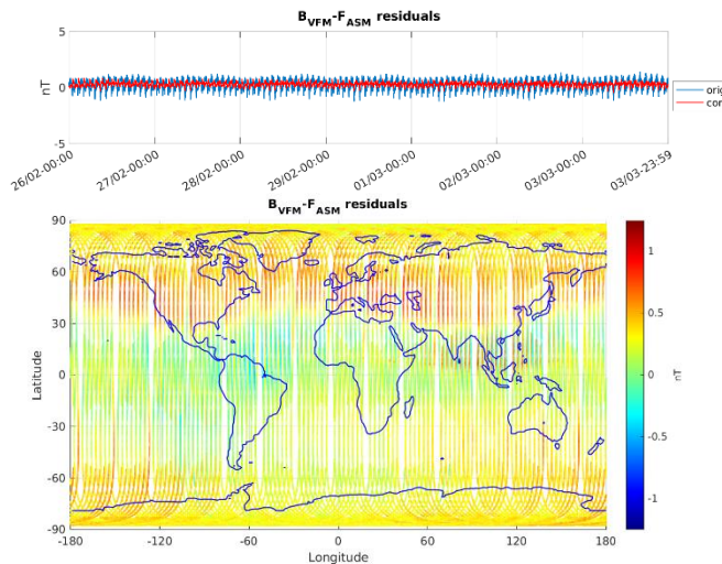
Figure 3-6: ASM-VFM residuals for S/C B, during monitoring period 26/02-03/03. In top figure are plotted: difference between |B_{VFM}| and F_{ASM} (without dB_{Sun} correction) (blue colour), and the residuals with dB_{Sun} corrections (red colour). In bottom figure residuals are presented on the world map.
