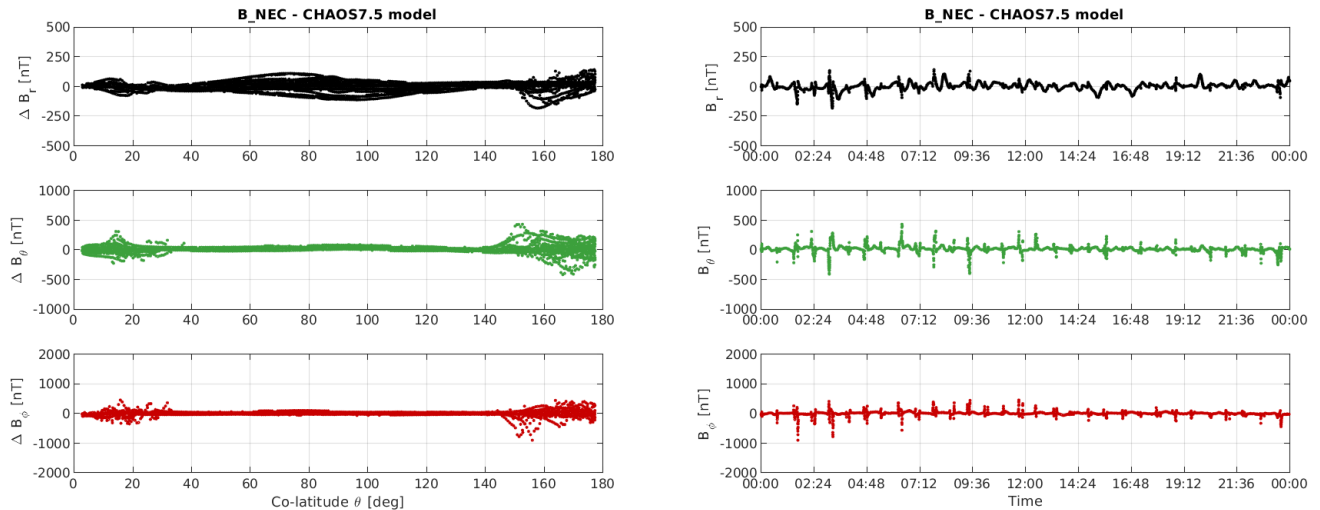
Figure 3-12: S/C C day 26/02: time series of B_{NEC} - B_{Chaos} residuals (right) and B_{NEC} - B_{Chaos} vs colatitude (left)
