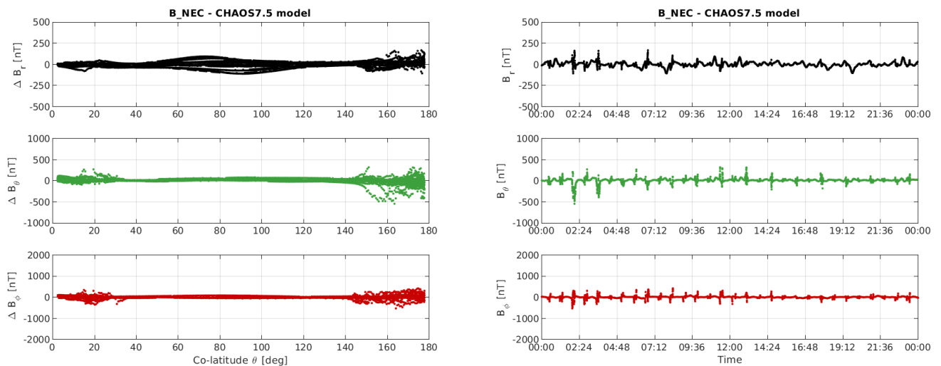
Figure 3-11: S/C B day 26/02: time series of B_{NEC} - B_{chaos} residuals (right) and B_{NEC} - B_{chaos} vs colatitude (left).
