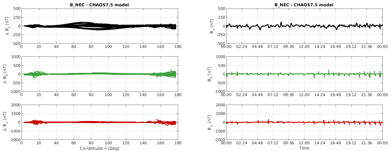
Figure 3-10: S/C A day 19/02: time series of B_{NEC} - B_{chaos} residuals (right) and B_{NEC} - B_{chaos} vs colatitude (left).
