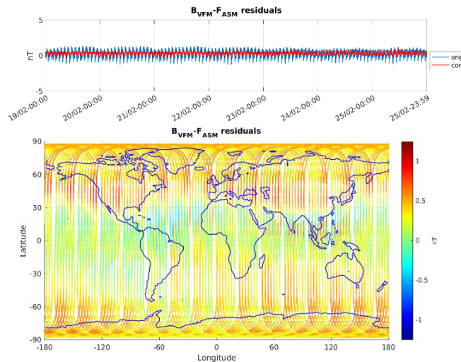
Figure 3-6: ASM-VFM residuals for S/C B, during monitoring period 19/02-25/02. In top figure are plotted: difference between |B_{VFM}| and F_{ASM} (without dB_{Sun} correction) (blue colour), and the residuals with dB_{Sun} corrections (red colour). In bottom figure residuals are presented on the world map.
