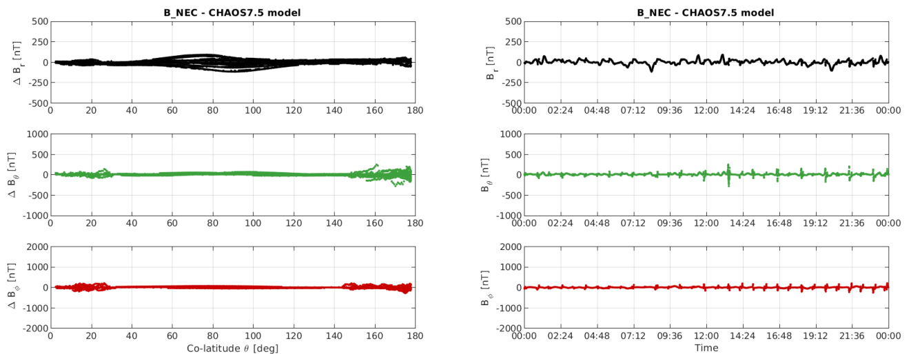
Figure 3-11: S/C B day 19/02: time series of B_{NEC} - B_{chaos} residuals (right) and B_{NEC} - B_{chaos} vs colatitude (left).
