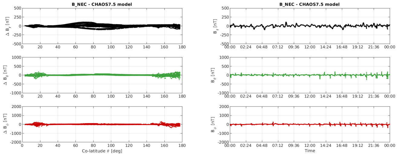
Figure 3-12: S/C C day 19/02: time series of B_{NEC} - B_{Chaos} residuals (right) and B_{NEC} - B_{Chaos} vs colatitude (left)
