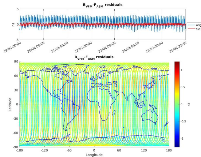
Figure 3-5: ASM-VFM residuals for S/C A, during monitoring period 19/02-25/02. In top figure are plotted: difference between |B_{VFM}| and F_{ASM} (without dB_{Sun} correction) (blue colour), and the residuals with dB_{Sun} corrections (red colour). In bottom figure residuals are presented on the world map.
