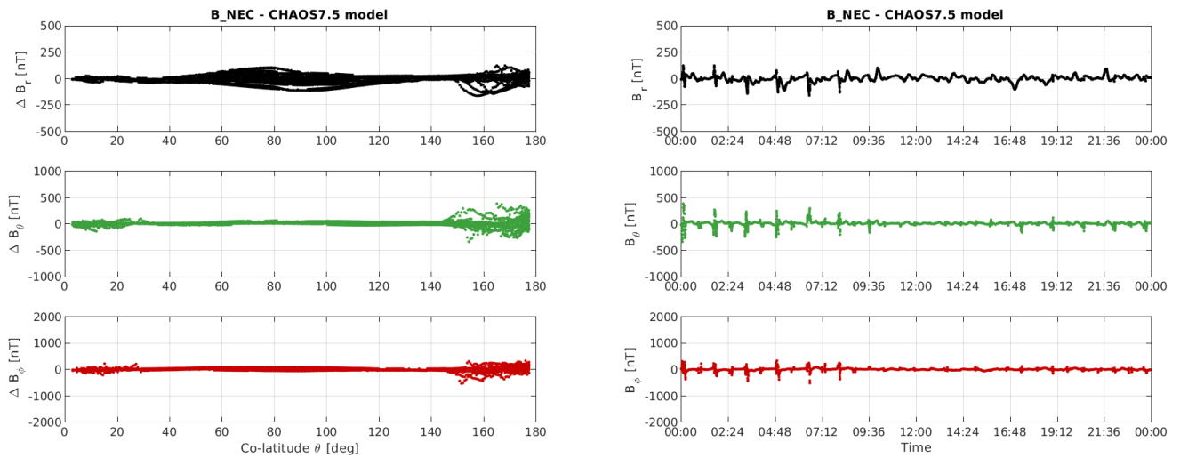
Figure 3-10: S/C A day 12/02: time series of B_{NEC} - B_{chaos} residuals (right) and B_{NEC} - B_{chaos} vs colatitude (left).
