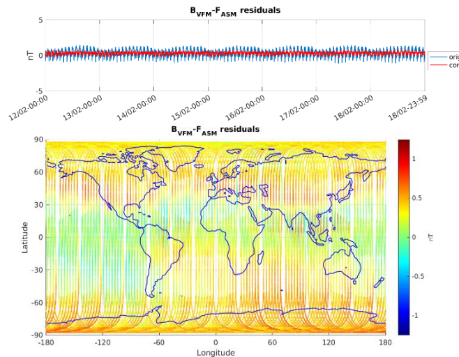
Figure 3-6: ASM-VFM residuals for S/C B, during monitoring period 12/02-18/02. In top figure are plotted: difference between |B_{VFM}| and F_{ASM} (without dB_{Sun} correction) (blue colour), and the residuals with dB_{Sun} corrections (red colour). In bottom figure residuals are presented on the world map.
