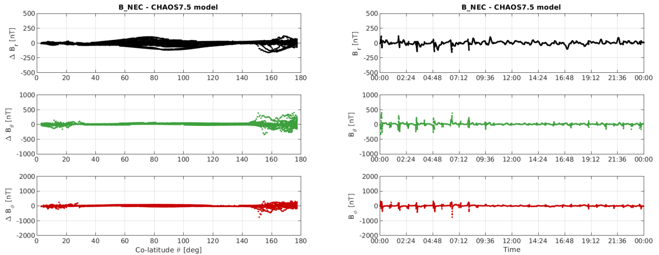
Figure 3-12: S/C C day 12/02: time series of B_{NEC} - B_{Chaos} residuals (right) and B_{NEC} - B_{Chaos} vs colatitude (left)
