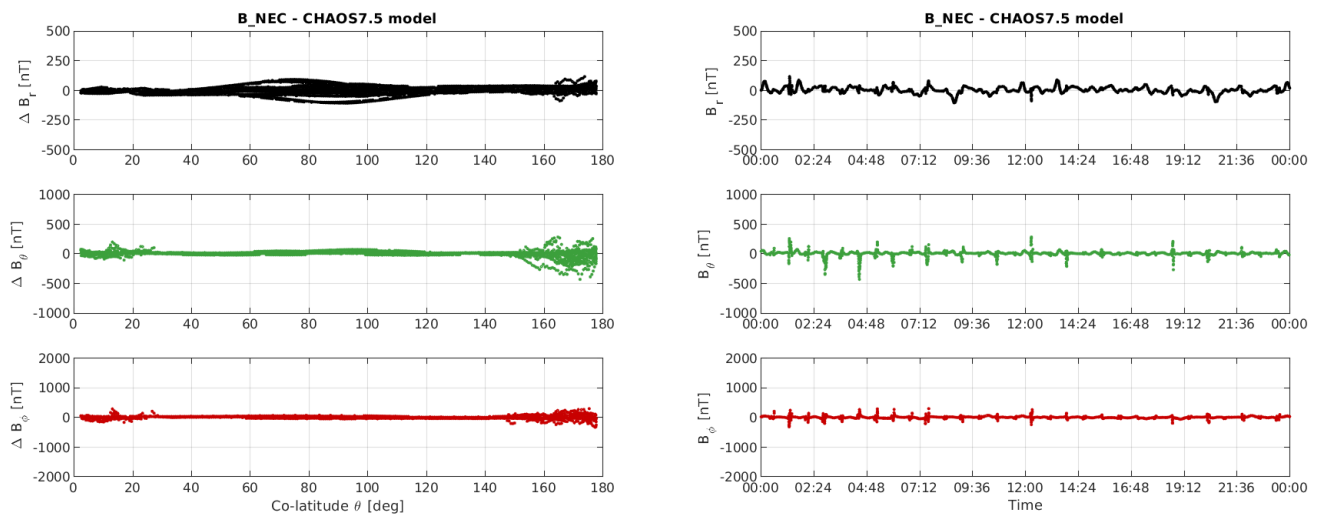
Figure 3-11: S/C B day 12/02: time series of B_{NEC} - B_{chaos} residuals (right) and B_{NEC} - B_{chaos} vs colatitude (left).
