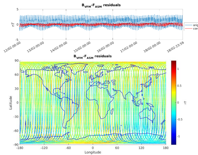
Figure 3-5: ASM-VFM residuals for S/C A, during monitoring period 12/02-18/02. In top figure are plotted: difference between |B_{VFM}| and F_{ASM} (without dB_{Sun} correction) (blue colour), and the residuals with dB_{Sun} corrections (red colour). In bottom figure residuals are presented on the world map.
