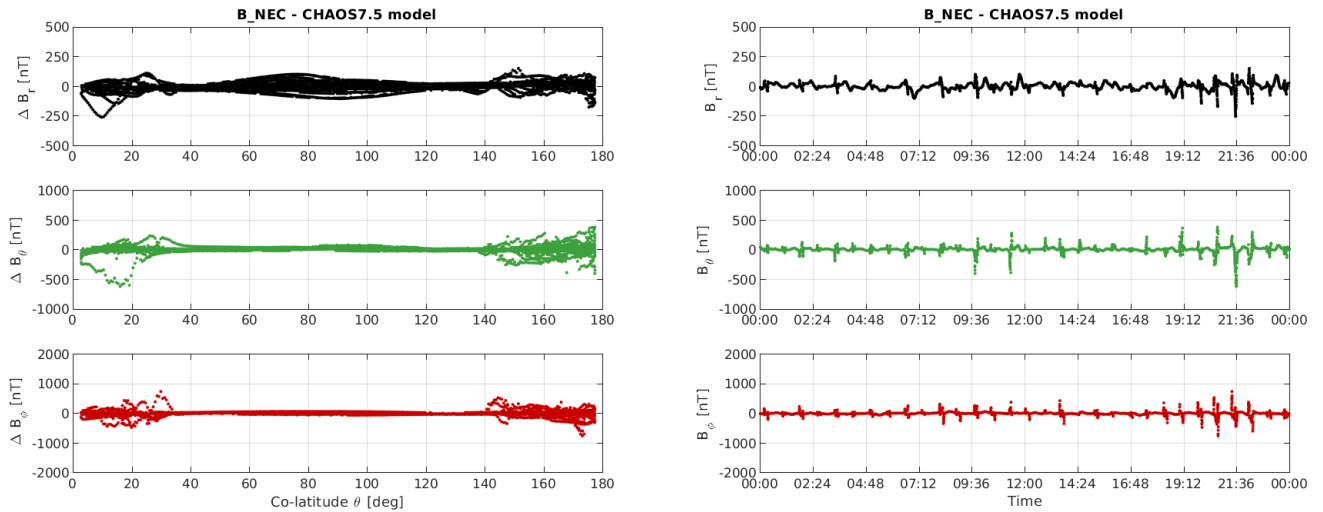
Figure 3-12: S/C C day 22.01: time series of B_{NEC} - B_{Chaos} residuals (right) and B_{NEC} - B_{Chaos} vs colatitude (left)
