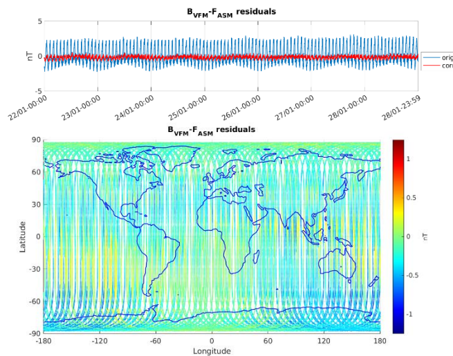
Figure 3-5: ASM-VFM residuals for S/C A, during monitoring period 22/01-28/01. In top figure are plotted: difference between |B_{VFM}| and F_{ASM} (without dB_{Sun} correction) (blue colour), and the residuals with dB_{Sun} corrections (red colour). In bottom figure residuals are presented on the world map.
