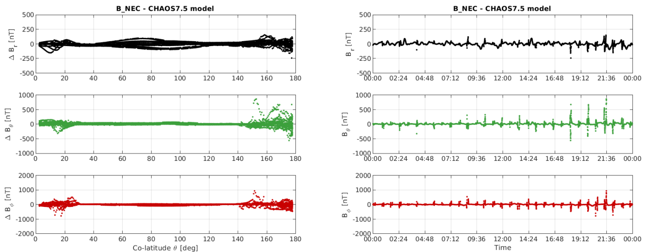
Figure 3-11: S/C B day 22.01: time series of B_{NEC} - B_{Chaos} residuals (right) and B_{NEC} - B_{Chaos} vs colatitude (left).
