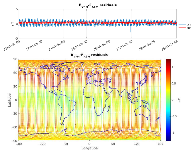
Figure 3-6: ASM-VFM residuals for S/C B, during monitoring period 22/01-28/01. In top figure are plotted: difference between |B_{VFM}| and F_{ASM} (without dB_{Sun} correction) (blue colour), and the residuals with dB_{Sun} corrections (red colour). In bottom figure residuals are presented on the world map.
