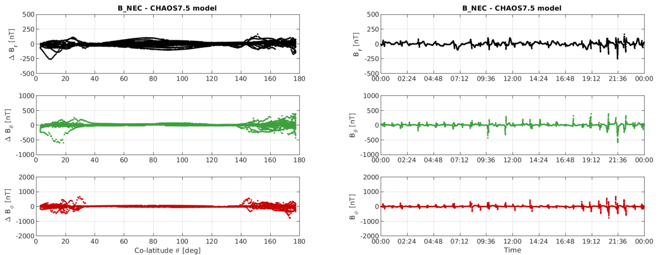
Figure 3-10: S/C A day 22.01: time series of B_{NEC} - B_{Chaos} residuals (right) and B_{NEC} - B_{Chaos} vs colatitude (left).
