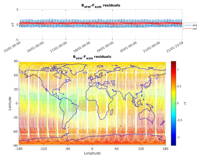
Figure 3-6: ASM-VFM residuals for S/C B, during monitoring period 15/01-21/01. In top figure are plotted: difference between |B_{VFM}| and F_{ASM} (without dB_{Sun} correction) (blue colour), and the residuals with dB_{Sun} corrections (red colour). In bottom figure residuals are presented on the world map.
