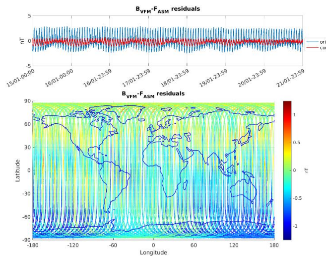
Figure 3-5: ASM-VFM residuals for S/C A, during monitoring period 15/01-21/01. In top figure are plotted: difference between |B_{VFM}| and F_{ASM} (without dB_Sun correction) (blue colour), and the residuals with dB_Sun corrections (red colour). In bottom figure residuals are presented on the world map.
