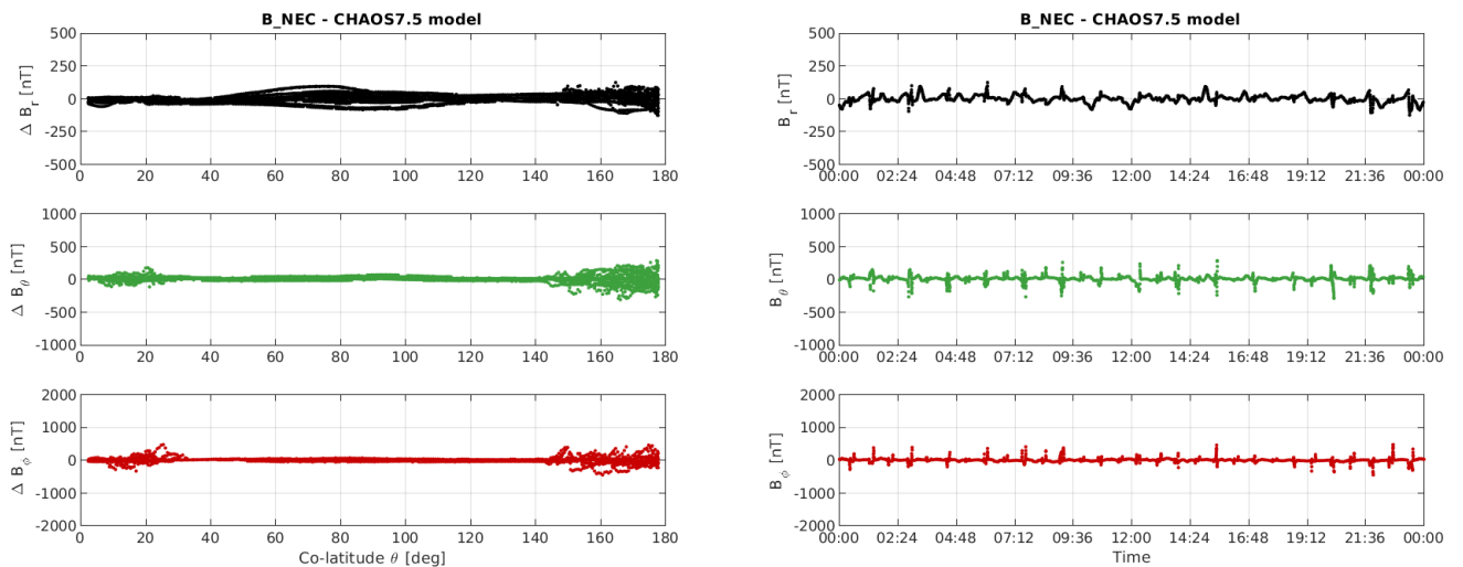
Figure 3-11: S/C B day 15.01: time series of B_{NEC} - B_{Chaos} residuals (right) and B_{NEC} - B_{Chaos} vs colatitude (left).
