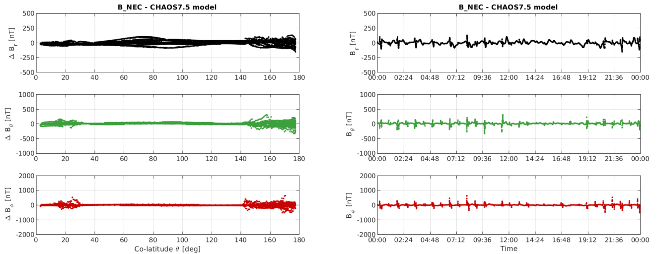
Figure 3-12: S/C C day 15:01: time series of B_{NEC} - B_{Chaos} residuals (right) and B_{NEC} - B_{Chaos} vs colatitude (left)
