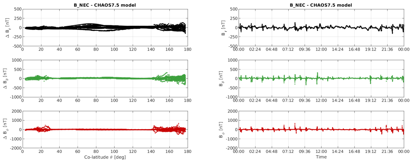
Figure 3-10: S/C A day 15.01: time series of B_{NEC} - B_{Chaos} residuals (right) and B_{NEC} - B_{Chaos} vs colatitude (left).
