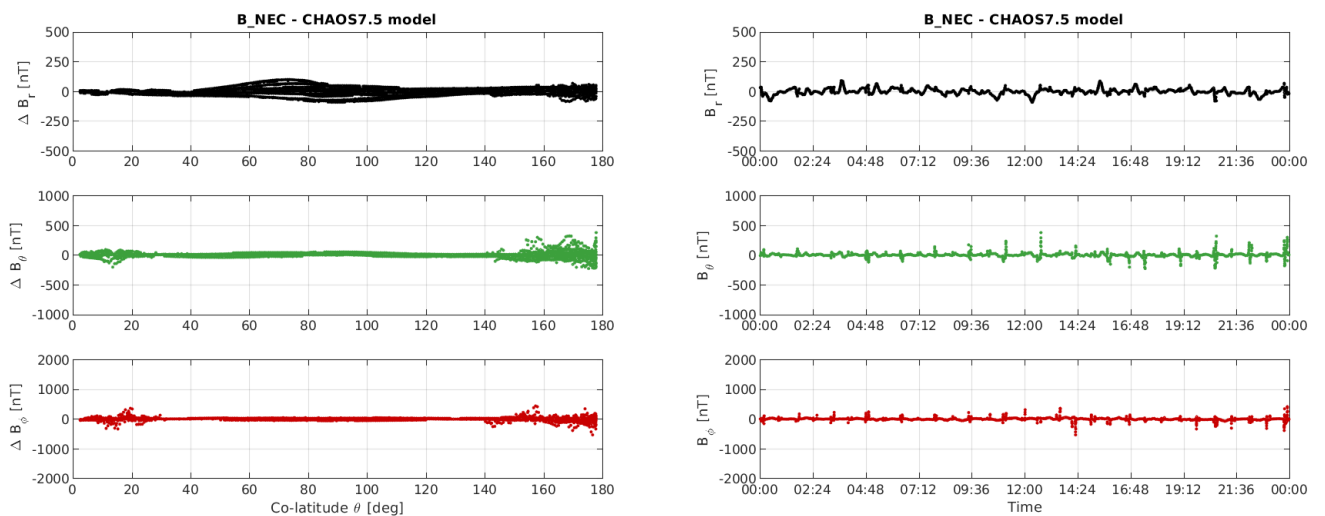
Figure 3-11: S/C B day 08.01: time series of B_{NEC} - B_{Chaos} residuals (right) and B_{NEC} - B_{Chaos} vs colatitude (left).
