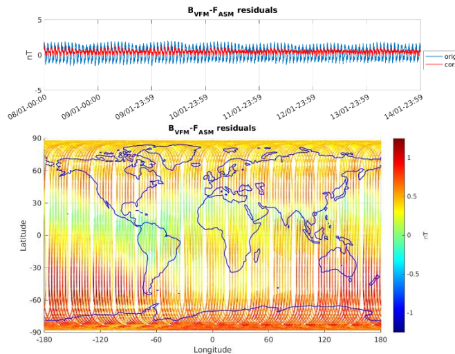
Figure 3-6: ASM-VFM residuals for S/C B, during monitoring period 08/01-14/01. In top figure are plotted: difference between |B_{VFM}| and F_{ASM} (without dB_{Sun} correction) (blue colour), and the residuals with dB_{Sun} corrections (red colour). In bottom figure residuals are presented on the world map.
