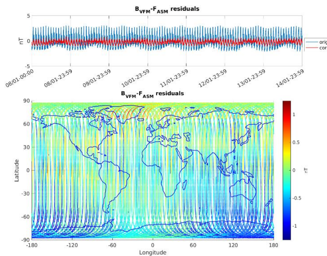
Figure 3-5: ASM-VFM residuals for S/C A, during monitoring period 08/01-14/01. In top figure are plotted: difference between |B_{VFM}| and F_{ASM} (without dB_{Sun} correction) (blue colour), and the residuals with dB_{Sun} corrections (red colour). In bottom figure residuals are presented on the world map.
