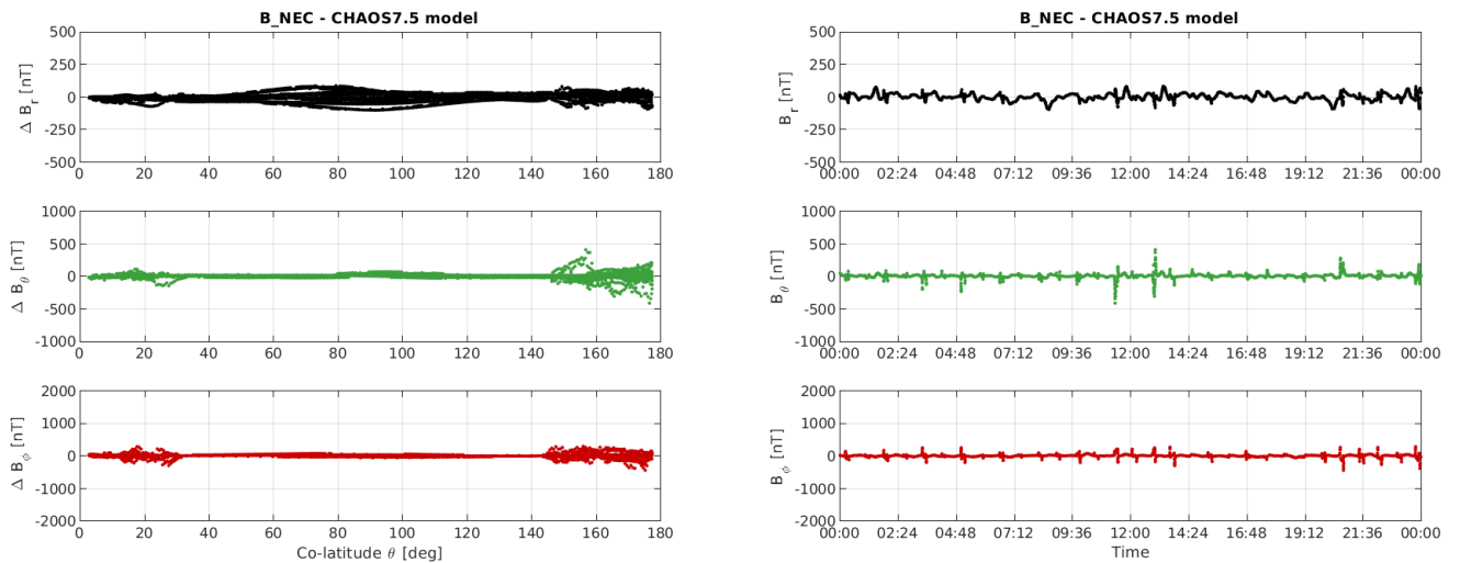
Figure 3-10: S/C A day 08.01: time series of B_{NEC} - B_{Chaos} residuals (right) and B_{NEC} - B_{Chaos} vs colatitude (left).
