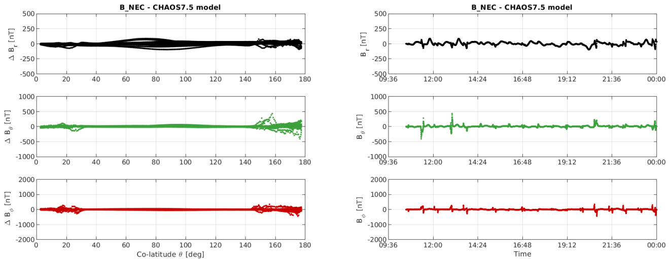
Figure 3-12: S/C C day 08.01: time series of B_{NEC} - B_{Chaos} residuals (right) and B_{NEC} - B_{Chaos} vs colatitude (left)
