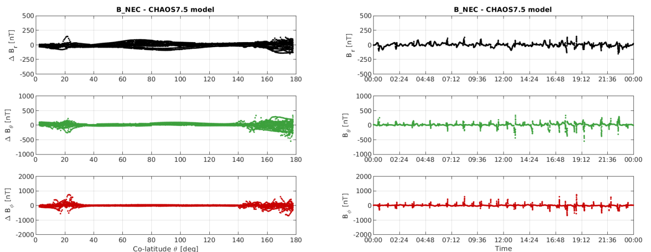
Figure 3-11: S/C B day 01/01: time series of B_{NEC} - B_{Chaos} residuals (right) and B_{NEC} - B_{Chaos} vs colatitude (left).
