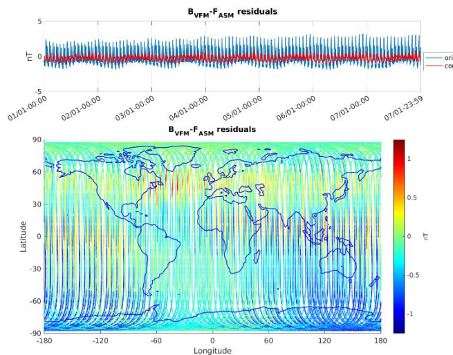
Figure 3-5: ASM-VFM residuals for S/C A, during monitoring period 01/01-07/01. In top figure are plotted: difference between |B_{VFM}| and F_{ASM} (without dB_{Sun} correction) (blue colour), and the residuals with dB_{Sun} corrections (red colour). In bottom figure residuals are presented on the world map.
