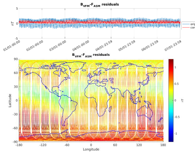
Figure 3-6: ASM-VFM residuals for S/C B, during monitoring period 01/01-07/01. In top figure are plotted: difference between |B_{VFM}| and F_{ASM} (without dB_Sun correction) (blue colour), and the residuals with dB_Sun corrections (red colour). In bottom figure residuals are presented on the world map.
