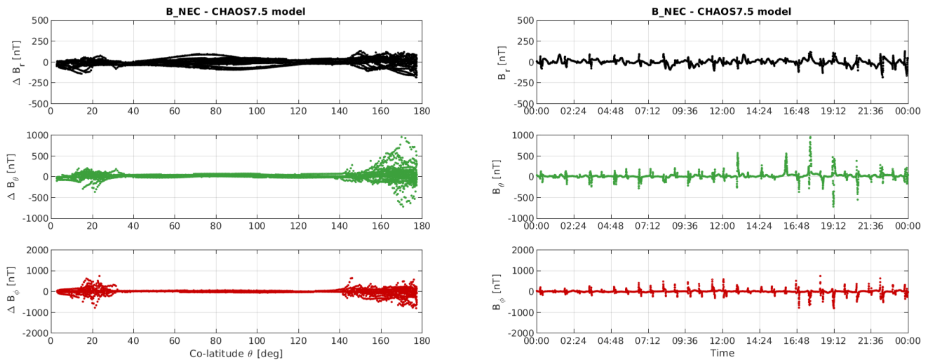
Figure 3-10: S/C A day 01/01: time series of B_{NEC} - B_{Chaos} residuals (right) and B_{NEC} - B_{Chaos} vs colatitude (left).
