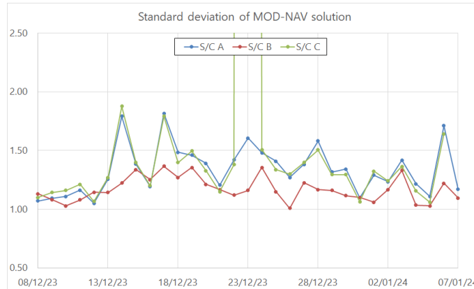
Figure 3-1: Plot of the standard deviation of the difference between MOD and NAV solutions for all satellites. Plot covers last month of operation. Swarm-C suffered an AOCS fallback to Coarse Pointing Mode on 7 th January and due to this analysis are missing for this day.
