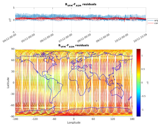
Figure 3-6: ASM-VFM residuals for S/C B, during monitoring period 04/12-10/12. In top figure are plotted: difference between |B_{VFM}| and F_{ASM} (without dB_{Sun} correction) (blue colour), and the residuals with dB_{Sun} corrections (red colour). In bottom figure residuals are presented on the world map.
