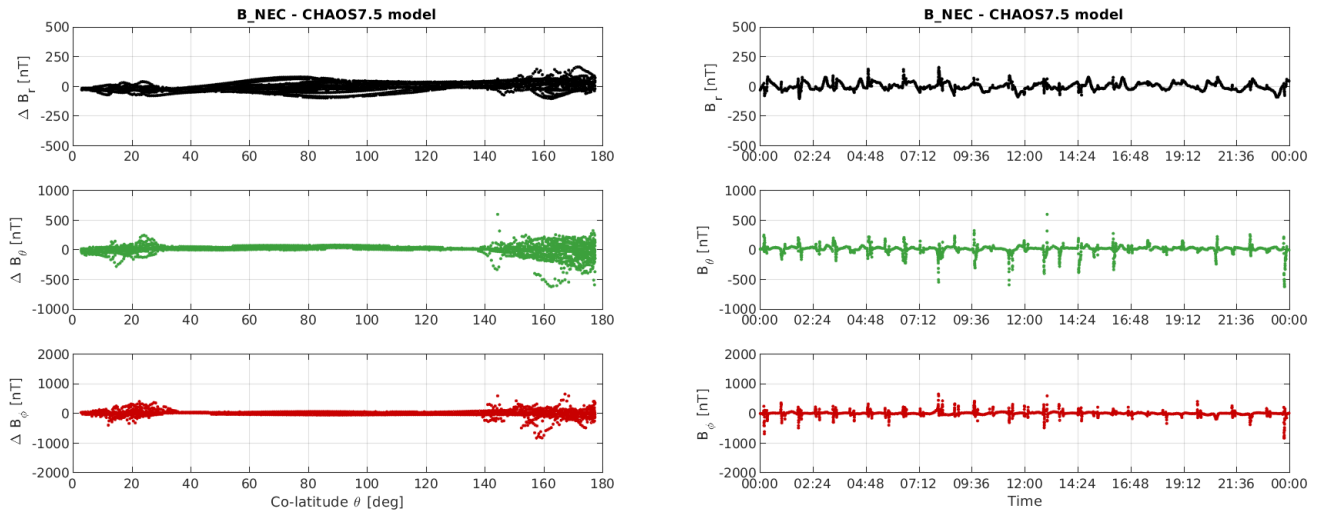
Figure 3-12: S/C C day 04/12: time series of B_{NEC} - B_{Chaos} residuals (right) and B_{NEC} - B_{Chaos} vs colatitude (left)
