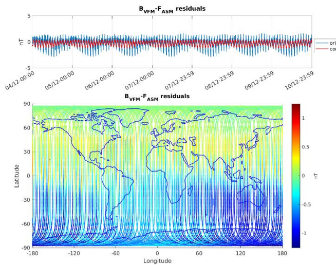
Figure 3-5: ASM-VFM residuals for S/C A, during monitoring period 04/12-10/12. In top figure are plotted: difference between |B_{VFM}| and F_{ASM} (without dB_{Sun} correction) (blue colour), and the residuals with dB_{Sun} corrections (red colour). In bottom figure residuals are presented on the world map.
