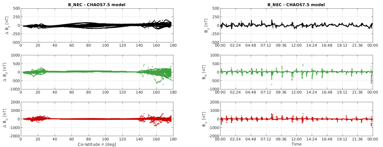
Figure 3-10: S/C A day 04/12: time series of B_{NEC} - B_{Chaos} residuals (right) and B_{NEC} - B_{Chaos} vs colatitude (left).
