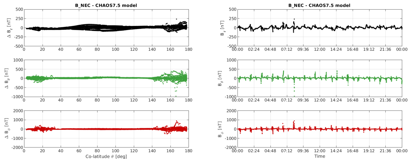
Figure 3-11: S/C B day 04/12: time series of B_{NEC} - B_{Chaos} residuals (right) and B_{NEC} - B_{Chaos} vs colatitude (left).
