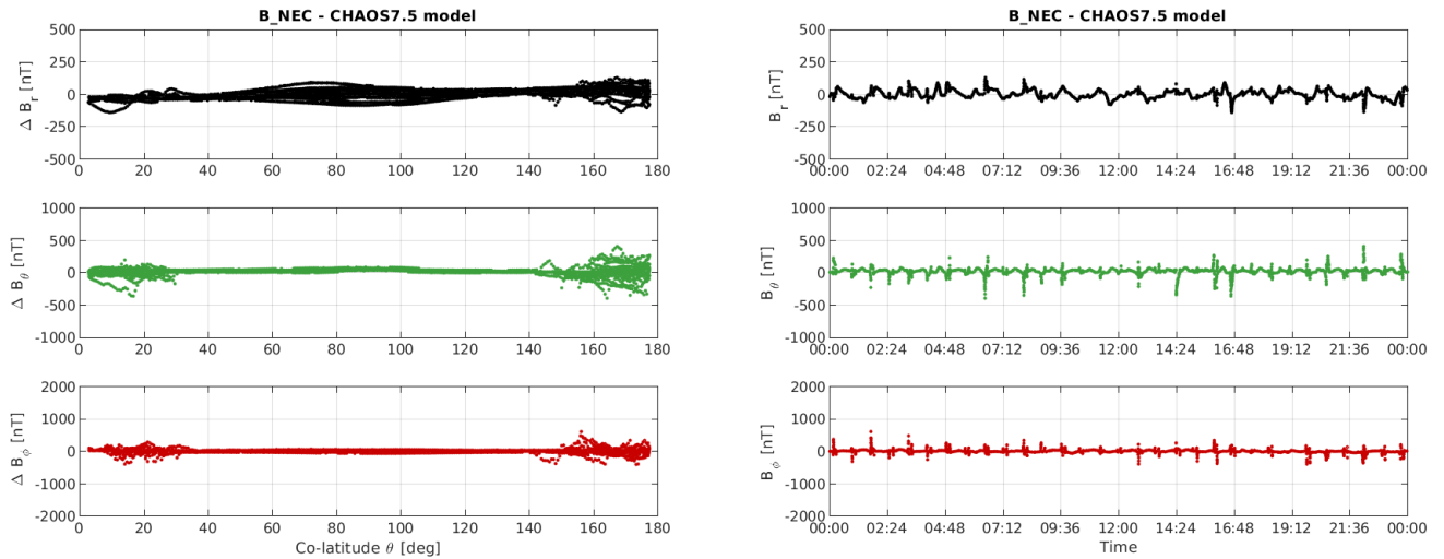
Figure 3-12: S/C C day 27/11: time series of B_{NEC} - B_{Chaos} residuals (right) and B_{NEC} - B_{Chaos} vs colatitude (left)
