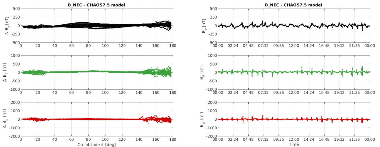
Figure 3-11: S/C B day 27/11: time series of B_{NEC} - B_{Chaos} residuals (right) and B_{NEC} - B_{Chaos} vs colatitude (left).
