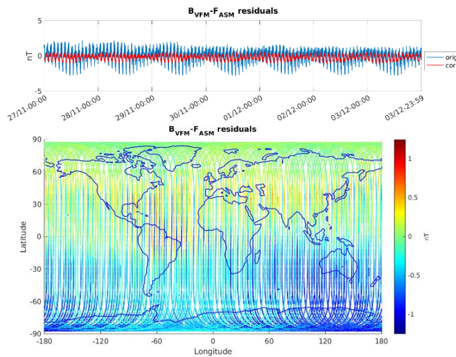
Figure 3-5: ASM-VFM residuals for S/C A, during monitoring period 27/11-03/12. In top figure are plotted: difference between |B_{VFM}| and F_{ASM} (without dB_{Sun} correction) (blue colour), and the residuals with dB_{Sun} corrections (red colour). In bottom figure residuals are presented on the world map.
