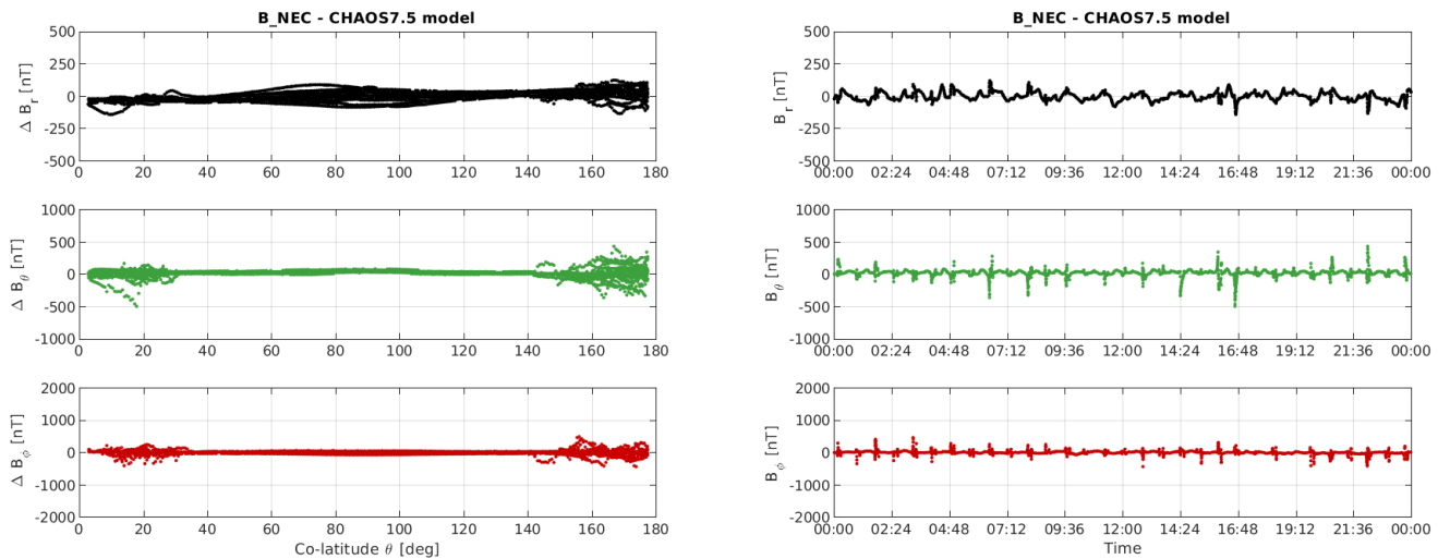
Figure 3-10: S/C A day 27/11: time series of B_{NEC} - B_{Chaos} residuals (right) and B_{NEC} - B_{Chaos} vs colatitude (left).
