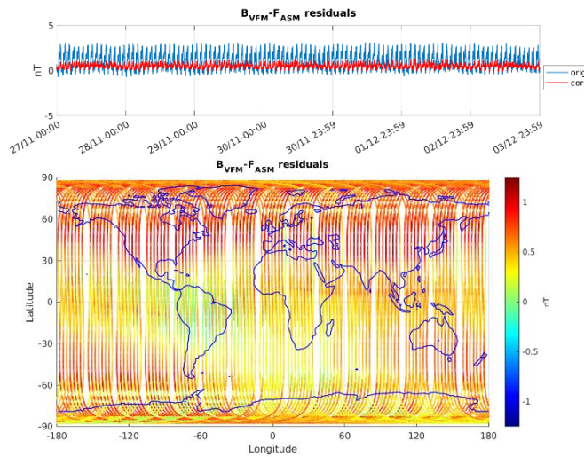
Figure 3-6: ASM-VFM residuals for S/C B, during monitoring period 27/11-03/12. In top figure are plotted: difference between |B_{VFM}| and F_{ASM} (without dB_{Sun} correction) (blue colour), and the residuals with dB_{Sun} corrections (red colour). In bottom figure residuals are presented on the world map.
