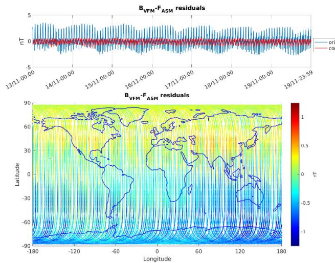
Figure 3-5: ASM-VFM residuals for S/C A, during monitoring period 13/11-19/11. In top figure are plotted: difference between |B_{VFM}| and F_{ASM} (without dB_{Sun} correction) (blue colour), and the residuals with dB_{Sun} corrections (red colour). In bottom figure residuals are presented on the world map.
