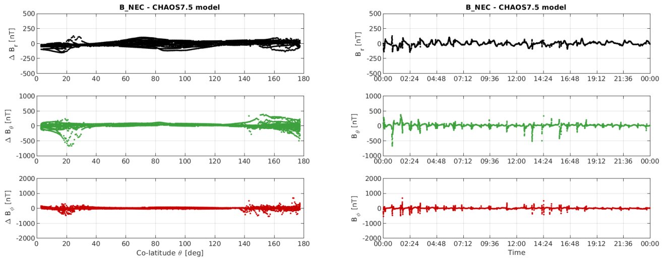
Figure 3-12: S/C C day 13/11: time series of B_{NEC} - B_{Chaos} residuals (right) and B_{NEC} - B_{Chaos} vs colatitude (left)
