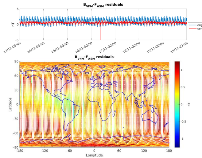
Figure 3-6: ASM-VFM residuals for S/C B, during monitoring period 13/11-19/11. In top figure are plotted: difference between |B_{VFM}| and F_{ASM} (without dB_{Sun} correction) (blue colour), and the residuals with dB_{Sun} corrections (red colour). In bottom figure residuals are presented on the world map.
