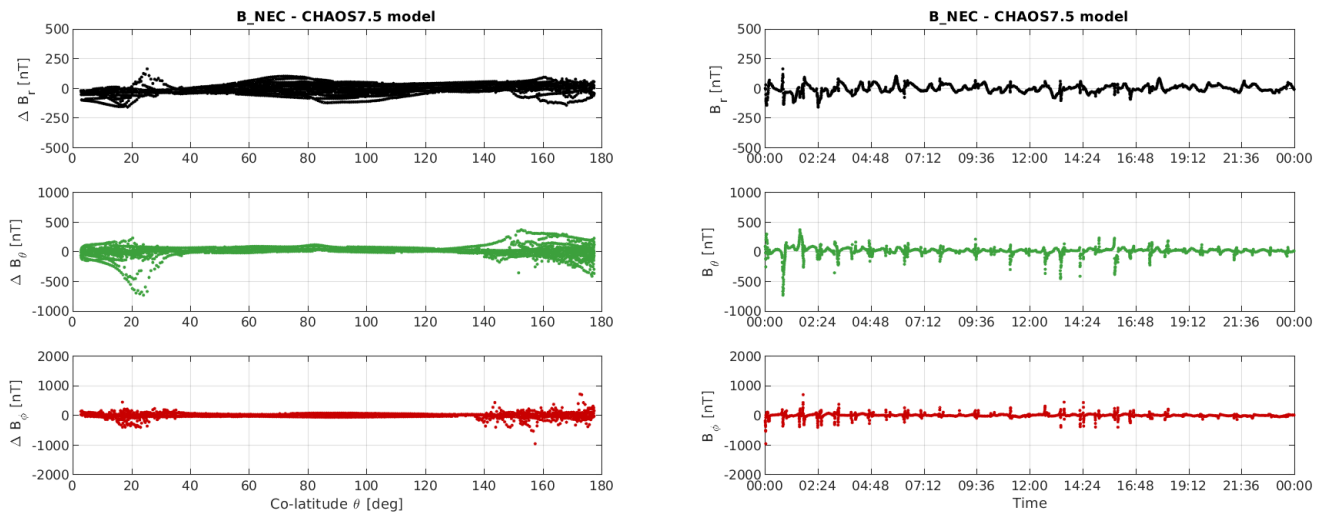
Figure 3-10: S/C A day 13/11: time series of B_{NEC} - B_{Chaos} residuals (right) and B_{NEC} - B_{Chaos} vs colatitude (left).
