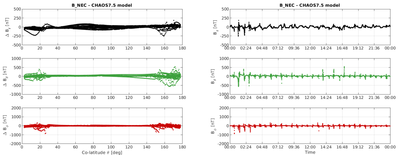
Figure 3-11: S/C B day 13/11: time series of B_{NEC} - B_{Chaos} residuals (right) and B_{NEC} - B_{Chaos} vs colatitude (left).
