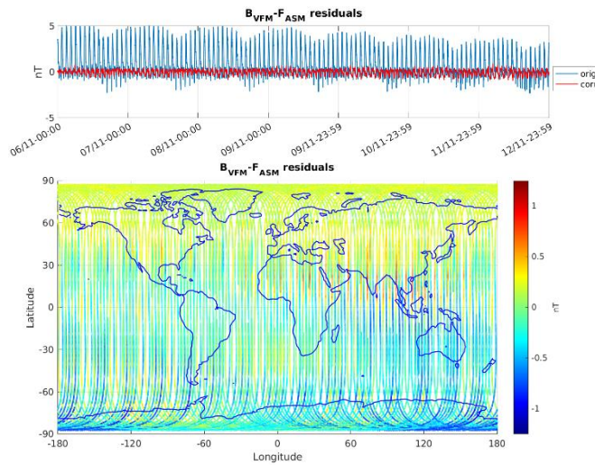
Figure 3-5: ASM-VFM residuals for S/C A, during monitoring period 06/11-12/11. In top figure are plotted: difference between |B_{VFM}| and F_{ASM} (without dB_{Sun} correction) (blue colour), and the residuals with dB_{Sun} corrections (red colour). In bottom figure residuals are presented on the world map.
