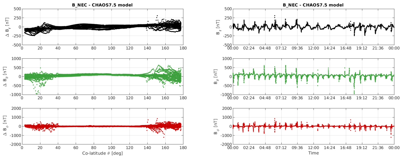
Figure 3-10: S/C A day 06/11: time series of B_{NEC} - B_{Chaos} residuals (right) and B_{NEC} - B_{Chaos} vs colatitude (left).
