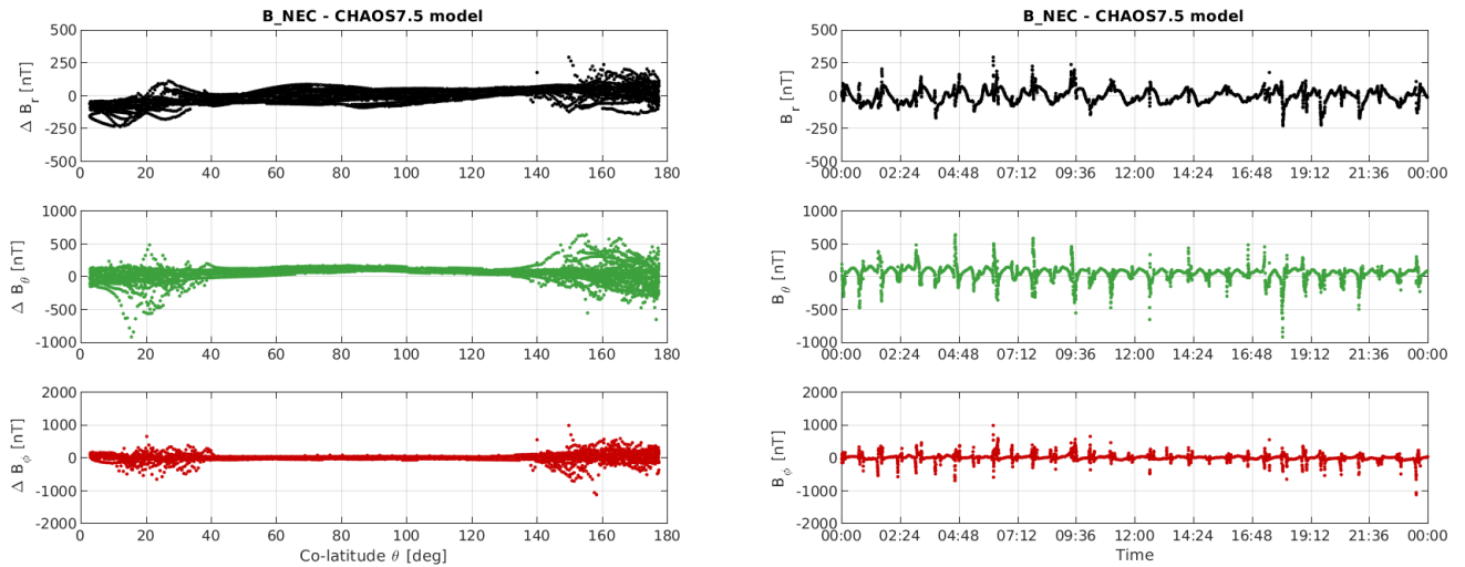
Figure 3-12: S/C C day 06/11: time series of B_{NEC} - B_{Chaos} residuals (right) and B_{NEC} - B_{Chaos} vs colatitude (left)
