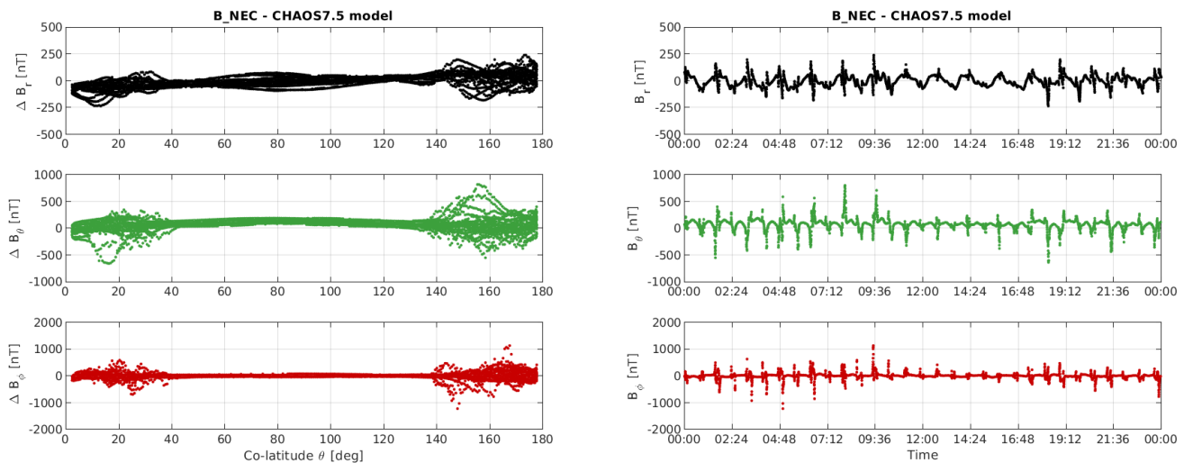
Figure 3-11: S/C B day 06/11: time series of B_{NEC} - B_{Chaos} residuals (right) and B_{NEC} - B_{Chaos} vs colatitude (left).
