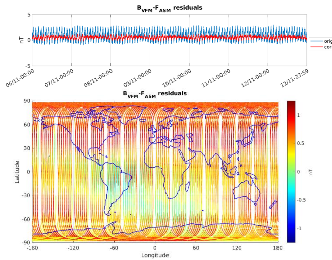
Figure 3-6: ASM-VFM residuals for S/C B, during monitoring period 06/11-12/11. In top figure are plotted: difference between |B_{VFM}| and F_{ASM} (without dB_{Sun} correction) (blue colour), and the residuals with dB_{Sun} corrections (red colour). In bottom figure residuals are presented on the world map.
