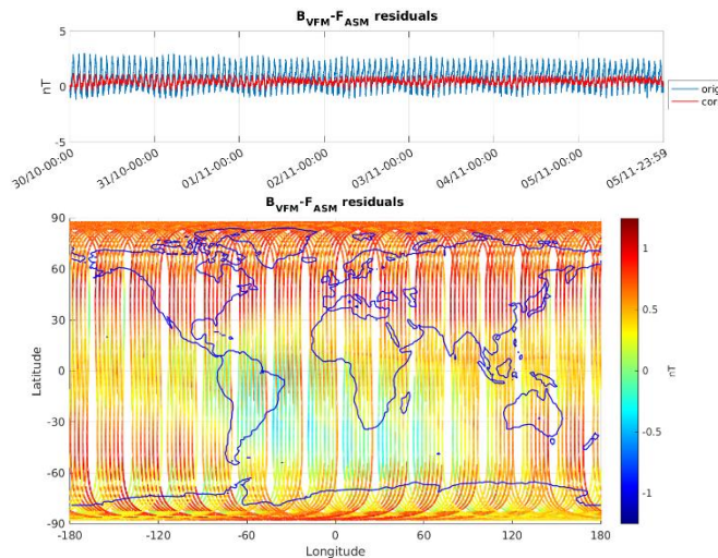
Figure 3-6: ASM-VFM residuals for S/C B, during monitoring period 30/10-05/11. In top figure are plotted: difference between |B_{VFM}| and F_{ASM} (without dB_{Sun} correction) (blue colour), and the residuals with dB_{Sun} corrections (red colour). In bottom figure residuals are presented on the world map.
