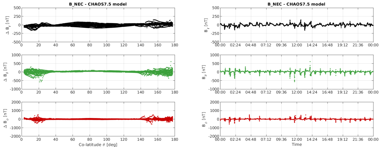
Figure 3-12: S/C C day 30/10: time series of B_{NEC} - B_{Chaos} residuals (right) and B_{NEC} - B_{Chaos} vs colatitude (left)
