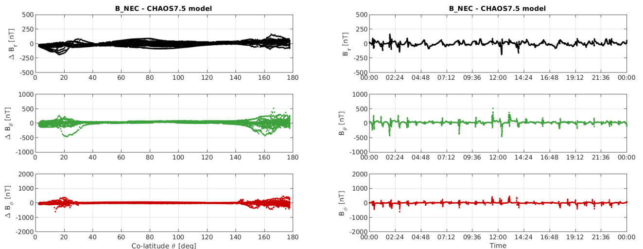
Figure 3-11: S/C B day 30/10: time series of B_{NEC} - B_{Chaos} residuals (right) and B_{NEC} - B_{Chaos} vs colatitude (left).
