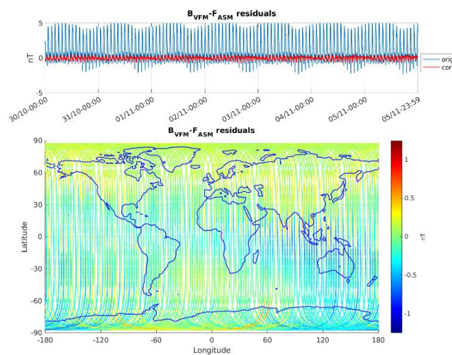
Figure 3-5: ASM-VFM residuals for S/C A, during monitoring period 30/10-05/11. In top figure are plotted: difference between |B_{VFM}| and F_{ASM} (without dB_Sun correction) (blue colour), and the residuals with dB_Sun corrections (red colour). In bottom figure residuals are presented on the world map.
