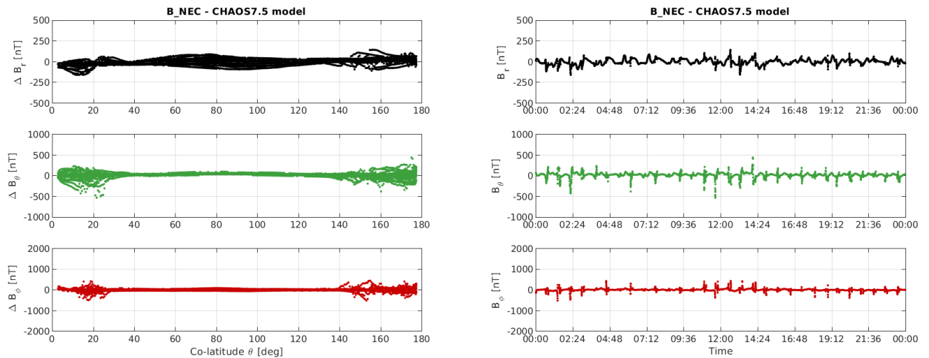
Figure 3-10: S/C A day 30/10: time series of B_{NEC} - B_{Chaos} residuals (right) and B_{NEC} - B_{Chaos} vs colatitude (left).
