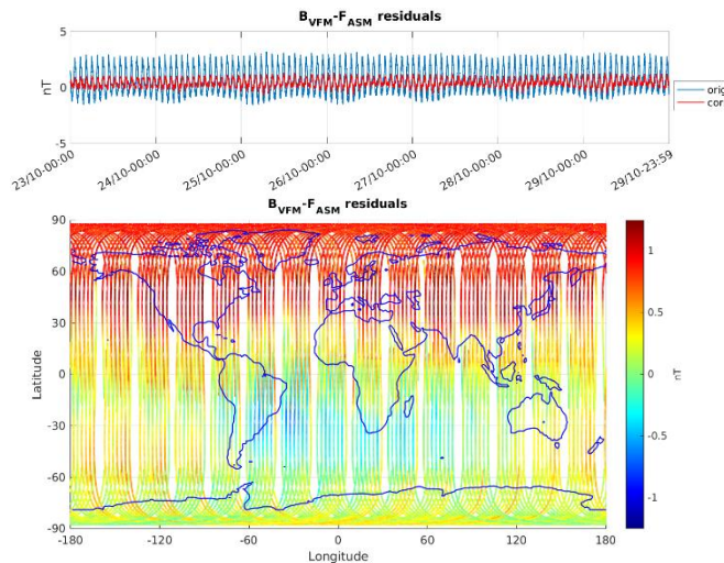
Figure 3-6: ASM-VFM residuals for S/C B, during monitoring period 23/10-29/10. In top figure are plotted: difference between |B_{VFM}| and F_{ASM} (without dB_{Sun} correction) (blue colour), and the residuals with dB_{Sun} corrections (red colour). In bottom figure residuals are presented on the world map.
