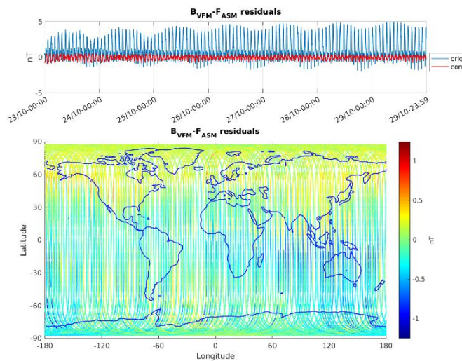
Figure 3-5: ASM-VFM residuals for S/C A, during monitoring period 23/10-29/10. In top figure are plotted: difference between |B_{VFM}| and F_{ASM} (without dB_{Sun} correction) (blue colour), and the residuals with dB_{Sun} corrections (red colour). In bottom figure residuals are presented on the world map.
