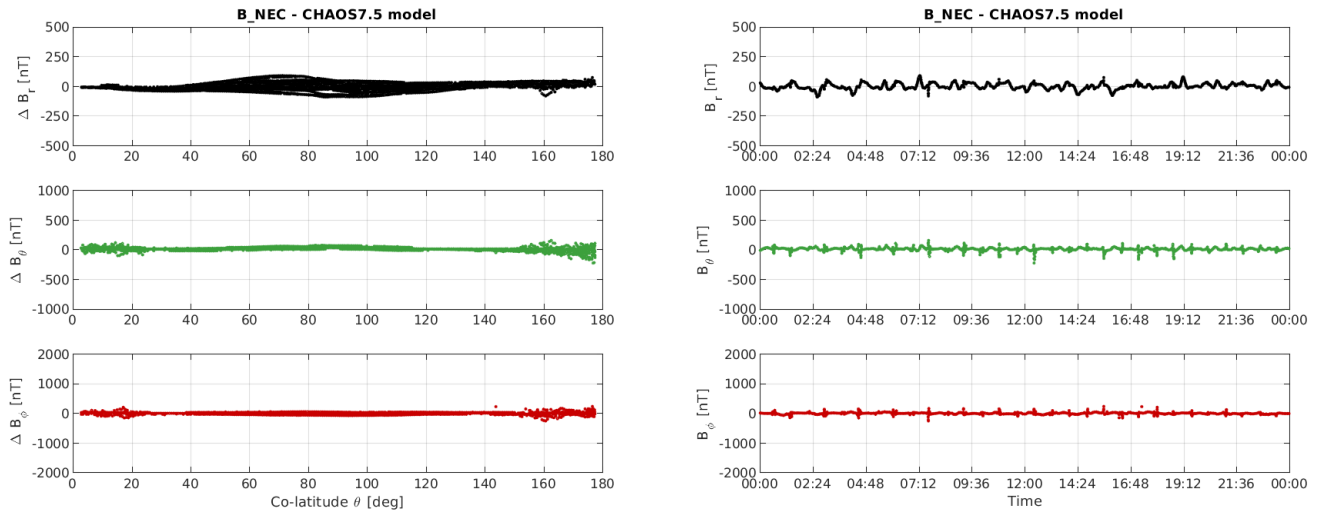
Figure 3-12: S/C C day 23/10: time series of B_{NEC} - B_{Chaos} residuals (right) and B_{NEC} - B_{Chaos} vs colatitude (left)
