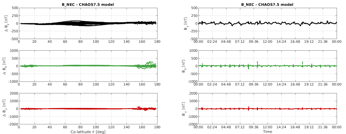
Figure 3-11: S/C B day 23/10: time series of B_{NEC} - B_{Chaos} residuals (right) and B_{NEC} - B_{Chaos} vs colatitude (left).
