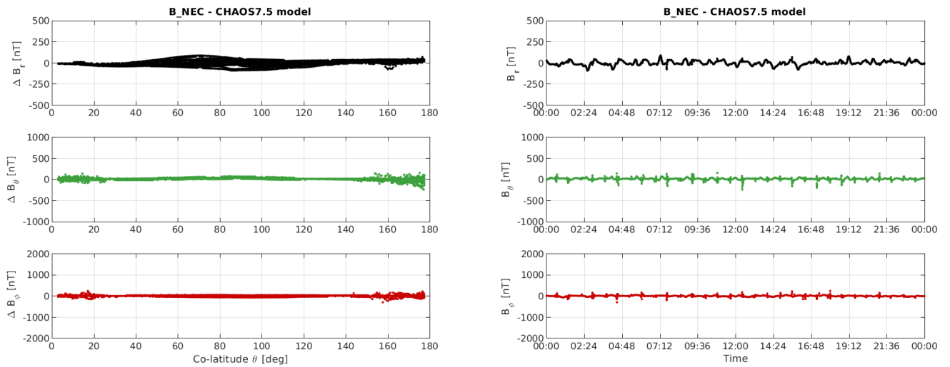
Figure 3-10: S/C A day 23/10: time series of B_{NEC} - B_{Chaos} residuals (right) and B_{NEC} - B_{Chaos} vs colatitude (left).
