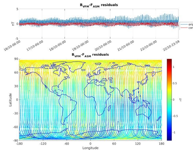
Figure 3-5: ASM-VFM residuals for S/C A, during monitoring period 16/10-22/10. In top figure are plotted: difference between |B_{VFM}| and F_{ASM} (without dB_{Sun} correction) (blue colour), and the residuals with dB_{Sun} corrections (red colour). In bottom figure residuals are presented on the world map.
