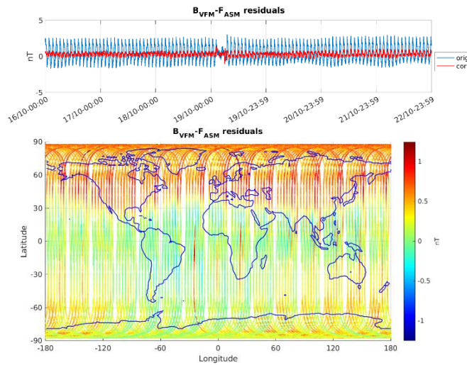
Figure 3-6: ASM-VFM residuals for S/C B, during monitoring period 16/10-22/10. In top figure are plotted: difference between |B_{VFM}| and F_{ASM} (without dB_{Sun} correction) (blue colour), and the residuals with dB_{Sun} corrections (red colour). In bottom figure residuals are presented on the world map.
