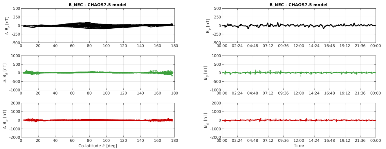
Figure 3-10: S/C A day 16/10: time series of B_{NEC} - B_{Chaos} residuals (right) and B_{NEC} - B_{Chaos} vs colatitude (left).
