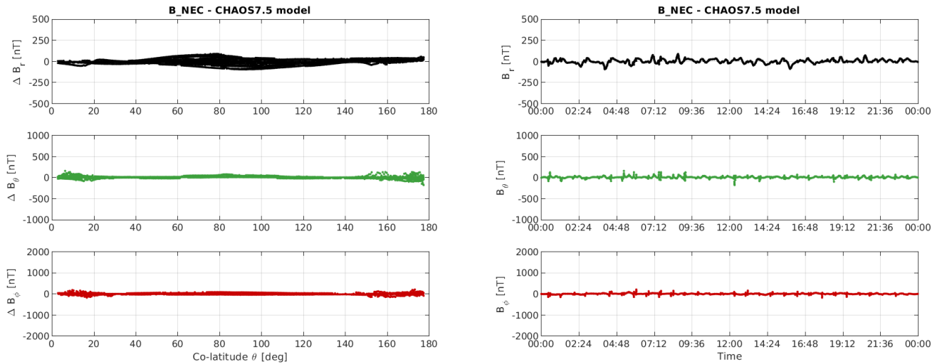
Figure 3-12: S/C C day 16/10: time series of B_{NEC} - B_{Chaos} residuals (right) and B_{NEC} - B_{Chaos} vs colatitude (left)
