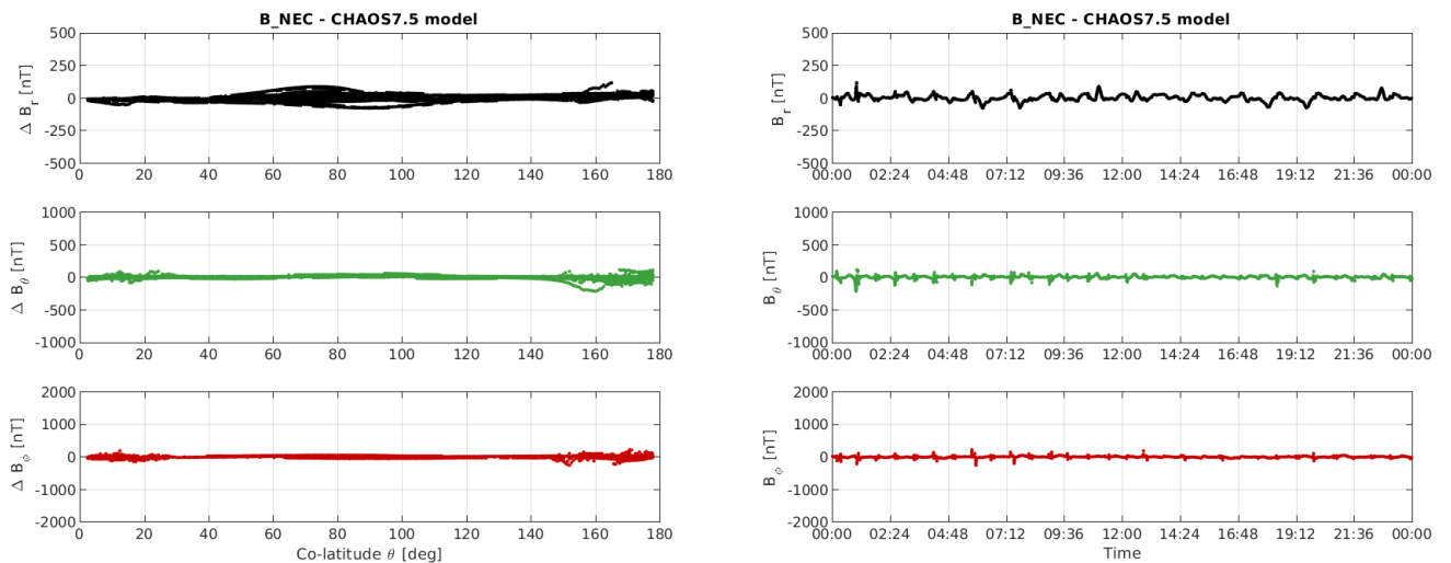
Figure 3-11: S/C B day 16/10: time series of B_{NEC} - B_{Chaos} residuals (right) and B_{NEC} - B_{Chaos} vs colatitude (left).
