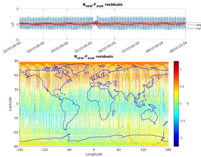
Figure 3-6: ASM-VFM residuals for S/C B, during monitoring period 02/10-08/10. In top figure are plotted: difference between |B_{VFM}| and F_{ASM} (without dB_Sun correction) (blue colour), and the residuals with dB_Sun corrections (red colour). In bottom figure residuals are presented on the world map.
