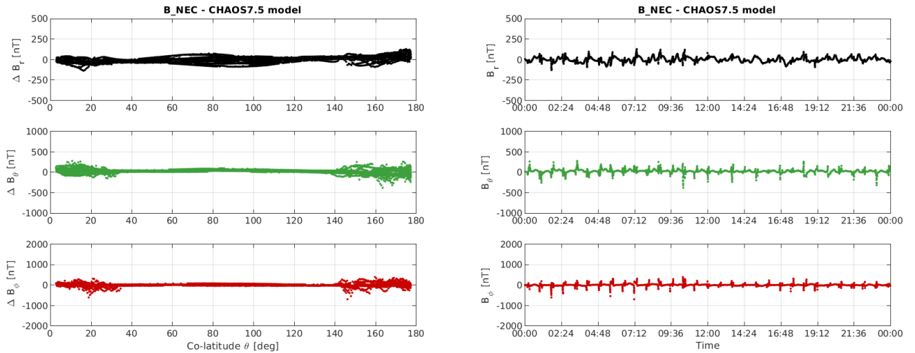
Figure 3-12: S/C C day 02/10: time series of B_{NEC} - B_{Chaos} residuals (right) and B_{NEC} - B_{Chaos} vs colatitude (left)
