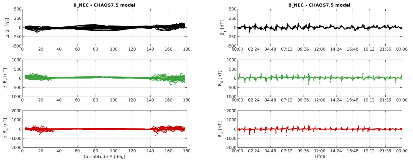
Figure 3-10: S/C A day 02/10: time series of B_{NEC} - B_{Chaos} residuals (right) and B_{NEC} - B_{Chaos} vs colatitude (left).
