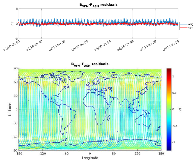
Figure 3-5: ASM-VFM residuals for S/C A, during monitoring period 02/10-08/10. In top figure are plotted: difference between |B_{VFM}| and F_{ASM} (without dB_{Sun} correction) (blue colour), and the residuals with dB_{Sun} corrections (red colour). In bottom figure residuals are presented on the world map.
