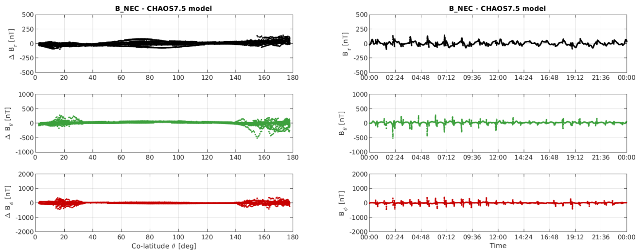
Figure 3-11: S/C B day 02/10: time series of B_{NEC} - B_{Chaos} residuals (right) and B_{NEC} - B_{Chaos} vs colatitude (left).
