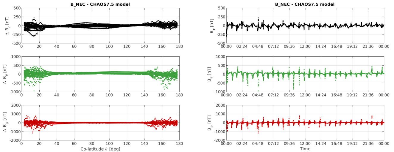
Figure 3-12: S/C C day 25/09: time series of B_{NEC} - B_{Chaos} residuals (right) and B_{NEC} - B_{Chaos} vs colatitude (left)
