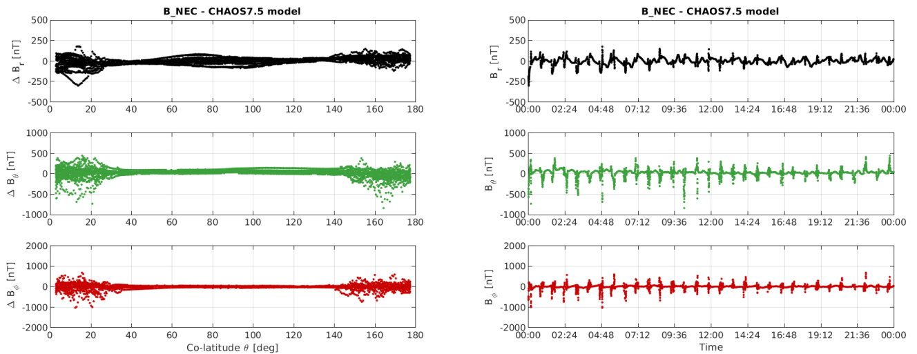
Figure 3-10: S/C A day 25/09: time series of B_{NEC} - B_{Chaos} residuals (right) and B_{NEC} - B_{Chaos} vs colatitude (left).
