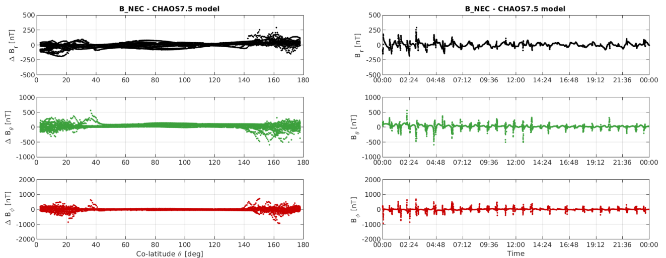
Figure 3-11: S/C B day 25/09: time series of B_{NEC} - B_{Chaos} residuals (right) and B_{NEC} - B_{Chaos} vs colatitude (left).
