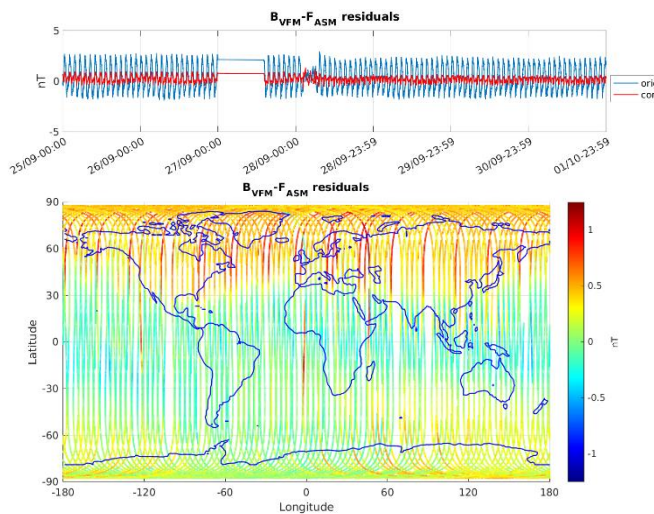
Figure 3-6: ASM-VFM residuals for S/C B, during monitoring period 25/09-01/10. In top figure are plotted: difference between |B_{VFM}| and F_{ASM} (without dB_{Sun} correction) (blue colour), and the residuals with dB_{Sun} corrections (red colour). In bottom figure residuals are presented on the world map.
