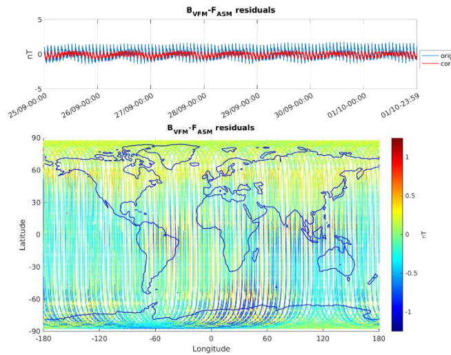
Figure 3-5: ASM-VFM residuals for S/C A, during monitoring period 25/09-01/10. In top figure are plotted: difference between |B_{VFM}| and F_{ASM} (without dB_{Sun} correction) (blue colour), and the residuals with dB_{Sun} corrections (red colour). In bottom figure residuals are presented on the world map.
