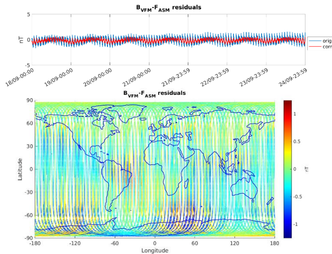
Figure 3-5: ASM-VFM residuals for S/C A, during monitoring period 18/09-24/09. In top figure are plotted: difference between |B_{VFM}| and F_{ASM} (without dB_{Sun} correction) (blue colour), and the residuals with dB_{Sun} corrections (red colour). In bottom figure residuals are presented on the world map.
