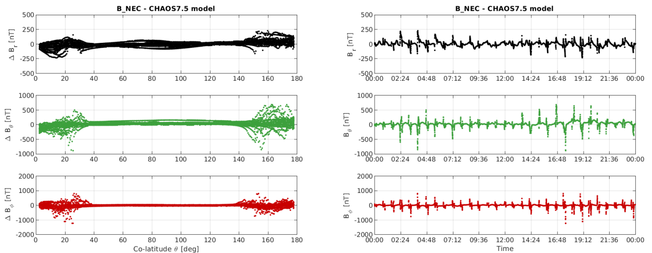
Figure 3-11: S/C B day 18/09: time series of B_{NEC} - B_{Chaos} residuals (right) and B_{NEC} - B_{Chaos} vs colatitude (left).
