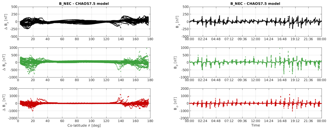
Figure 3-12: S/C C day 18/09: time series of B_{NEC} - B_{Chaos} residuals (right) and B_{NEC} - B_{Chaos} vs colatitude (left)
