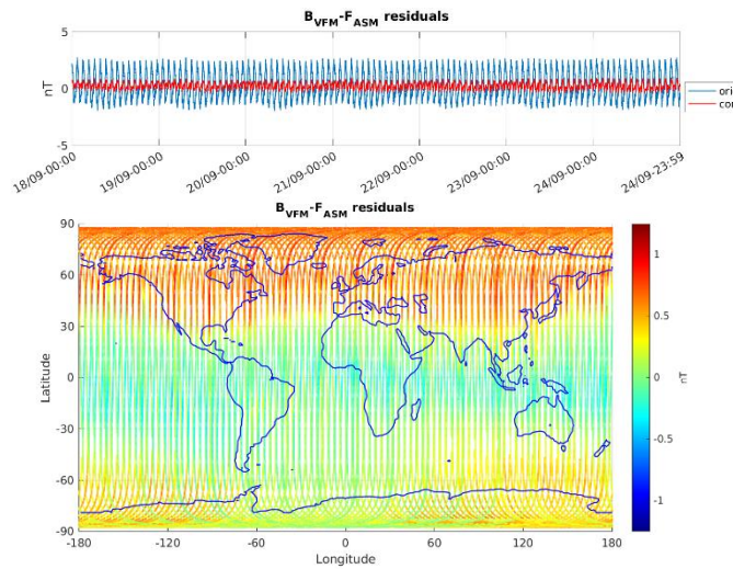
Figure 3-6: ASM-VFM residuals for S/C B, during monitoring period 18/09-24/09. In top figure are plotted: difference between |B_{VFM}| and F_{ASM} (without dB_{Sun} correction) (blue colour), and the residuals with dB_{Sun} corrections (red colour). In bottom figure residuals are presented on the world map.
