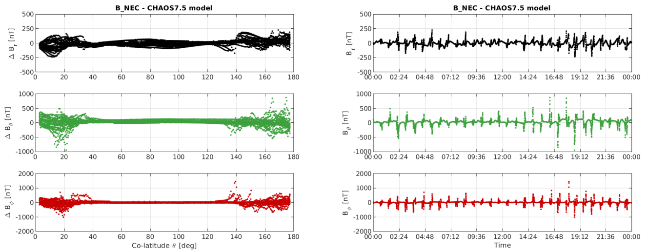
Figure 3-10: S/C A day 18/09: time series of B_{NEC} - B_{Chaos} residuals (right) and B_{NEC} - B_{Chaos} vs colatitude (left).
