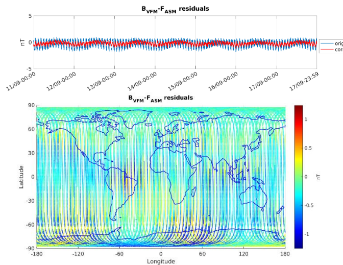
Figure 3-5: ASM-VFM residuals for S/C A, during monitoring period 11/09-17/09. In top figure are plotted: difference between |B_{VFM}| and F_{ASM} (without dB_{Sun} correction) (blue colour), and the residuals with dB_{Sun} corrections (red colour). In bottom figure residuals are presented on the world map.
