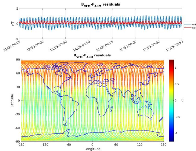
Figure 3-6: ASM-VFM residuals for S/C B, during monitoring period 11/09-17/09. In top figure are plotted: difference between |B_{VFM}| and F_{ASM} (without dB Sun correction) (blue colour), and the residuals with dB Sun corrections (red colour). In bottom figure residuals are presented on the world map.
