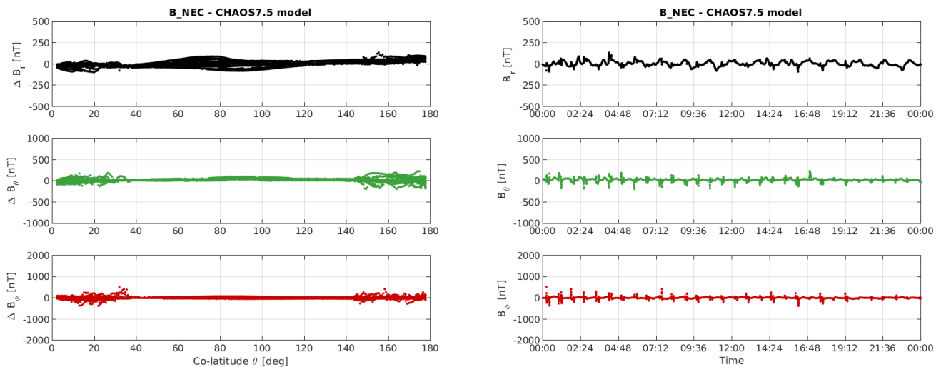
Figure 3-11: S/C B day 04/09: time series of B_{NEC} - B_{Chaos} residuals (right) and B_{NEC} - B_{Chaos} vs colatitude (left).
