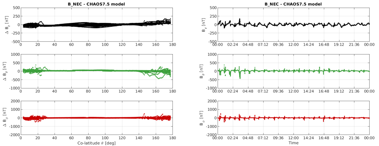
Figure 3-12: S/C C day 04/09: time series of B_{NEC} - B_{Chaos} residuals (right) and B_{NEC} - B_{Chaos} vs colatitude (left)
