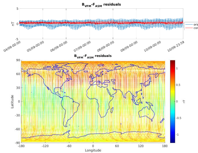
Figure 3-6: ASM-VFM residuals for S/C B, during monitoring period 04/09-10/09. In top figure are plotted: difference between |B_{VFM}| and F_{ASM} (without dB_Sun correction) (blue colour), and the residuals with dB_Sun corrections (red colour). In bottom figure residuals are presented on the world map.
