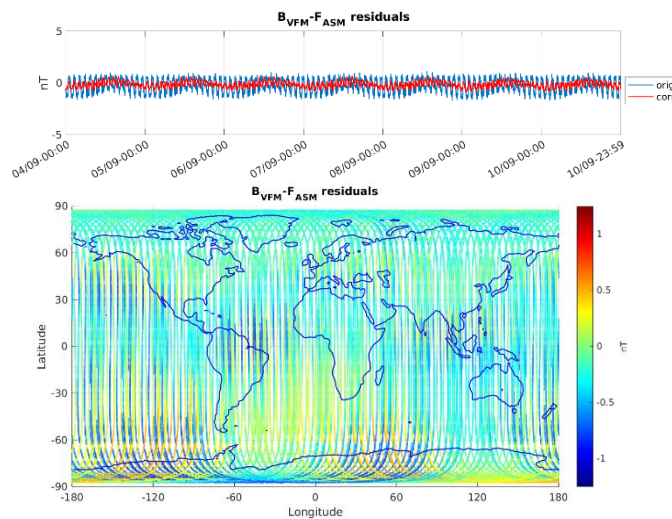
Figure 3-5: ASM-VFM residuals for S/C A, during monitoring period 04/09-10/09. In top figure are plotted: difference between |B_{VFM}| and F_{ASM} (without dB_{Sun} correction) (blue colour), and the residuals with dB_{Sun} corrections (red colour). In bottom figure residuals are presented on the world map.
