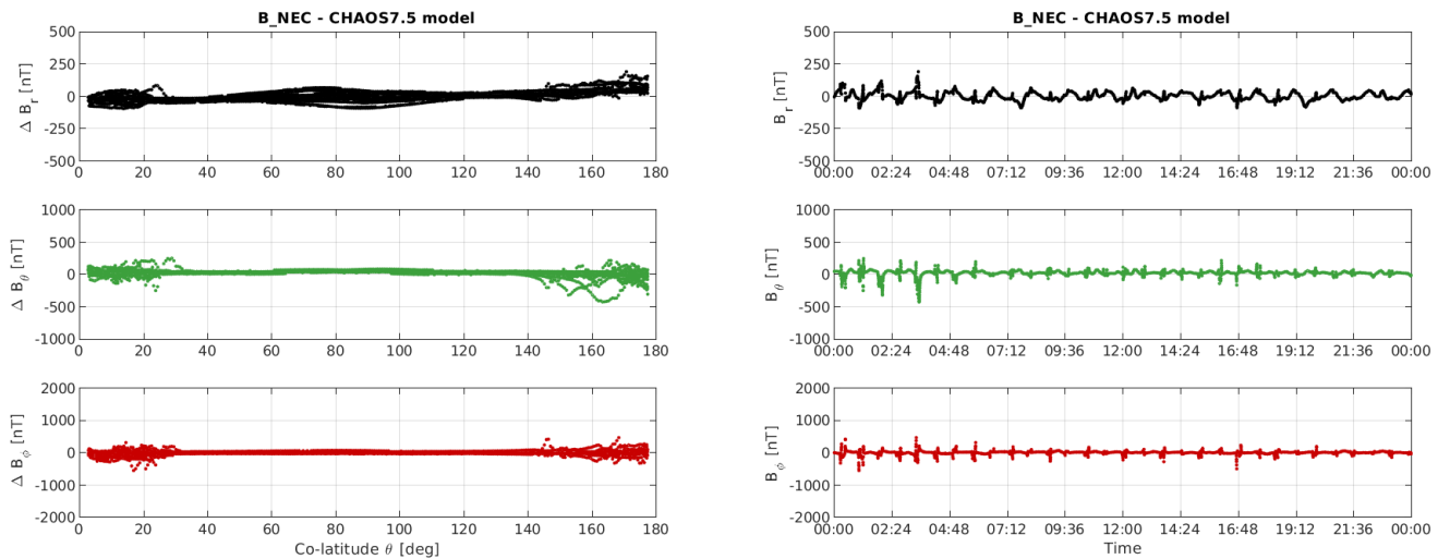
Figure 3-10: S/C A day 04/09: time series of B_{NEC} - B_{Chaos} residuals (right) and B_{NEC} - B_{Chaos} vs colatitude (left).
