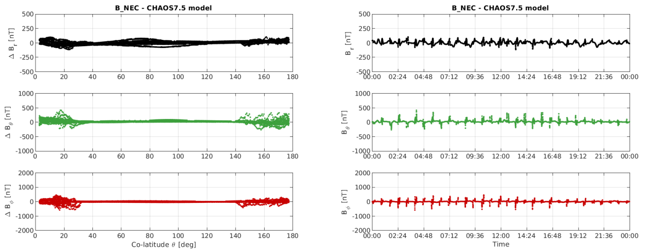
Figure 3-10: S/C A day 28/08: time series of B_{NEC} - B_{Chaos} residuals (right) and B_{NEC} - B_{Chaos} vs colatitude (left).
