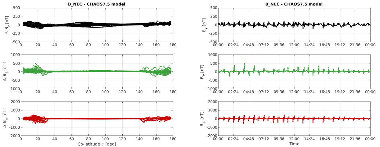
Figure 3-12: S/C C day 28/08: time series of B_{NEC} - B_{Chaos} residuals (right) and B_{NEC} - B_{Chaos} vs colatitude (left)
