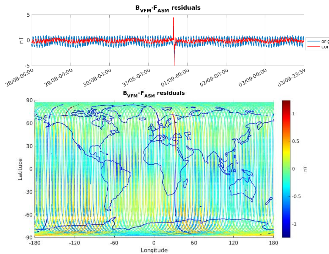
Figure 3-5: ASM-VFM residuals for S/C A, during monitoring period 28/08-03/09. In top figure are plotted: difference between |B_{VFM}| and F_{ASM} (without dB_{Sun} correction) (blue colour), and the residuals with dB_{Sun} corrections (red colour). In bottom figure residuals are presented on the world map.
