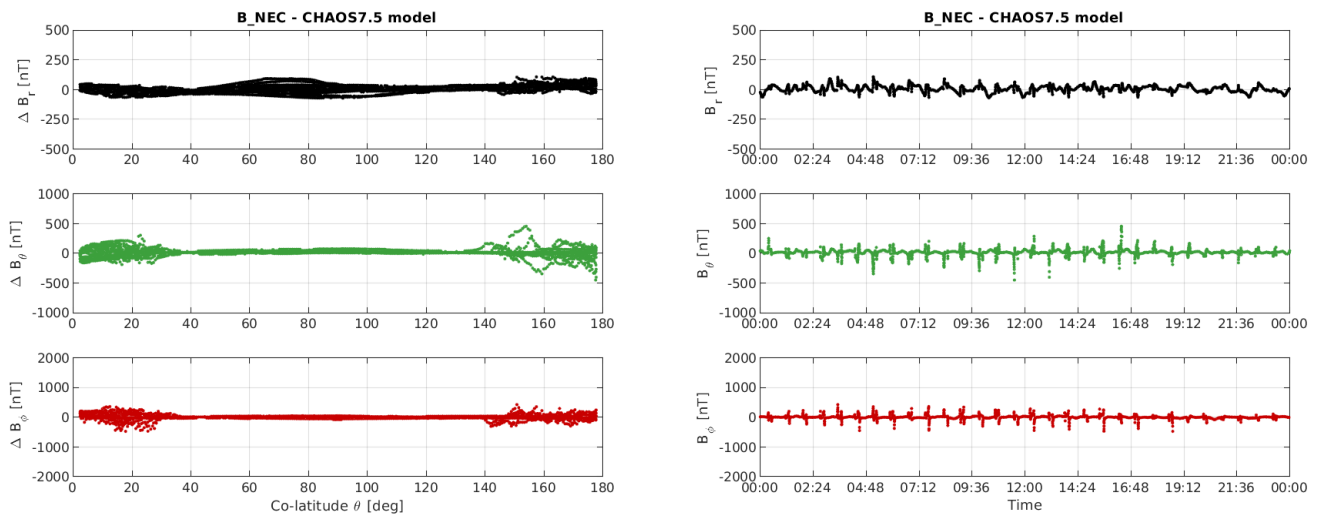
Figure 3-11: S/C B day 28/08: time series of B_{NEC} - B_{Chaos} residuals (right) and B_{NEC} - B_{Chaos} vs colatitude (left).
