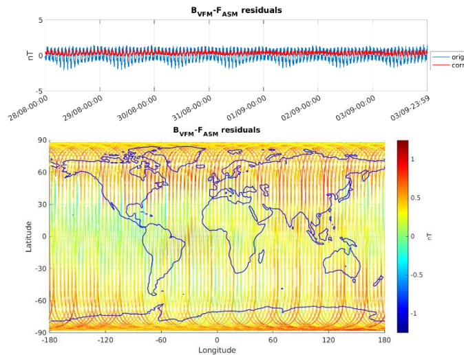
Figure 3-6: ASM-VFM residuals for S/C B, during monitoring period 28/08-03/09. In top figure are plotted: difference between |B_{VFM}| and F_{ASM} (without dB_Sun correction) (blue colour), and the residuals with dB_Sun corrections (red colour). In bottom figure residuals are presented on the world map.
