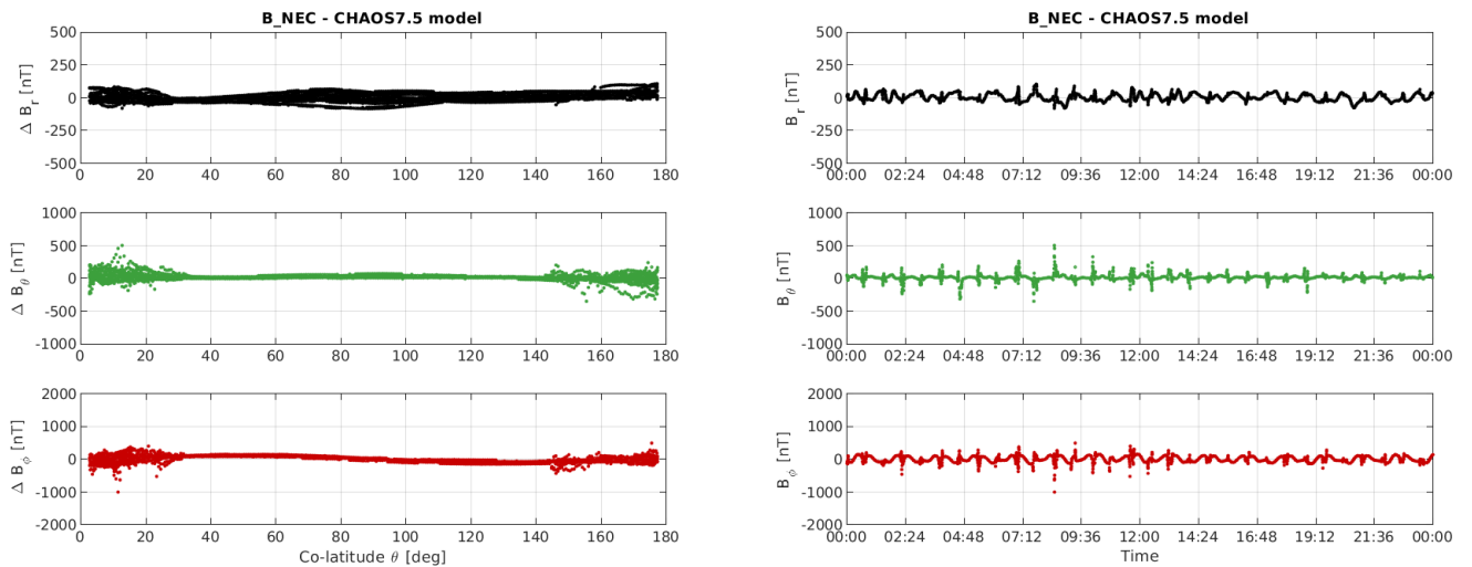
Figure 3-10: S/C A day 21/08: time series of B_{NEC} - B_{Chaos} residuals (right) and B_{NEC} - B_{Chaos} vs colatitude (left).
