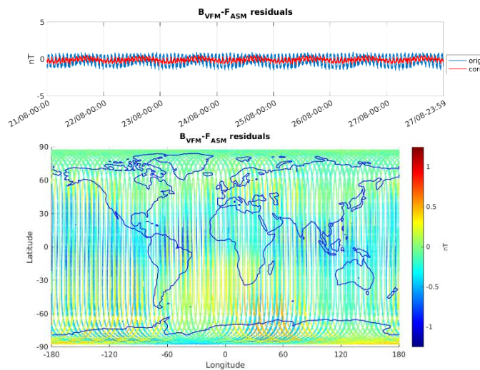
Figure 3-5: ASM-VFM residuals for S/C A, during monitoring period 21/08-27/08. In top figure are plotted: difference between |B_{VFM}| and F_{ASM} (without dB_{Sun} correction) (blue colour), and the residuals with dB_{Sun} corrections (red colour). In bottom figure residuals are presented on the world map.
