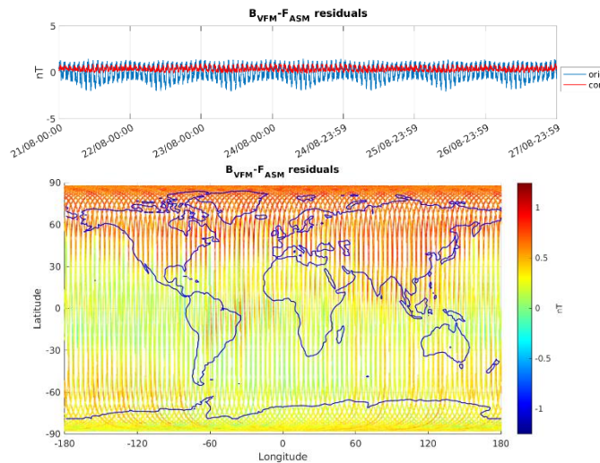
Figure 3-6: ASM-VFM residuals for S/C B, during monitoring period 21/08-27/08. In top figure are plotted: difference between |B_{VFM}| and F_{ASM} (without dB_{Sun} correction) (blue colour), and the residuals with dB_{Sun} corrections (red colour). In bottom figure residuals are presented on the world map.
