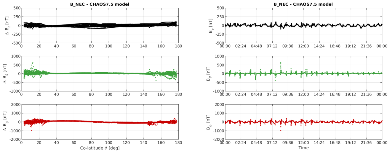
Figure 3-12: S/C C day 21/08: time series of B_{NEC} - B_{Chaos} residuals (right) and B_{NEC} - B_{Chaos} vs colatitude (left)
