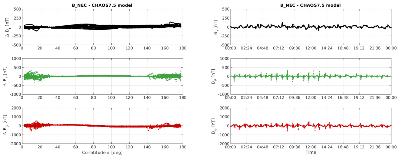
Figure 3-11: S/C B day 21/08: time series of B_{NEC} - B_{Chaos} residuals (right) and B_{NEC} - B_{Chaos} vs colatitude (left).
