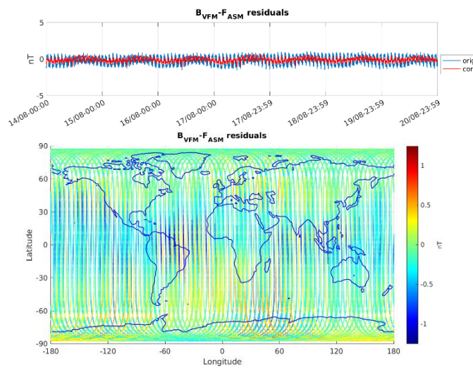
Figure 3-5: ASM-VFM residuals for S/C A, during monitoring period 14/08-20/08. In top figure are plotted: difference between |B_{VFM}| and F_{ASM} (without dB_{Sun} correction) (blue colour), and the residuals with dB_{Sun} corrections (red colour). In bottom figure residuals are presented on the world map.
