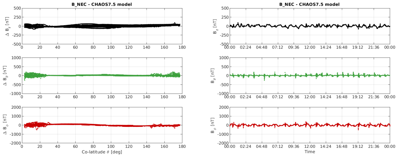
Figure 3-12: S/C C day 14/08: time series of B_{NEC} - B_{Chaos} residuals (right) and B_{NEC} - B_{Chaos} vs colatitude (left)
