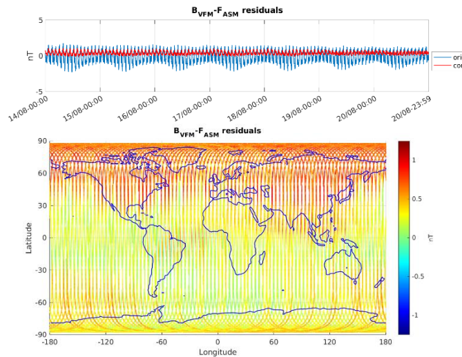
Figure 3-6: ASM-VFM residuals for S/C B, during monitoring period 14/08-20/08. In top figure are plotted: difference between |B_{VFM}| and F_{ASM} (without dB_Sun correction) (blue colour), and the residuals with dB_Sun corrections (red colour). In bottom figure residuals are presented on the world map.
