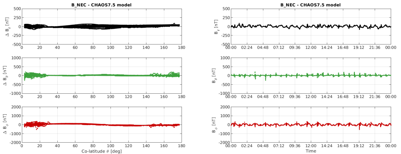
Figure 3-10: S/C A day 14/08: time series of B_{NEC} - B_{Chaos} residuals (right) and B_{NEC} - B_{Chaos} vs colatitude (left).
