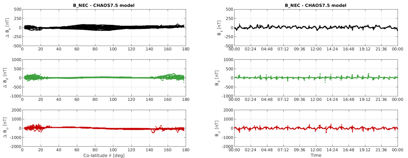
Figure 3-11: S/C B day 14/08: time series of B_{NEC} - B_{Chaos} residuals (right) and B_{NEC} - B_{Chaos} vs colatitude (left).
