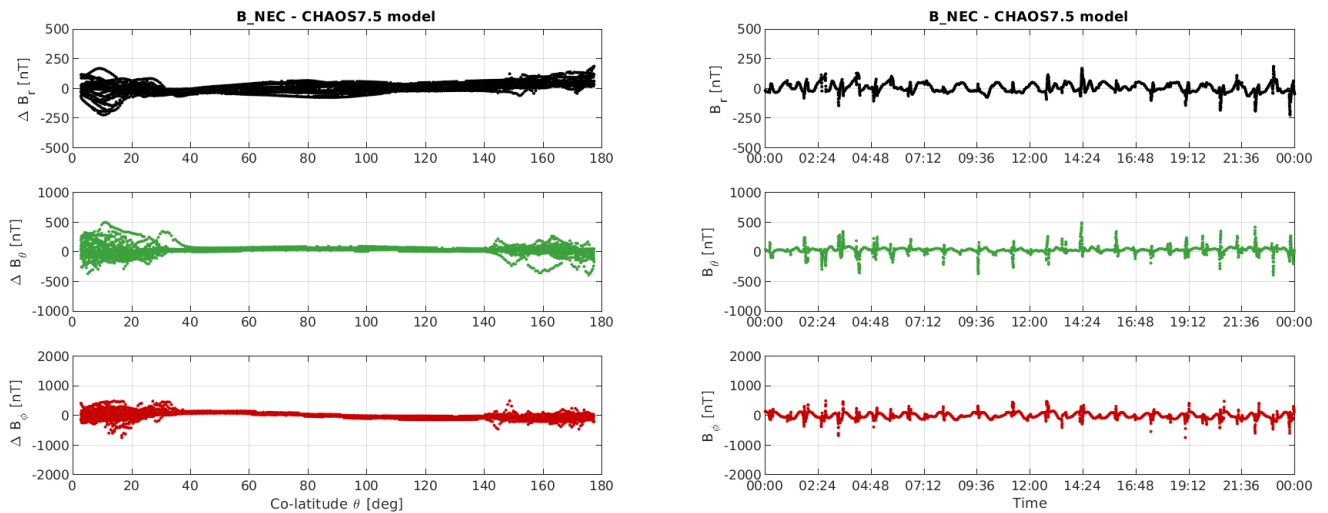
Figure 3-10: S/C A day 07/08: time series of B_{NEC} - B_{Chaos} residuals (right) and B_{NEC} - B_{Chaos} vs colatitude (left).
