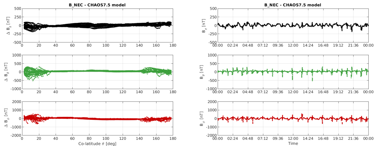
Figure 3-11: S/C B day 07/08: time series of B_{NEC} - B_{Chaos} residuals (right) and B_{NEC} - B_{Chaos} vs colatitude (left).
