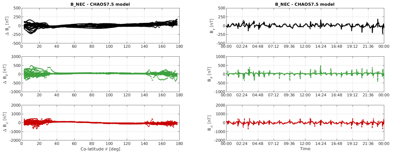
Figure 3-12: S/C C day 07/08: time series of B_{NEC} - B_{Chaos} residuals (right) and B_{NEC} - B_{Chaos} vs colatitude (left)
