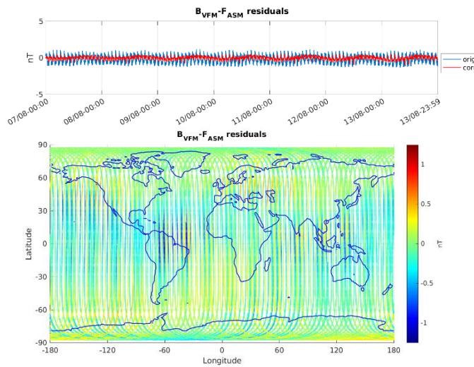
Figure 3-5: ASM-VFM residuals for S/C A, during monitoring period 07/08-13/08. In top figure are plotted: difference between |B_{VFM}| and F_{ASM} (without dB_{Sun} correction) (blue colour), and the residuals with dB_{Sun} corrections (red colour). In bottom figure residuals are presented on the world map.
