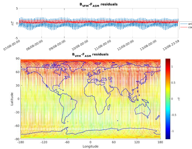
Figure 3-6: ASM-VFM residuals for S/C B, during monitoring period 07/08-13/08. In top figure are plotted: difference between |B_{VFM}| and F_{ASM} (without dB_Sun correction) (blue colour), and the residuals with dB_Sun corrections (red colour). In bottom figure residuals are presented on the world map.
