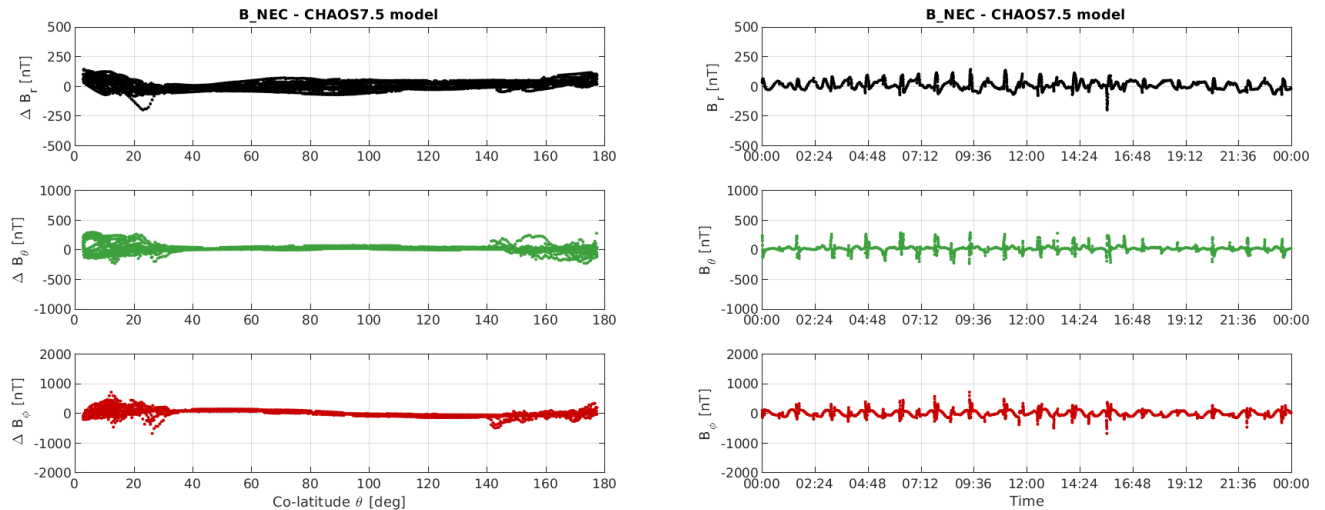
Figure 3-12: S/C C day 31/07: time series of B_{NEC} - B_{Chaos} residuals (right) and B_{NEC} - B_{Chaos} vs colatitude (left)
