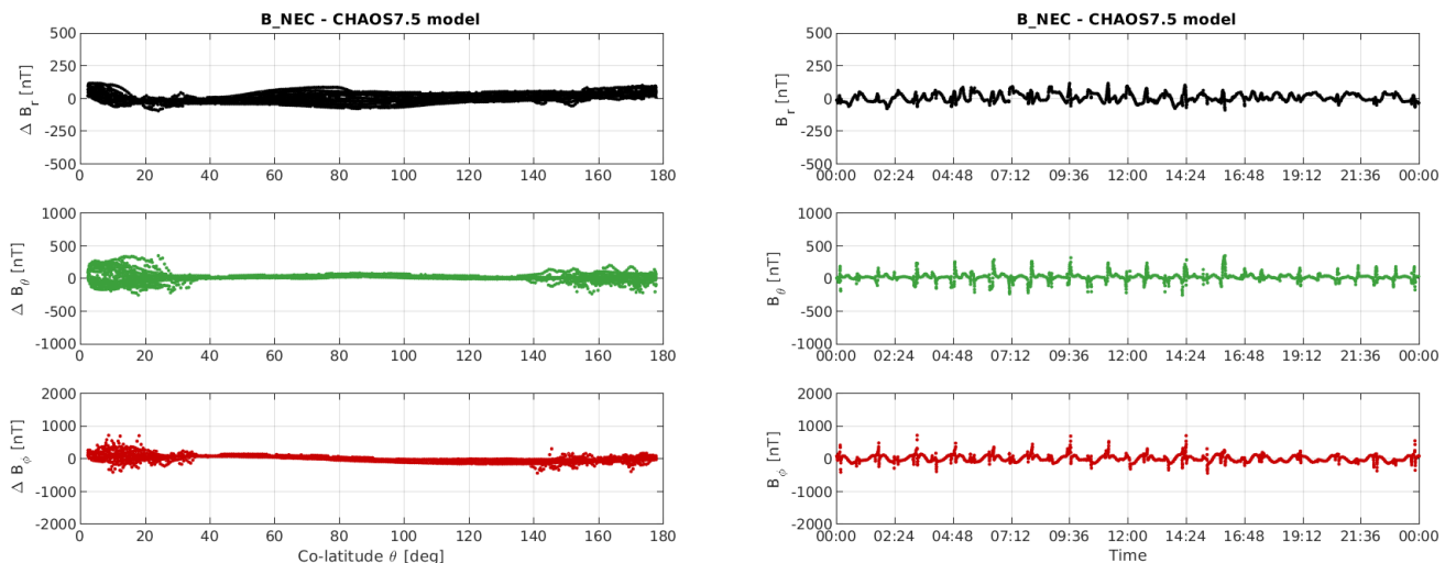
Figure 3-11: S/C B day 31/07: time series of B_{NEC} - B_{Chaos} residuals (right) and B_{NEC} - B_{Chaos} vs colatitude (left).
