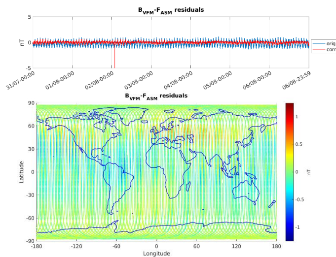
Figure 3-5: ASM-VFM residuals for S/C A, during monitoring period 31/07-06/08. In top figure are plotted: difference between |B_{VFM}| and F_{ASM} (without dB_{Sun} correction) (blue colour), and the residuals with dB_{Sun} corrections (red colour). In bottom figure residuals are presented on the world map.
