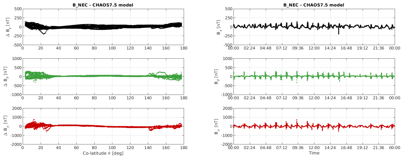
Figure 3-10: S/C A day 31/07: time series of B_{NEC} - B_{Chaos} residuals (right) and B_{NEC} - B_{Chaos} vs colatitude (left).
