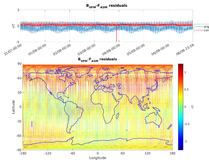
Figure 3-6: ASM-VFM residuals for S/C B, during monitoring period 31/07-06/08. In top figure are plotted: difference between |B_{VFM}| and F_{ASM} (without dB Sun correction) (blue colour), and the residuals with dB Sun corrections (red colour). In bottom figure residuals are presented on the world map.
