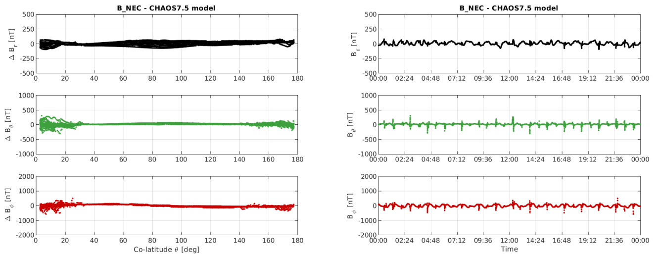
Figure 3-10: S/C A day 24/07: time series of B_{NEC} - B_{Chaos} residuals (right) and B_{NEC} - B_{Chaos} vs colatitude (left).
