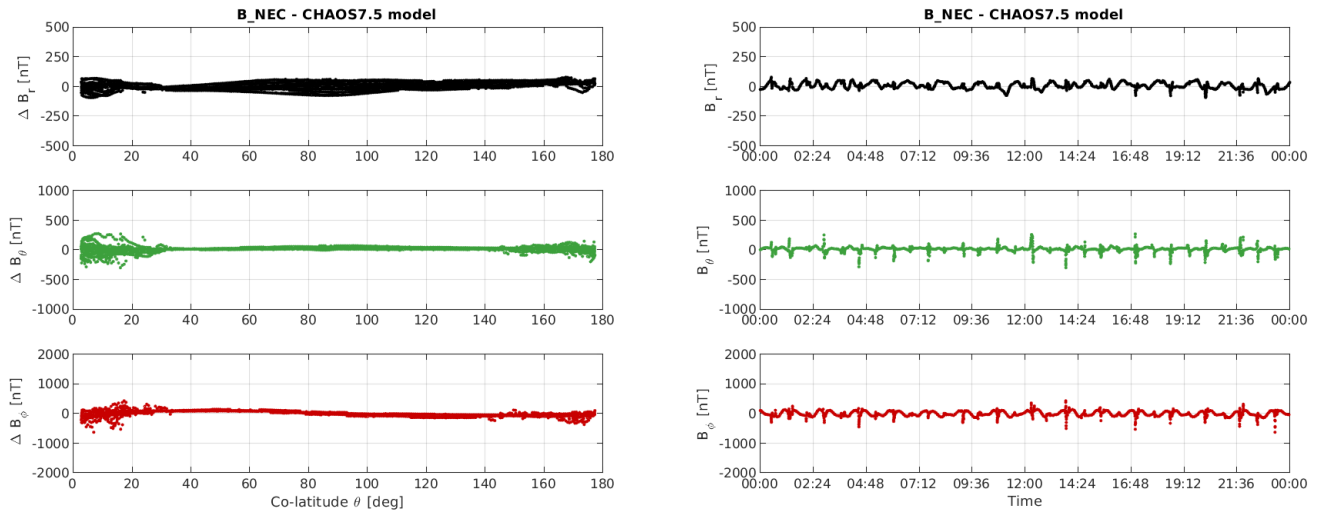
Figure 3-12: S/C C day 24/07: time series of B_{NEC} - B_{Chaos} residuals (right) and B_{NEC} - B_{Chaos} vs colatitude (left)
