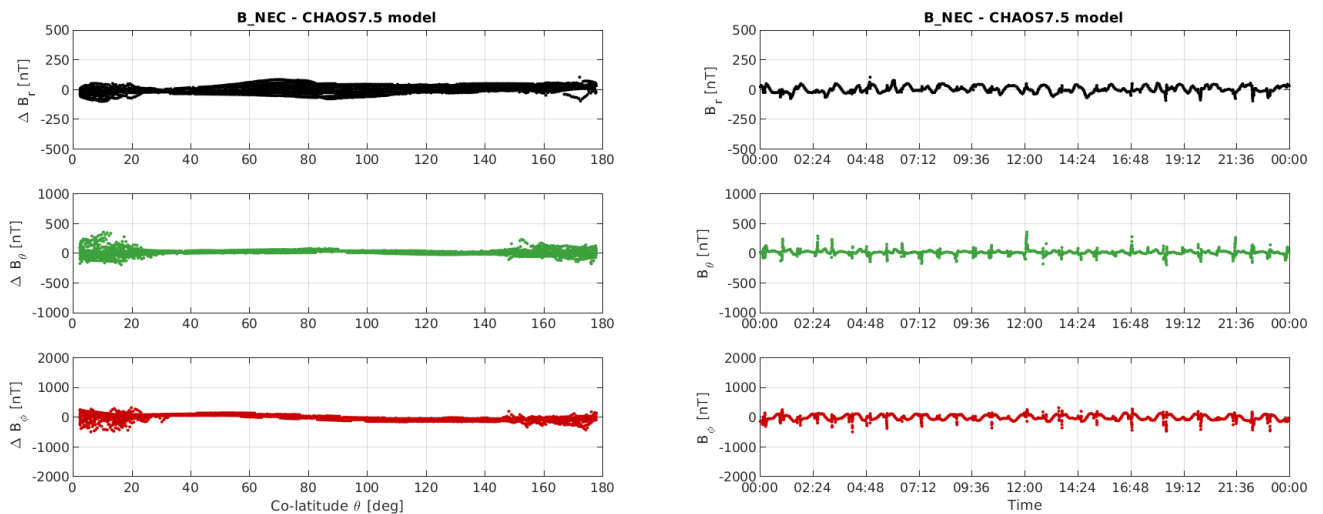
Figure 3-11: S/C B day 24/07: time series of B_{NEC} - B_{Chaos} residuals (right) and B_{NEC} - B_{Chaos} vs colatitude (left).
