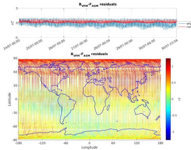
Figure 3-6: ASM-VFM residuals for S/C B, during monitoring period 24/07-30/07. In top figure are plotted: difference between |B_{VFM}| and F_{ASM} (without dB_{Sun} correction) (blue colour), and the residuals with dB_{Sun} corrections (red colour). In bottom figure residuals are presented on the world map.
