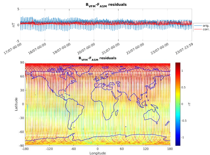
Figure 3-6: ASM-VFM residuals for S/C B, during monitoring period 17/07-23/07. In top figure are plotted: difference between |B_{VFM}| and F_{ASM} (without dB_Sun correction) (blue colour), and the residuals with dB_Sun corrections (red colour). In bottom figure residuals are presented on the world map.
