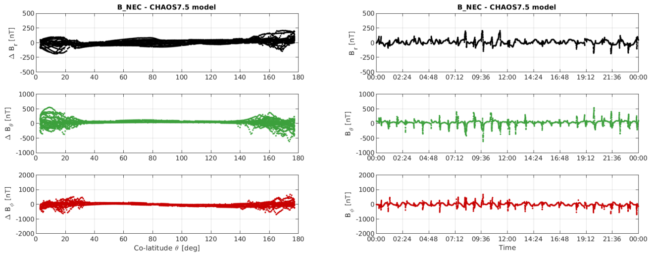
Figure 3-12: S/C C day 17/07: time series of B_{NEC} - B_{Chaos} residuals (right) and B_{NEC} - B_{Chaos} vs colatitude (left)
