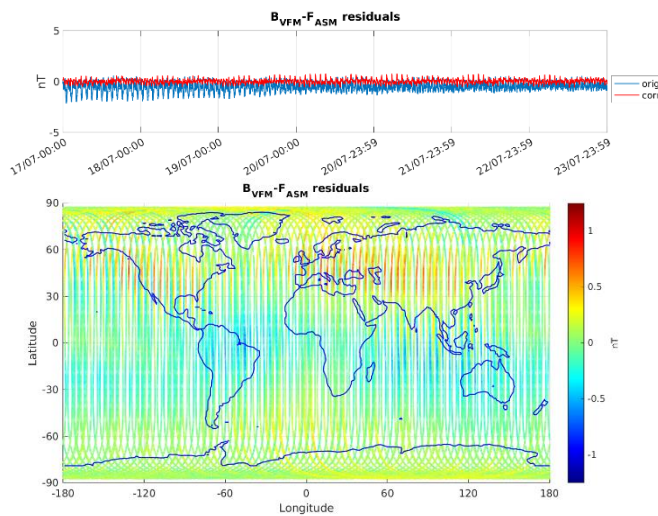
Figure 3-5: ASM-VFM residuals for S/C A, during monitoring period 17/07-23/07. In top figure are plotted: difference between |B_{VFM}| and F_{ASM} (without dB_{Sun} correction) (blue colour), and the residuals with dB_{Sun} corrections (red colour). In bottom figure residuals are presented on the world map.
