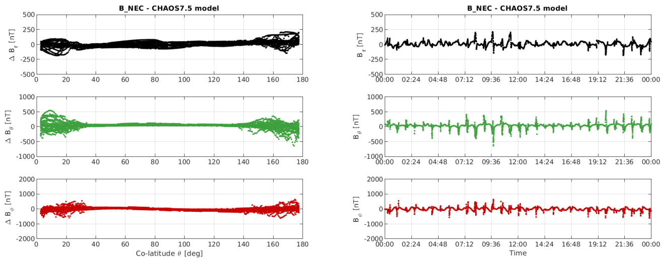
Figure 3-10: S/C A day 17/07: time series of B_{NEC} - B_{Chaos} residuals (right) and B_{NEC} - B_{Chaos} vs colatitude (left).
