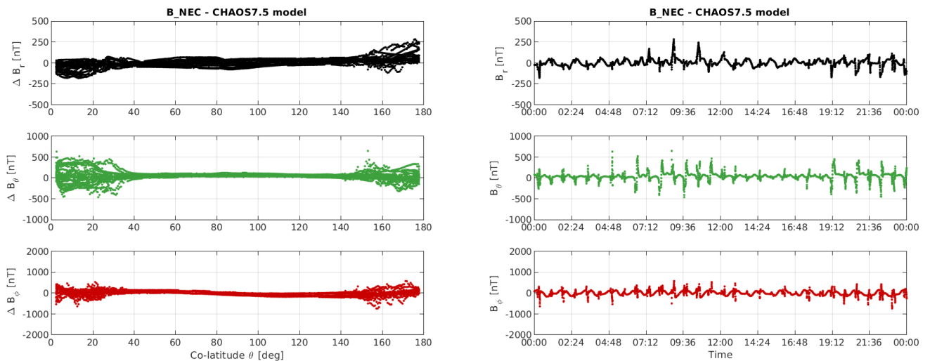
Figure 3-11: S/C B day 17/07: time series of B_{NEC} - B_{Chaos} residuals (right) and B_{NEC} - B_{Chaos} vs colatitude (left).
