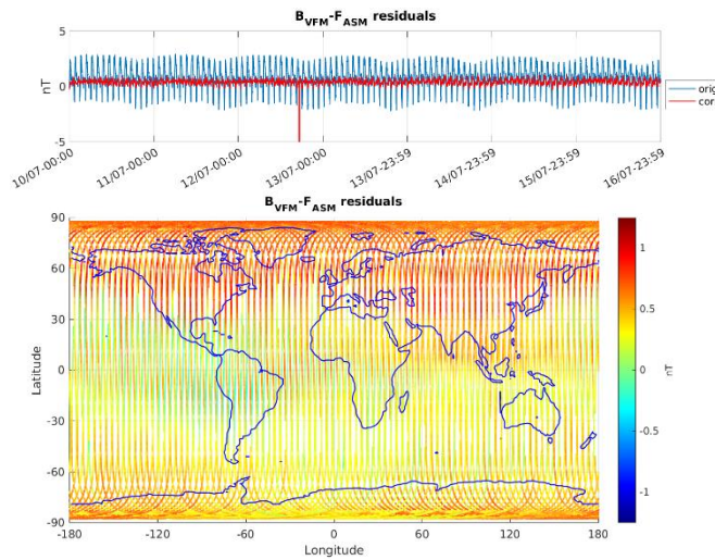
Figure 3-6: ASM-VFM residuals for S/C B, during monitoring period 10/07-16/07. In top figure are plotted: difference between |B_{VFM}| and F_{ASM} (without dB_{Sun} correction) (blue colour), and the residuals with dB_{Sun} corrections (red colour). In bottom figure residuals are presented on the world map. Outlier from 12/07/2023 is coming from the data gap registered on all instruments of SWARM-B.
