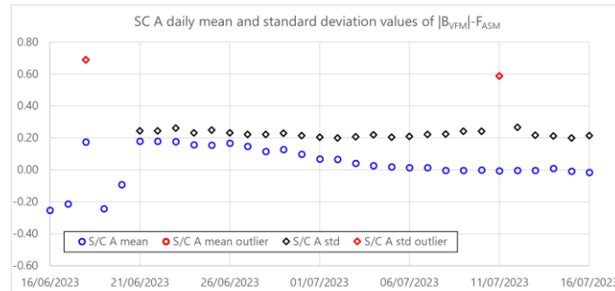
Figure 3-3: Daily mean and standard deviation values of ASM-VFM residuals (defined as dF = |B_{VFM}| - F_{ASM} ) for S/C A. Outlier from 11/07/2023 is coming from the manoeuvre of SWARM-A.
