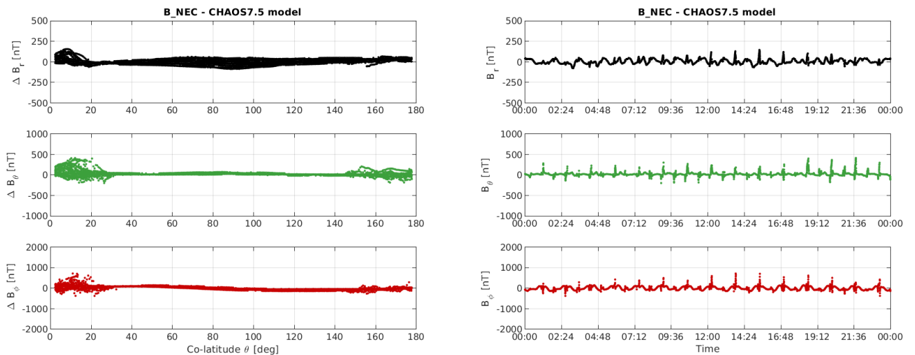
Figure 3-11: S/C B day 10/07: time series of B_{NEC} - B_{Chaos} residuals (right) and B_{NEC} - B_{Chaos} vs colatitude (left).
