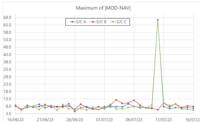
Figure 3-2: Plot of the maximum difference of the absolute value of the difference between MOD and NAV solutions for all satellites. Plot covers last month of operation. Outliers in SWARM-A and -C on 10/07/2023 are due to L0 GPSANAV and GPSCNAV peaks registered in quality index and dilution of precision characteristics.
