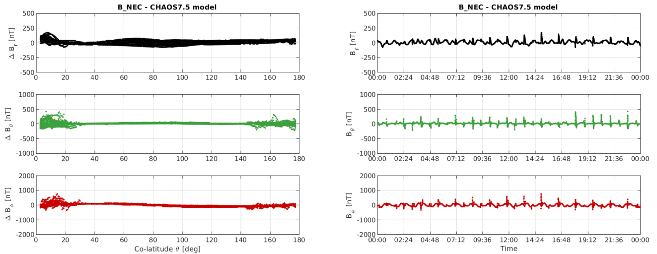
Figure 3-12: S/C C day 10/07: time series of B_{NEC} - B_{Chaos} residuals (right) and B_{NEC} - B_{Chaos} vs colatitude (left)
