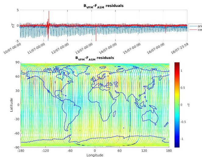
Figure 3-5: ASM-VFM residuals for S/C A, during monitoring period 10/07-16/07. In top figure are plotted: difference between |B_{VFM}| and F_{ASM} (without dB_{Sun} correction) (blue colour), and the residuals with dB_{Sun} corrections (red colour). In bottom figure residuals are presented on the world map. Outlier from 11/07/2023 is coming from the manoeuvre of SWARM-A.
