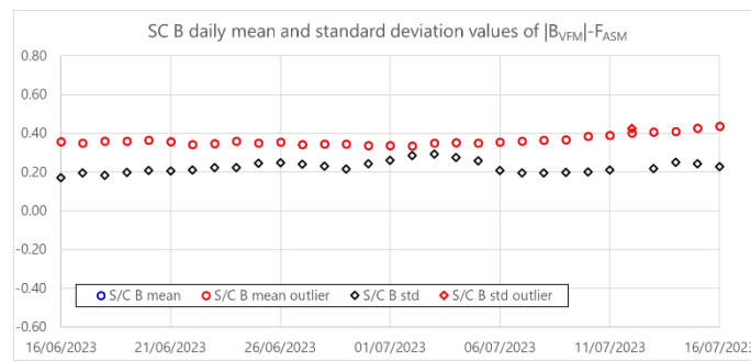
Figure 3-4: Daily mean and standard deviation values of ASM-VFM residuals (defined as dF = |B_{VFM}| - F_{ASM} ) for S/C B. Outlier from 12/07/2023 is coming from the data gap registered on all instruments of SWARM-B.
