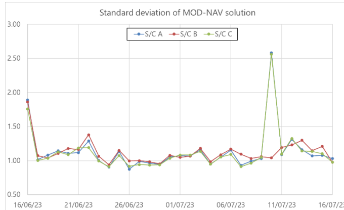
Figure 3-1: Plot of the standard deviation of the difference between MOD and NAV solutions for all satellites. Plot covers last month of operation. Outliers in SWARM-A and -C on 10/07/2023 are due to L0 GPSANAV and GPSCNAV peaks registered in quality index and dilution of precision characteristics.
