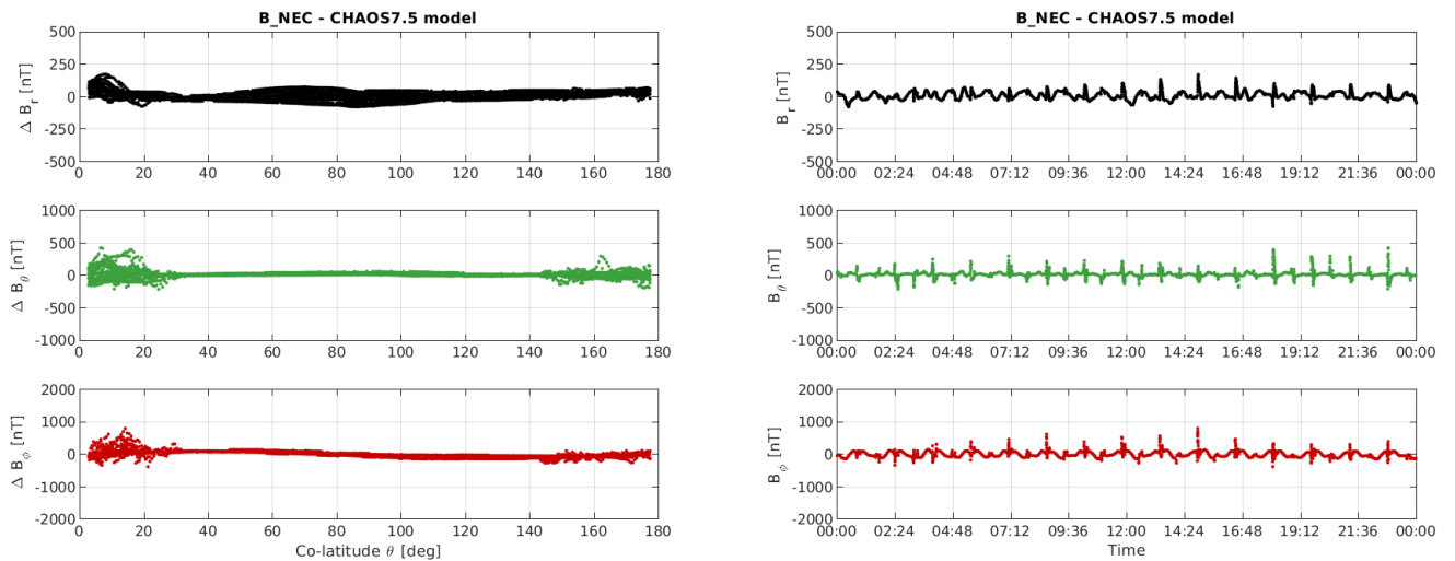
Figure 3-10: S/C A day 10/07: time series of B_{NEC} - B_{Chaos} residuals (right) and B_{NEC} - B_{Chaos} vs colatitude (left).
