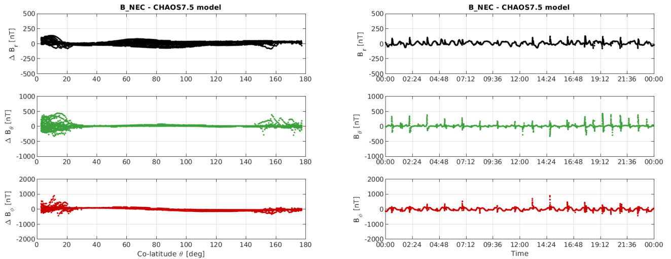
Figure 3-12: S/C C day 03/07: time series of B_{NEC} - B_{Chaos} residuals (right) and B_{NEC} - B_{Chaos} vs colatitude (left)
