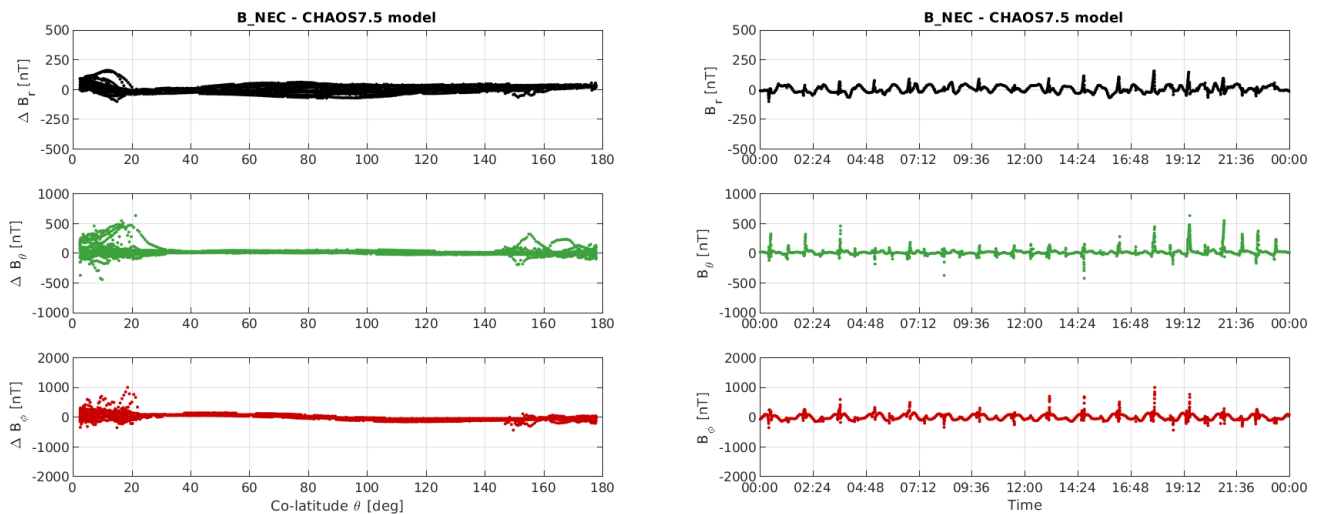
Figure 3-11: S/C B day 03/07: time series of B_{NEC} - B_{Chaos} residuals (right) and B_{NEC} - B_{Chaos} vs colatitude (left).
