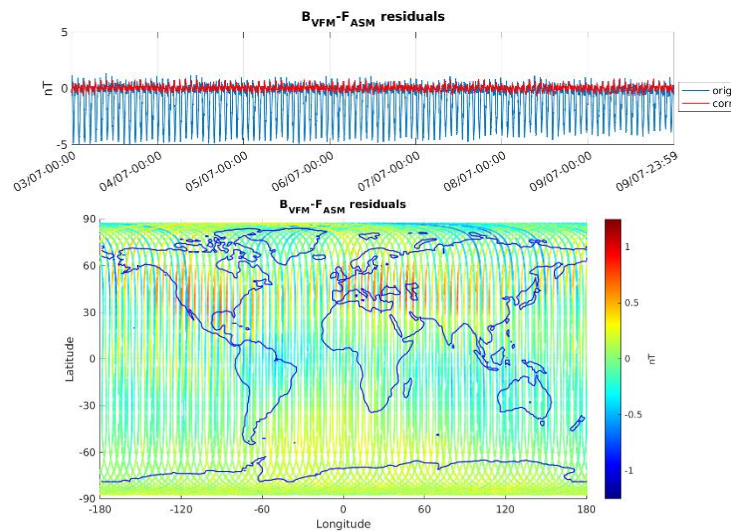
Figure 3-5: ASM-VFM residuals for S/C A, during monitoring period 03/07-09/07. In top figure are plotted: difference between |B_{VFM}| and F_{ASM} (without dB_{Sun} correction) (blue colour), and the residuals with dB_{Sun} corrections (red colour). In bottom figure residuals are presented on the world map.
