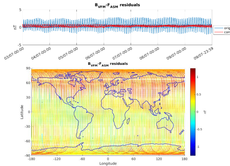
Figure 3-6: ASM-VFM residuals for S/C B, during monitoring period 03/07-09/07. In top figure are plotted: difference between |B_{VFM}| and F_{ASM} (without dB_{Sun} correction) (blue colour), and the residuals with dB_{Sun} corrections (red colour). In bottom figure residuals are presented on the world map.
