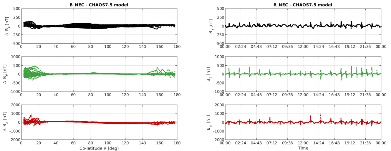
Figure 3-10: S/C A day 03/07: time series of B_{NEC} - B_{Chaos} residuals (right) and B_{NEC} - B_{Chaos} vs colatitude (left).
