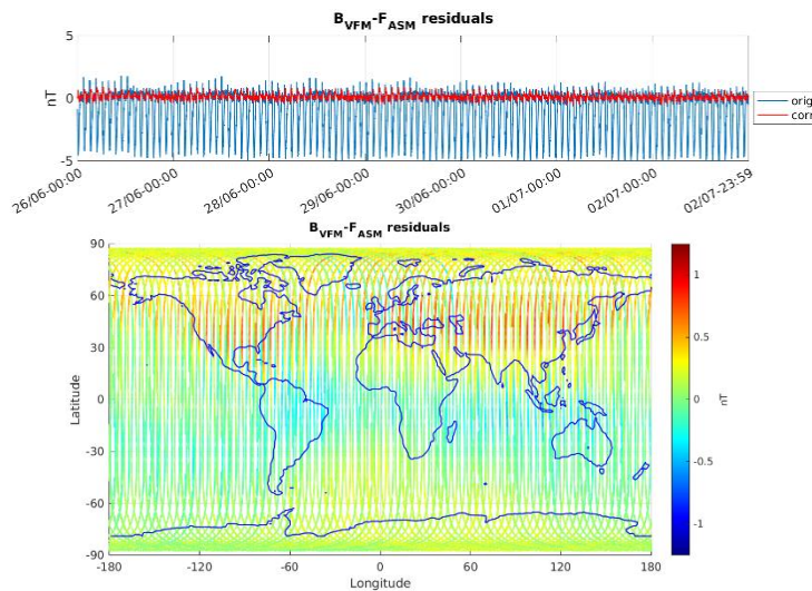
Figure 3-5: ASM-VFM residuals for S/C A, during monitoring period 26/06-02/07. In top figure are plotted: difference between |B_{VFM}| and F_{ASM} (without dB_{Sun} correction) (blue colour), and the residuals with dB_{Sun} corrections (red colour). In bottom figure residuals are presented on the world map.
