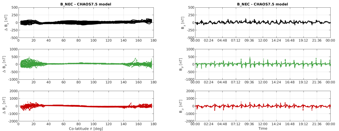
Figure 3-10: S/C A day 26/06: time series of B_{NEC} - B_{Chaos} residuals (right) and B_{NEC} - B_{Chaos} vs colatitude (left).
