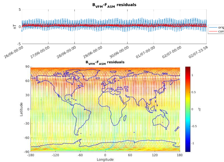
Figure 3-6: ASM-VFM residuals for S/C B, during monitoring period 26/06-02/07. In top figure are plotted: difference between |B_{VFM}| and F_{ASM} (without dB_{Sun} correction) (blue colour), and the residuals with dB_{Sun} corrections (red colour). In bottom figure residuals are presented on the world map.
