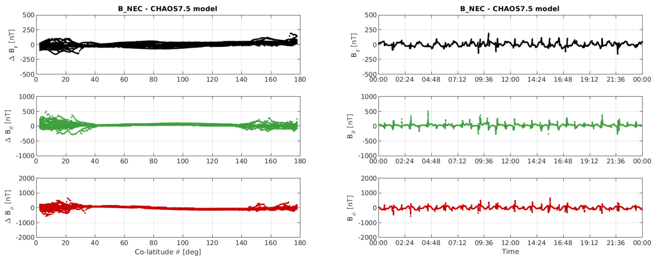
Figure 3-11: S/C B day 26/06: time series of B_{NEC} - B_{Chaos} residuals (right) and B_{NEC} - B_{Chaos} vs colatitude (left).
