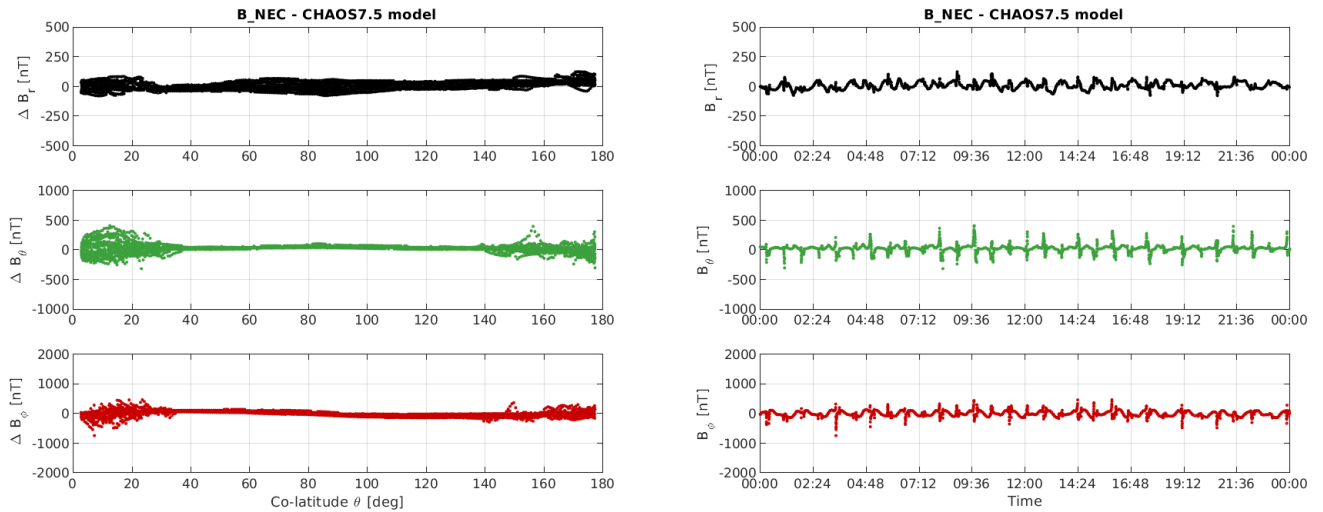
Figure 3-12: S/C C day 26/06: time series of B_{NEC} - B_{Chaos} residuals (right) and B_{NEC} - B_{Chaos} vs colatitude (left)
