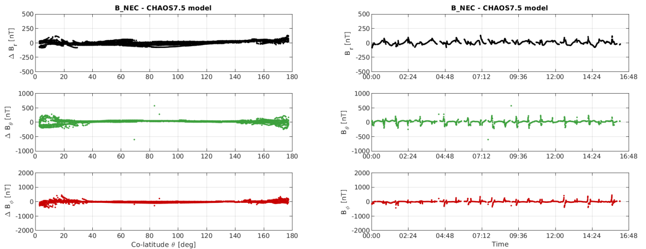
Figure 3-10: S/C A day 19/06: time series of B_{NEC} - B_{Chaos} residuals (right) and B_{NEC} - B_{Chaos} vs colatitude (left).
