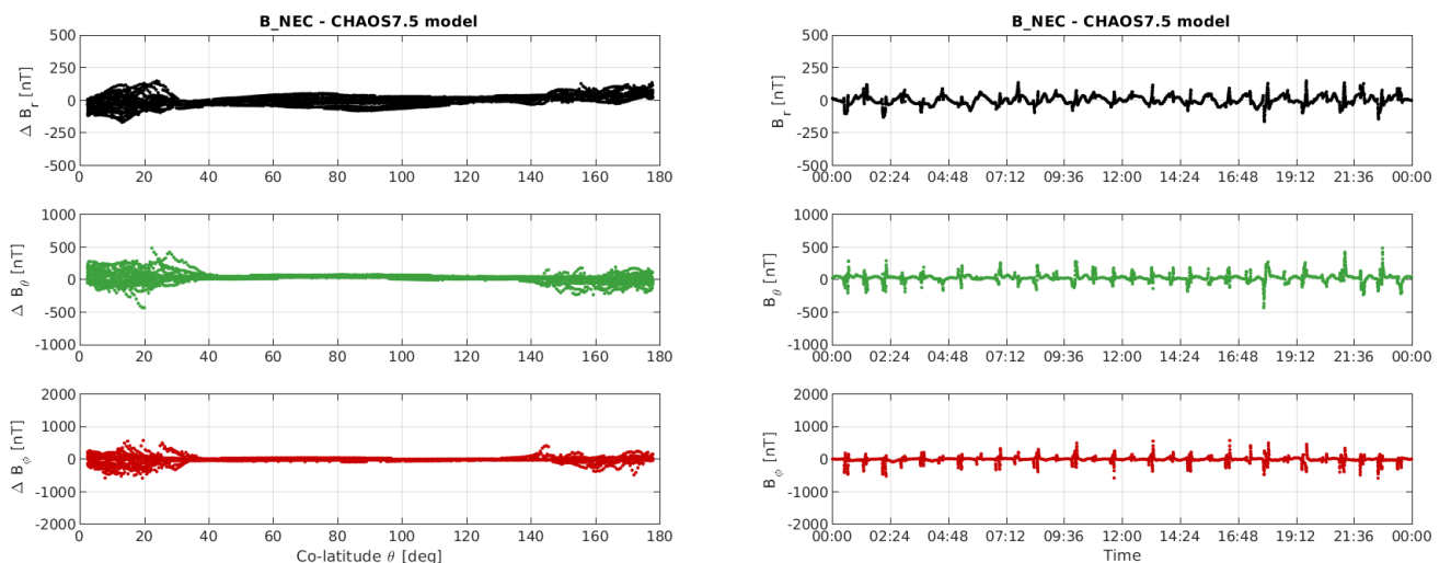
Figure 3-11: S/C B day 19/06: time series of B_{NEC} - B_{Chaos} residuals (right) and B_{NEC} - B_{Chaos} vs colatitude (left).
