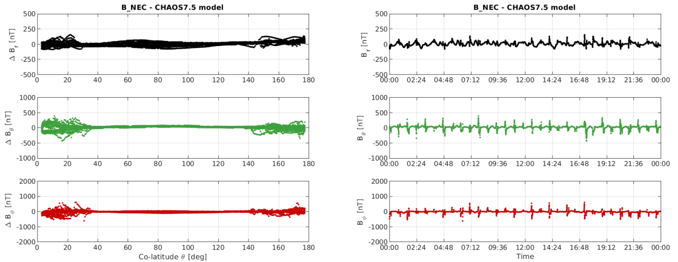
Figure 3-12: S/C C day 19/06: time series of B_{NEC} - B_{Chaos} residuals (right) and B_{NEC} - B_{Chaos} vs colatitude (left)
