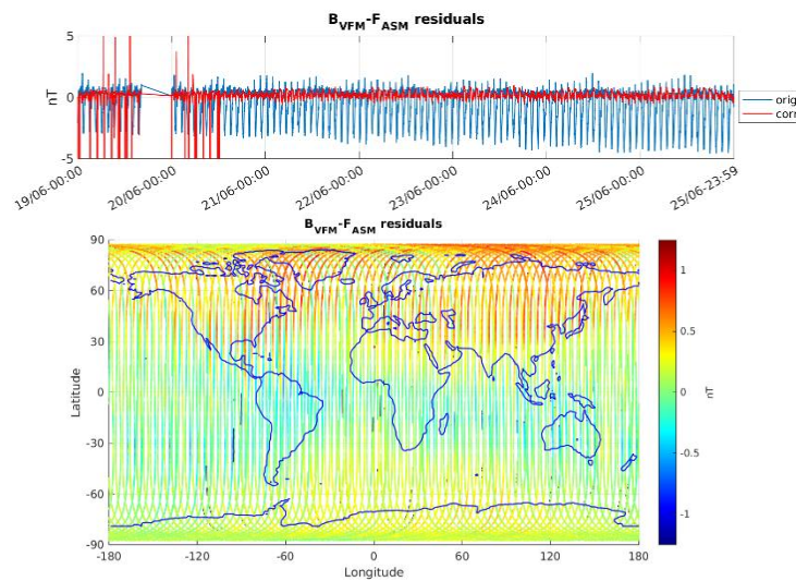
Figure 3-5: ASM-VFM residuals for S/C A, during monitoring period 19/06-25/06. In top figure are plotted: difference between |B_{VFM}| and F_{ASM} (without dB_{Sun} correction) (blue colour), and the residuals with dB_{Sun} corrections (red colour). In bottom figure residuals are presented on the world map.
