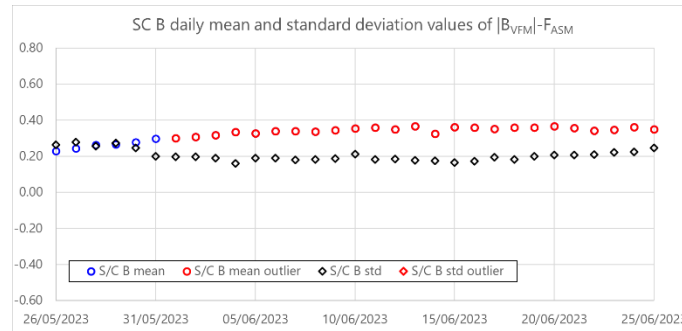
Figure 3-4: Daily mean and standard deviation values of ASM-VFM residuals (defined as dF = |B_{VFM}| - F_{ASM} ) for S/C B.
