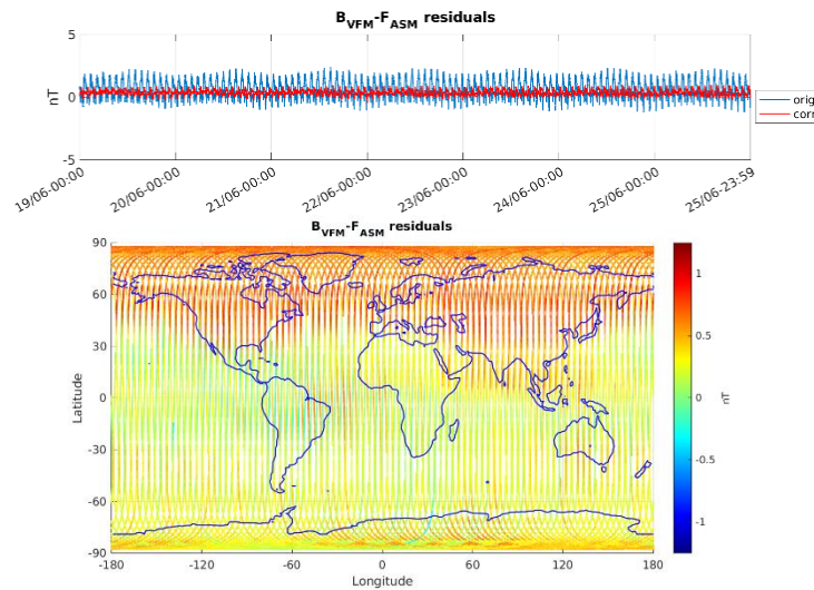
Figure 3-6: ASM-VFM residuals for S/C B, during monitoring period 19/06-25/06. In top figure are plotted: difference between |B_{VFM}| and F_{ASM} (without dB_{Sun} correction) (blue colour), and the residuals with dB_{Sun} corrections (red colour). In bottom figure residuals are presented on the world map.
