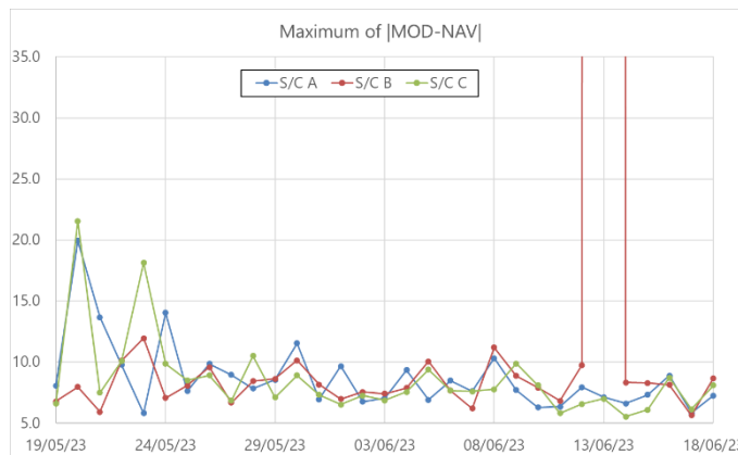
Figure 3-2: Plot of the maximum difference of the absolute value of the difference between MOD and NAV solutions for all satellites. Plot covers last month of operation. was caused by manual restart of ASM burst mode session due to spontaneous GPS reboot.
