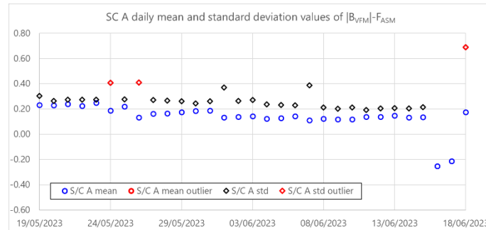
Figure 3-3: Daily mean and standard deviation values of ASM-VFM residuals (defined as dF=|B_{VFM}|-F_{ASM} ) for S/C A. Outliers presented from 16-18/06 are caused due to VFM L0 uncompressed data missing.
