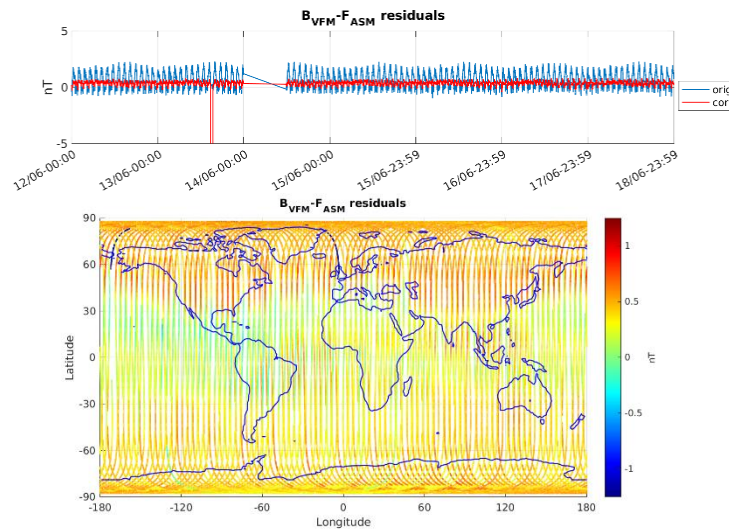
Figure 3-6: ASM-VFM residuals for S/C B, during monitoring period 12/06-18/06. In top figure are plotted: difference between |B_{VFM}| and F_{ASM} (without dB_{Sun} correction) (blue colour), and the residuals with dB_{Sun} corrections (red colour). In bottom figure residuals are presented on the world map. Data gap in MAGB\_CA\_1B registered on 14/06 from 00:00:00 to 11:49:15 was caused by manual restart of ASM burst mode session due to spontaneous GPS reboot.
