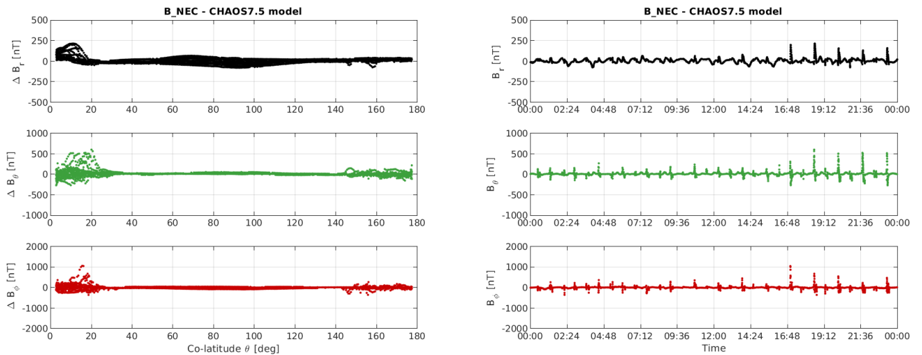
Figure 3-10: S/C A day 12/06: time series of B_{NEC} - B_{Chaos} residuals (right) and B_{NEC} - B_{Chaos} vs colatitude (left).
