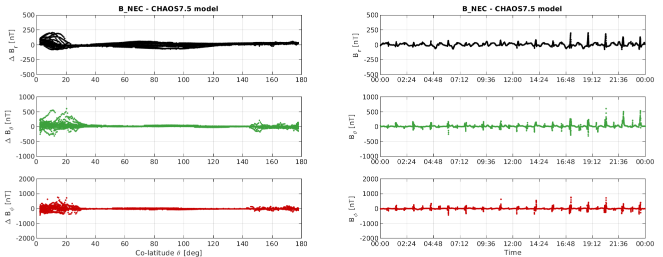
Figure 3-11: S/C B day 12/06: time series of B_{NEC} - B_{Chaos} residuals (right) and B_{NEC} - B_{Chaos} vs colatitude (left).
