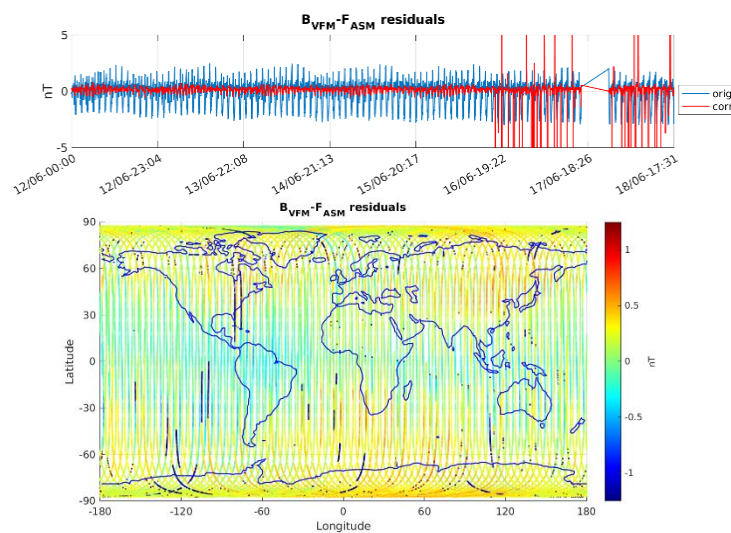
Figure 3-5: ASM-VFM residuals for S/C A, during monitoring period 12/06-18/06. In top figure are plotted: difference between |B_{VFM}| and F_{ASM} (without dB_{Sun} correction) (blue colour), and the residuals with dB_{Sun} corrections (red colour). In bottom figure residuals are presented on the world map. Data gaps in MAGA_CA_1B registered on 17/06 from 16:42:47 to 23:59:59 and on 18/06 from 17:31:04 to 23:59:59 were caused due to VFM L0 uncompressed data missing.
