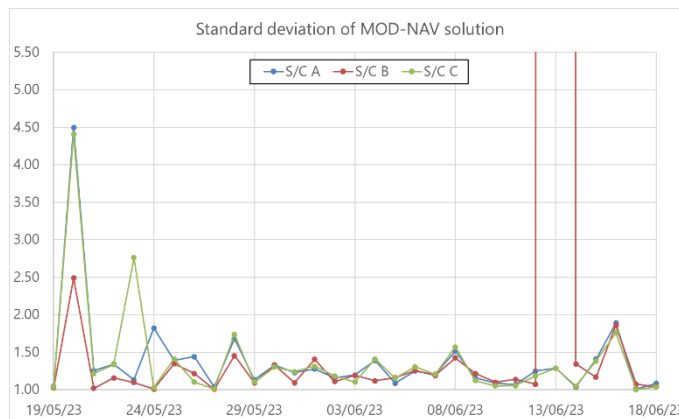
Figure 3-1: Plot of the standard deviation of the difference between MOD and NAV solutions for all satellites. Plot covers last month of operation. On 13/06 is registered outlier in Swarm-B characteristic due to spontaneous GPS reboot.
