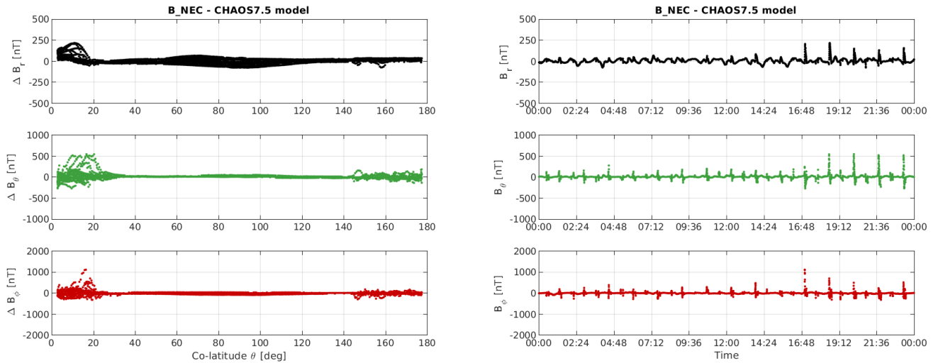
Figure 3-12: S/C C day 12/06: time series of B_{NEC} - B_{Chaos} residuals (right) and B_{NEC} - B_{Chaos} vs colatitude (left)
